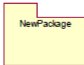
Gambar II.23. Notasi Package
