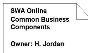
Gambar II.19. Notasi Note
