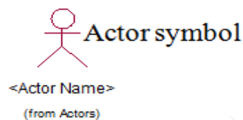
Gambar II.13. Notasi Actor
