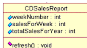
Gambar II.14. Notasi Class
