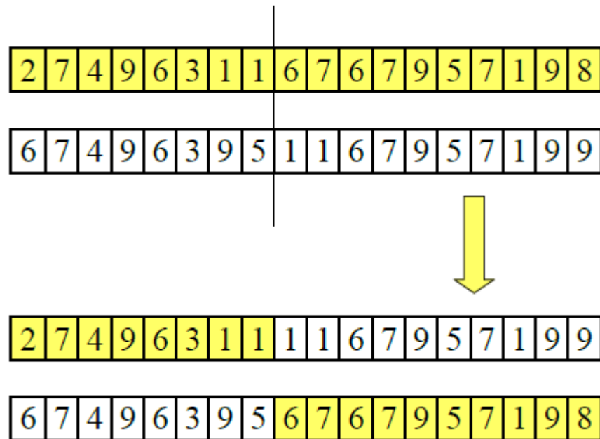
Gambar III.6. Crossover Single Point
