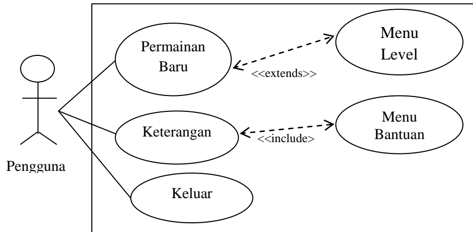
Gambar III.9. Use Case Diagram Aplikasi Game Sudoku
