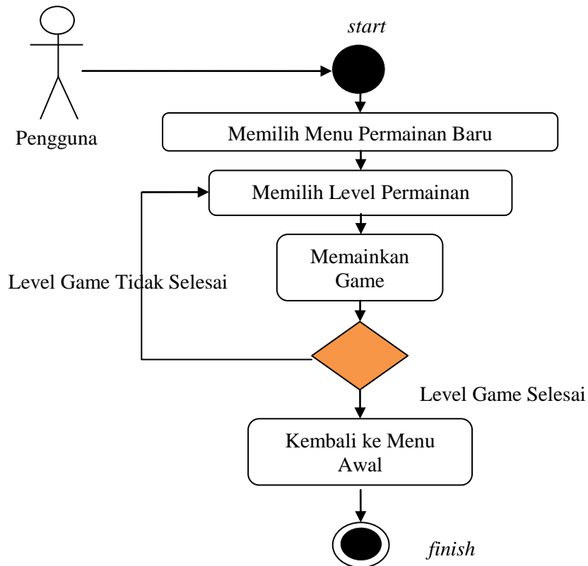
Gambar III.10. Activity Diagram Memainkan Game
