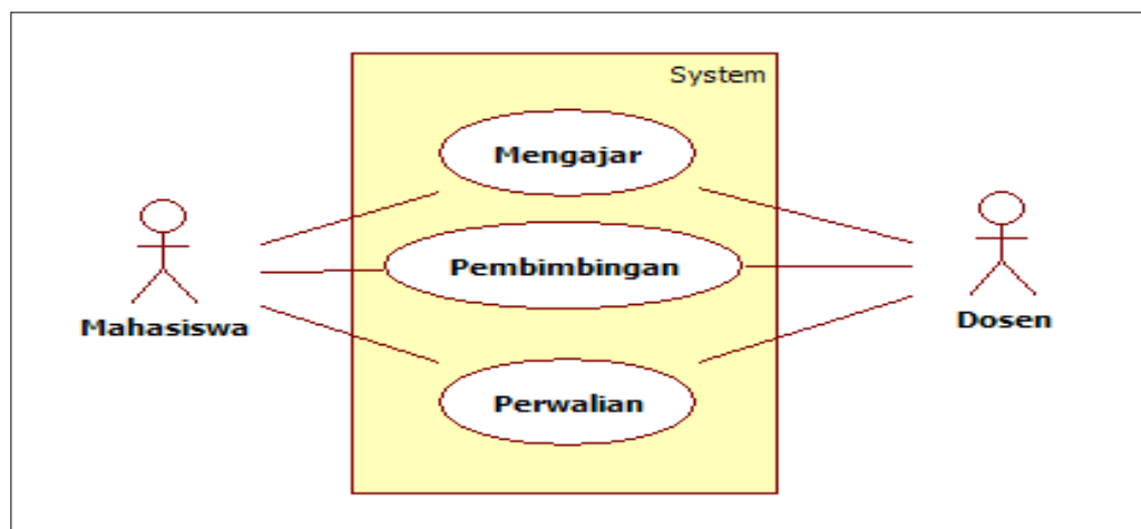
Gambar II.3. Contoh Use Case Diagram
