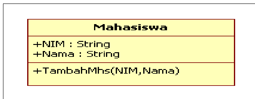
Gambar II.4. Contoh Class Diagram
