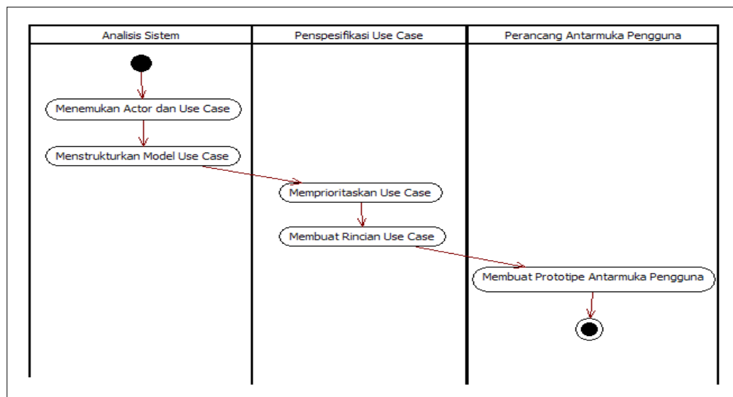
Gambar II.6. Contoh Activity Diagram
