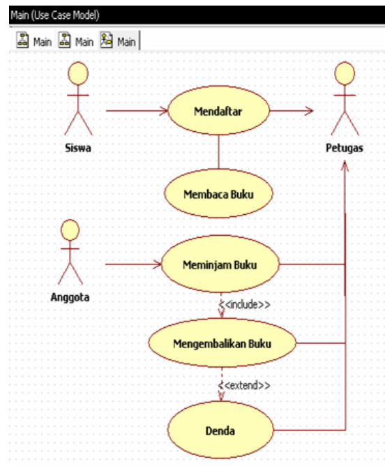
Gambar. II.7. Use Case Diagram
