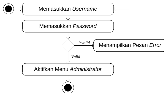
Gambar. II.6. Activity Diagram
