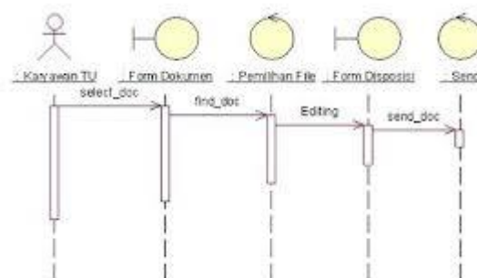
Gambar. II.4. Sequence Diagram
