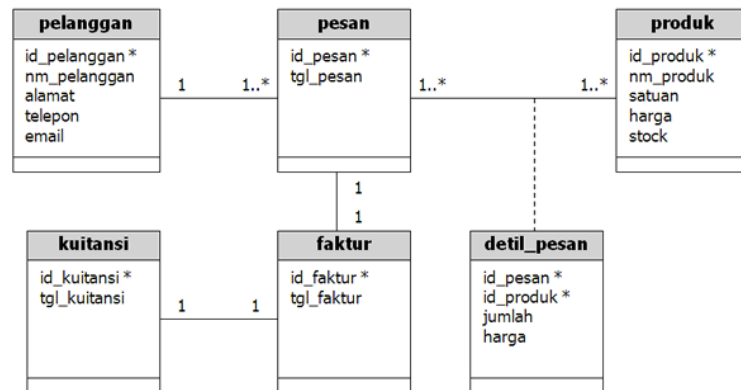
Gambar. II.5. Class Diagram
