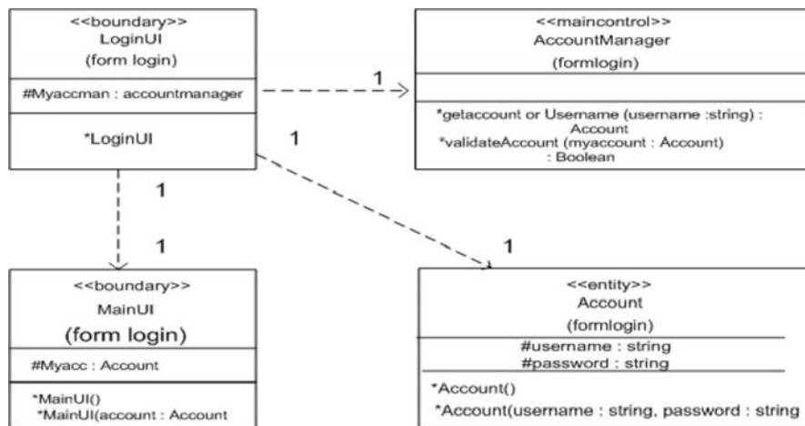
Gambar II.5. Notasi class diagram (Sumber : Haviluddin; 2011 : 3 )
