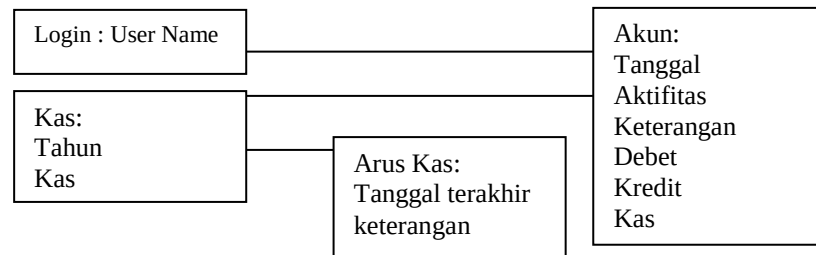
Gambar II.1. Class diagram Sumber : Prabowo Pudjo Widodo ; 2011 : 38
