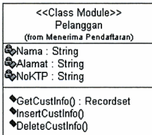
Gambar II.4. Notasi Class
