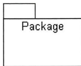
Gambar II.8. Notasi Package
