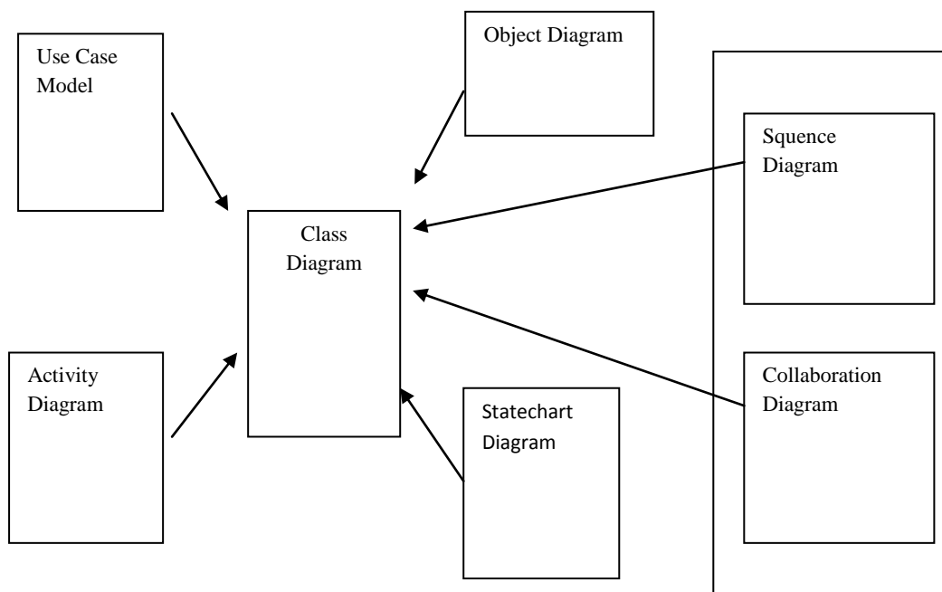
Gambar II.9. Class Diagram
