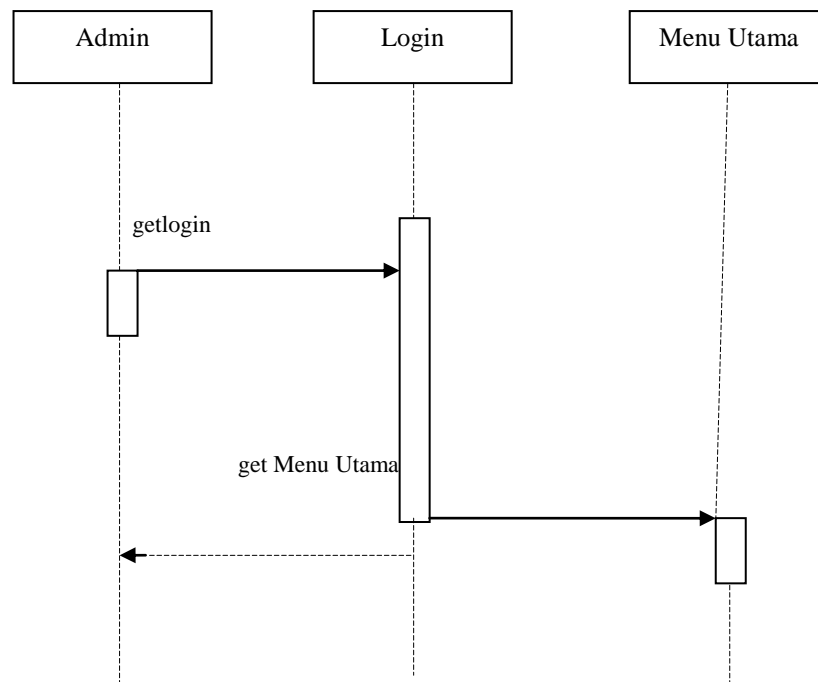
Gambar III.12 Sequence Diagram Urutan
