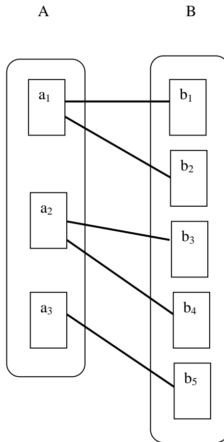
Gambar II.5. Hubungan one-to-many
