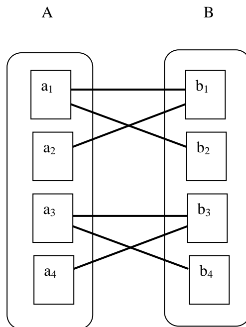
Gambar II.7. Hubungan many-to-many
