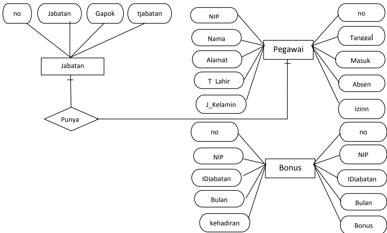
Gambar II.3. Entity Relationship Diagram
