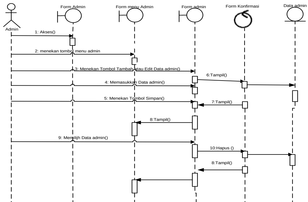
Gambar III.14 Sequence diagram proses input data Admin
