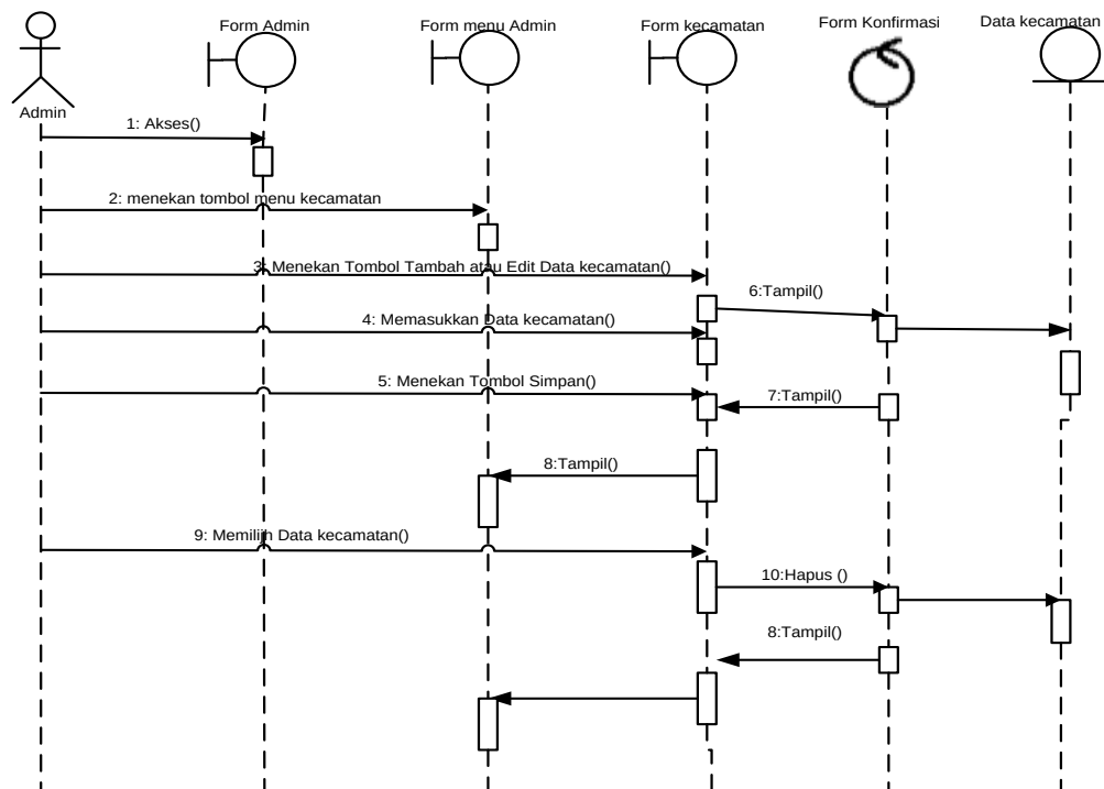
Gambar III.15 Sequence diagram proses input data kecamatan
