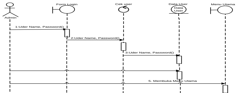
Gambar III.13 Sequence diagram Login Ke Sistem
