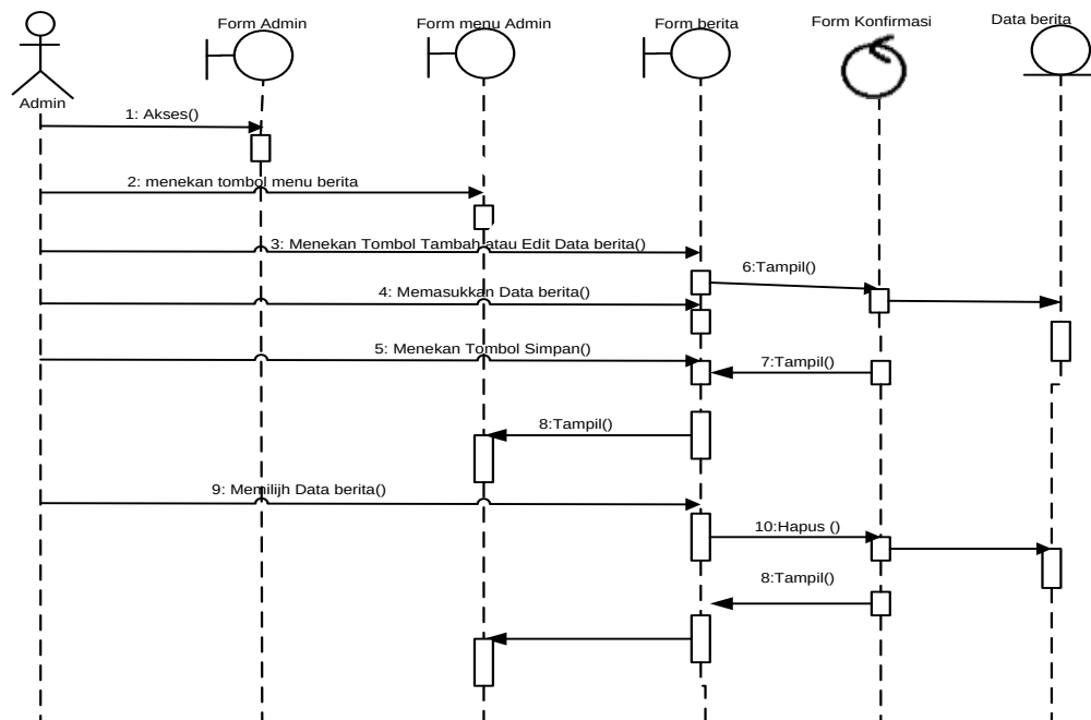
Gambar III.18 Sequence diagram proses input data berita dan kegiatan
