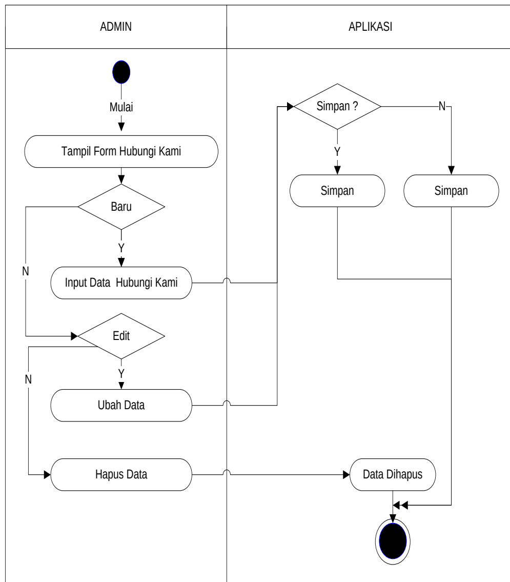
Gambar III.9. Diagram Activity Hubungi Kami
