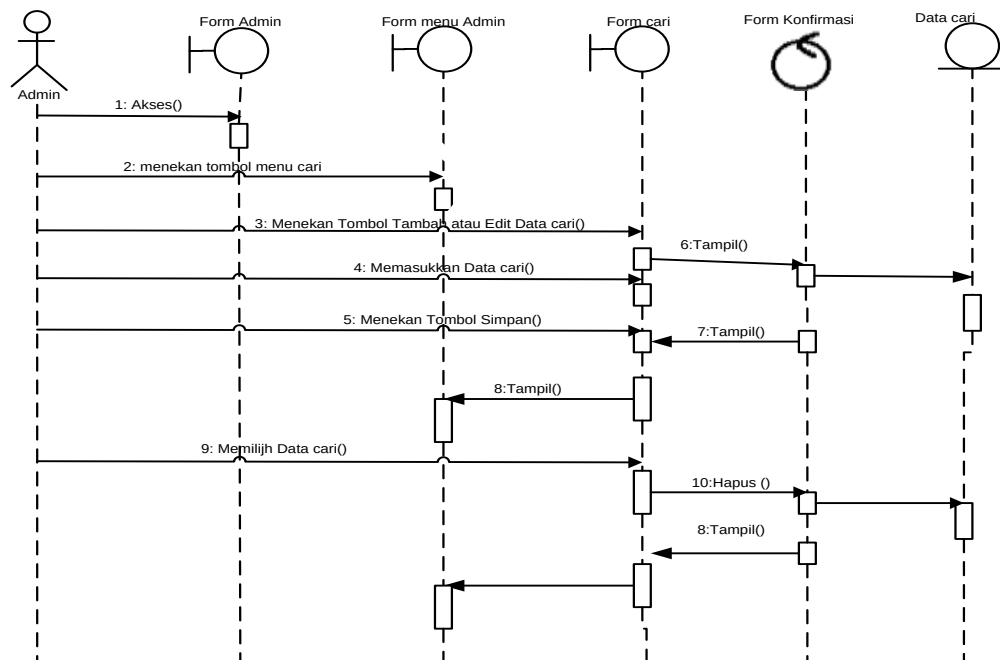
Gambar III.20 Sequence diagram proses Cari Karate Wadokai
