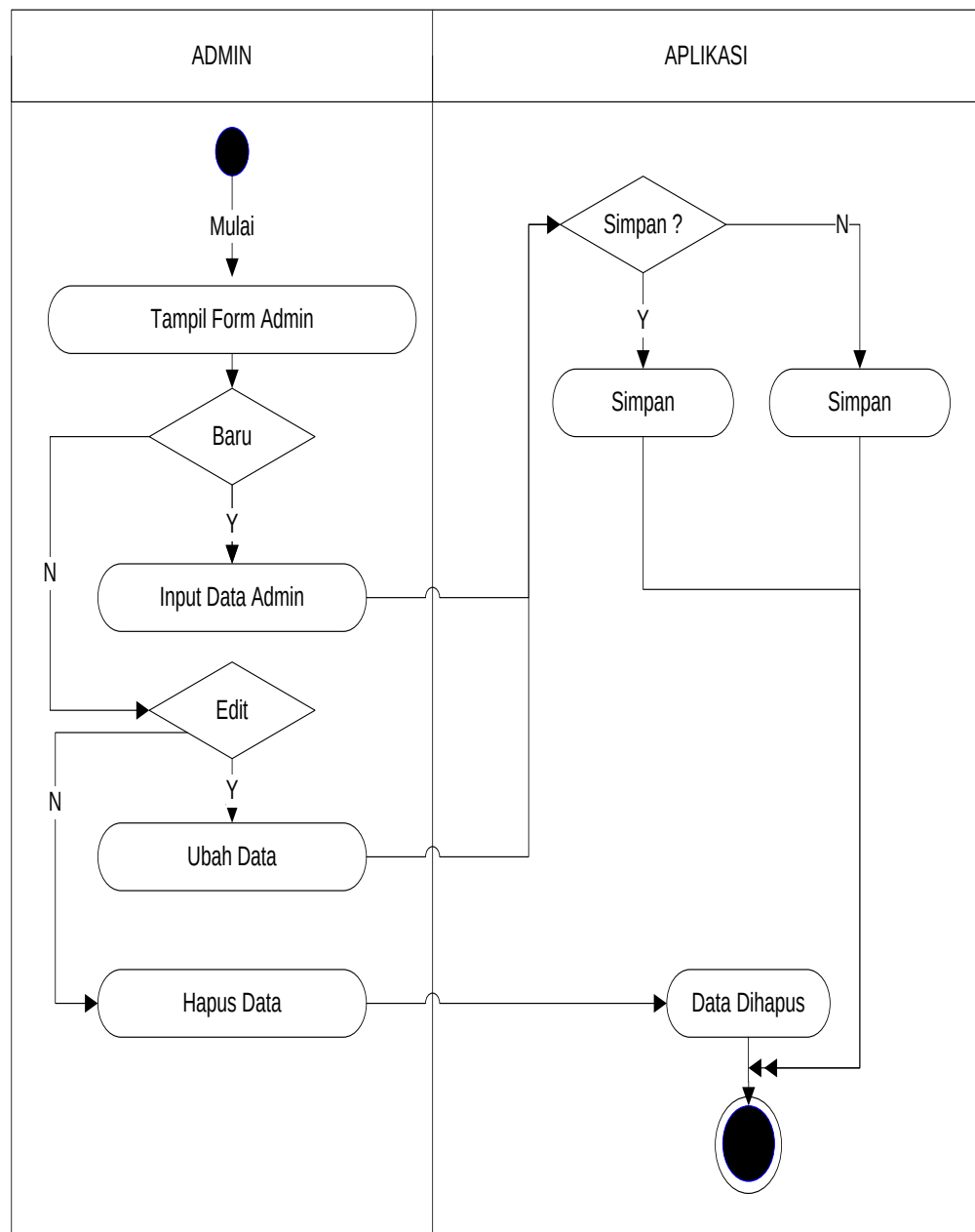
Gambar III.4. Diagram Activity Form Admin
