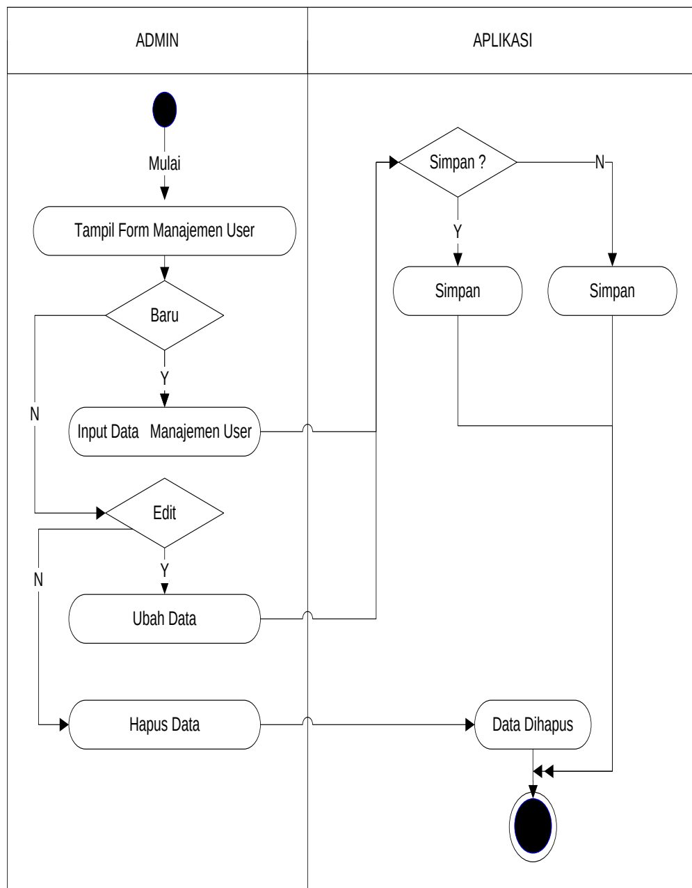
Gambar III.11. Diagram Activity Manajemen User
