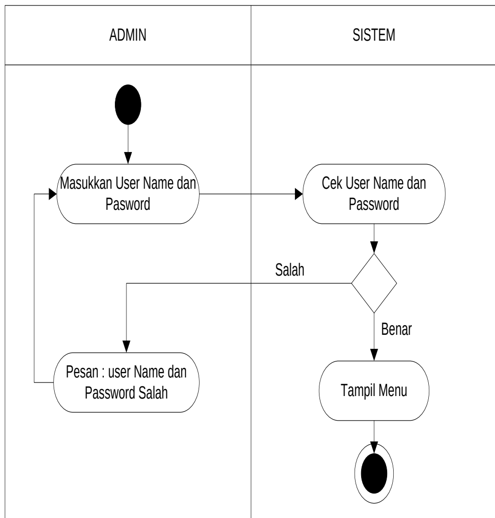
Gambar III.3. Diagram Activity Login
