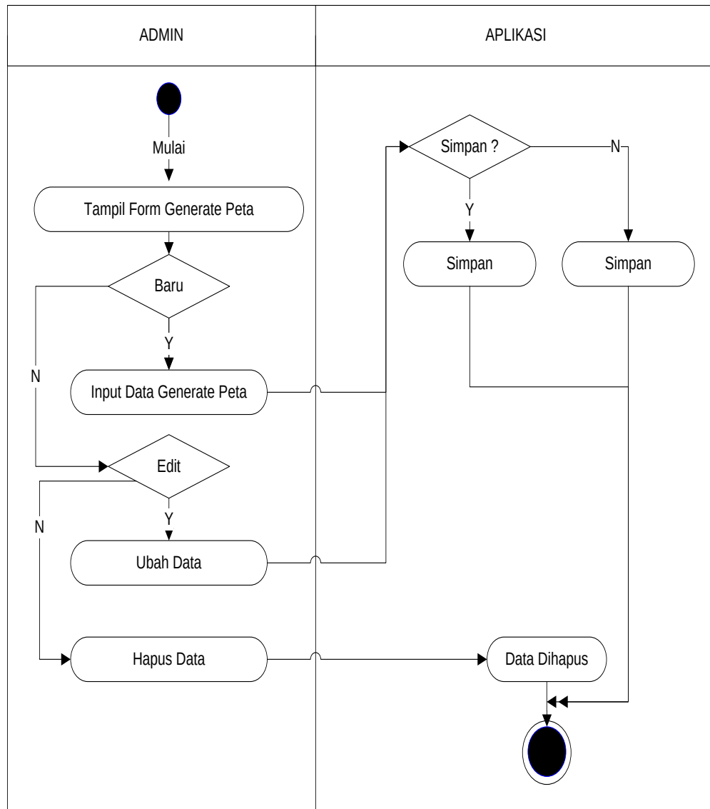
Gambar III.7. Diagram Activity Generate Peta
