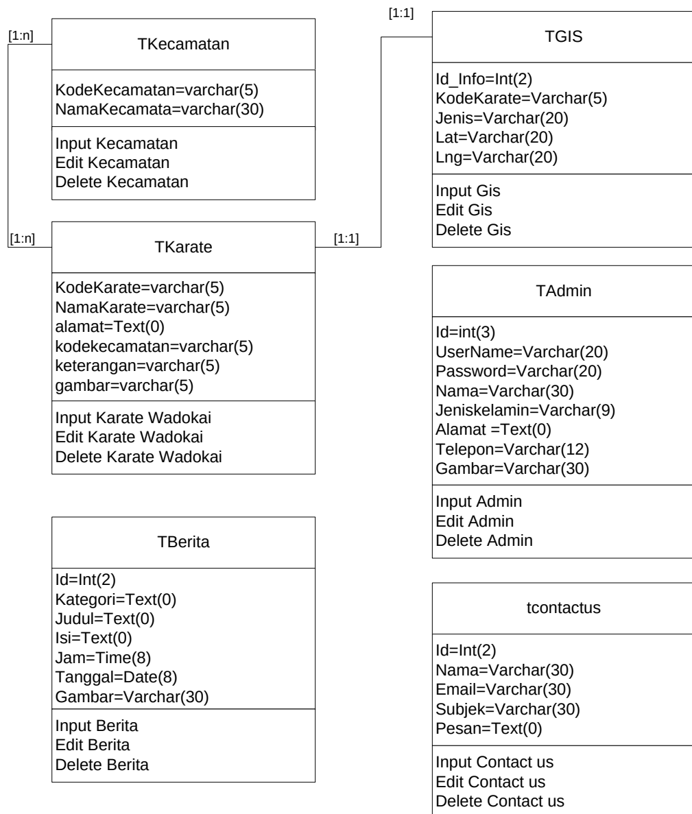
Gambar III.2 Class diagram Admin
