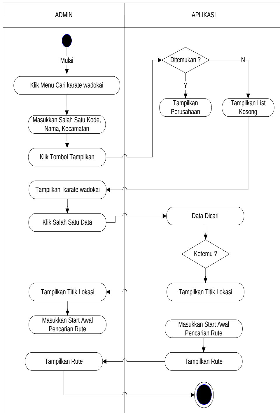
Gambar III.12. Diagram Activity Cari Karate Wadokai
