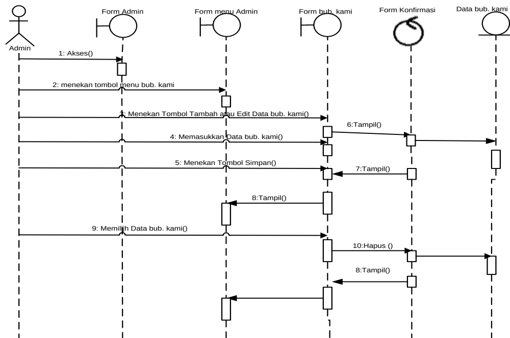
Gambar III.19 Sequence diagram proses input data Hubungi Kami
