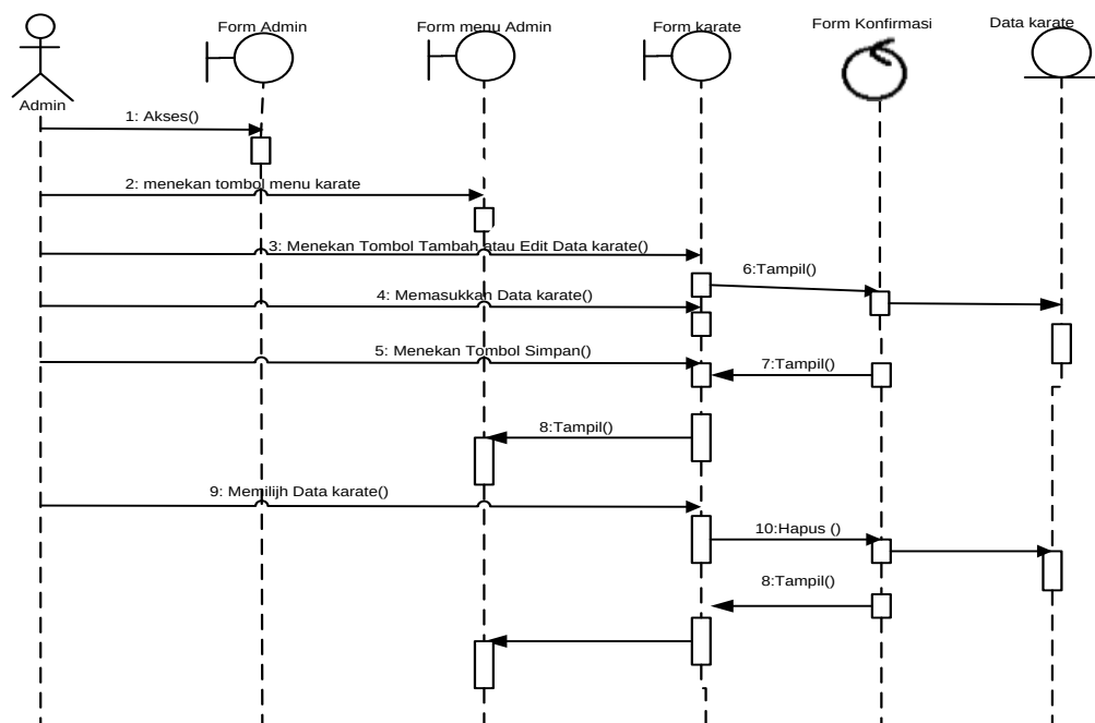
Gambar III.16 Sequence diagram proses input data Karate Wadokai
