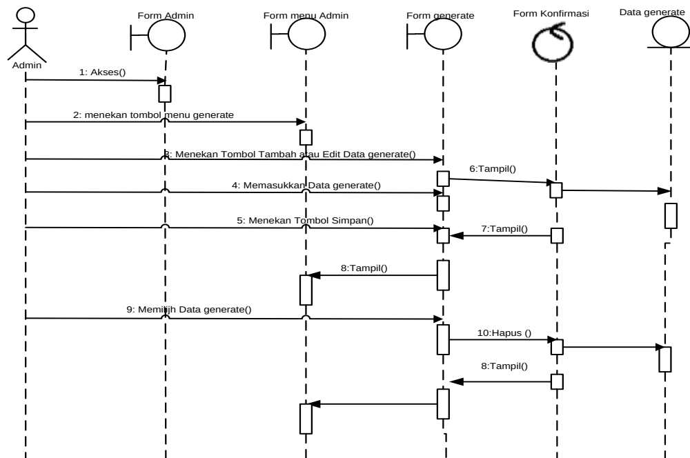
Gambar III.17 Sequence diagram proses input data generate peta
