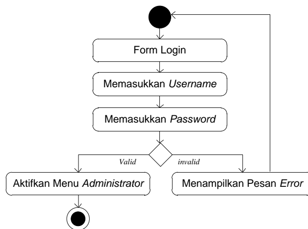
Gambar III.5. Activity Diagram Login
