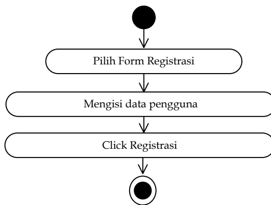
Gambar III.14. Activity Diagram Registrasi
