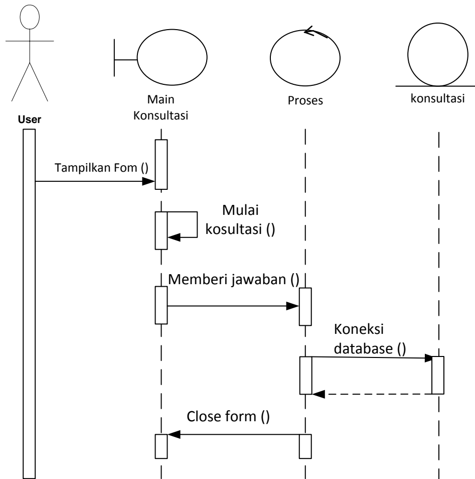
Gambar III.22. Sequence Diagram Konsultasi
