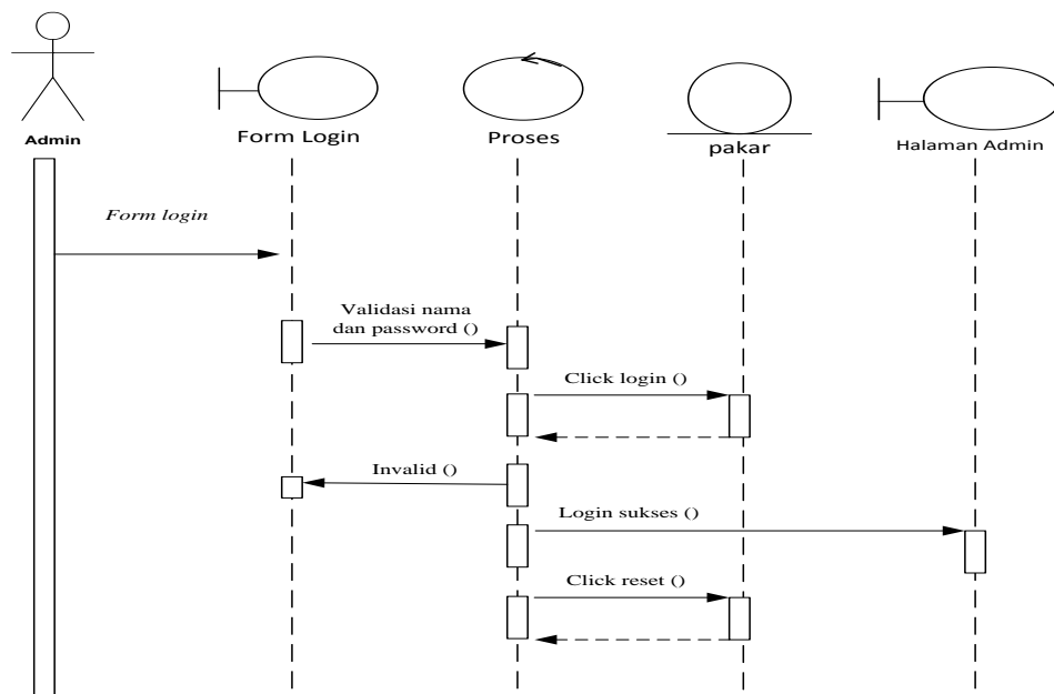
Gambar III.15. Sequence Diagram Login
