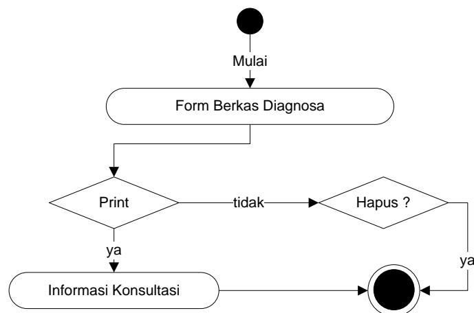
Gambar III.13. Activity Diagram Berkas Diagnosa
