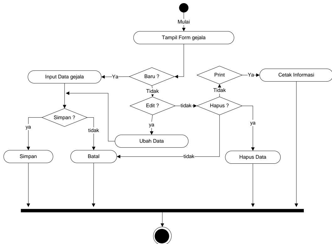
Gambar III.7. Activity Diagram Data Gejala
