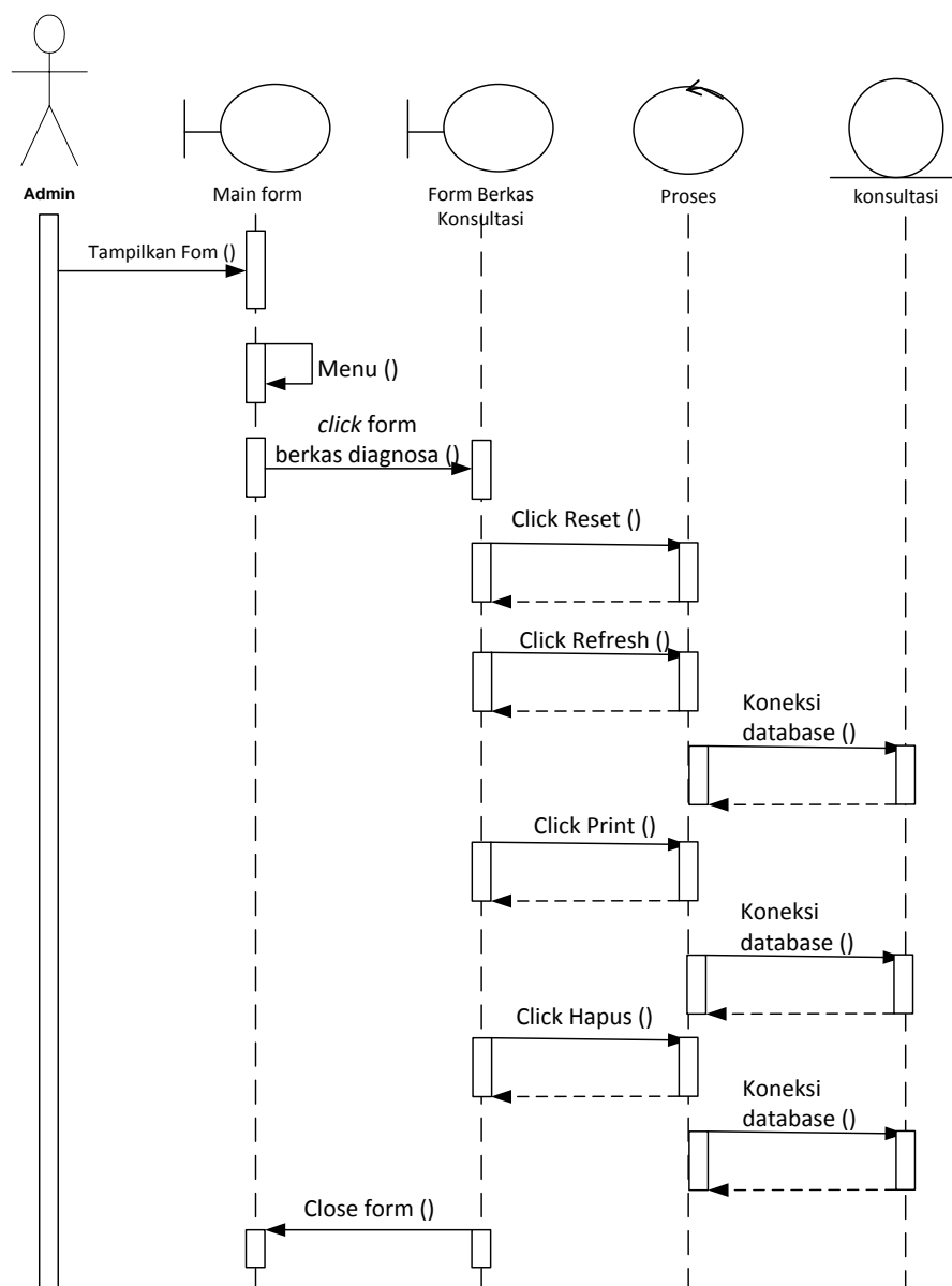
Gambar III.18. Sequence Diagram Data Berkas Diagnosa
