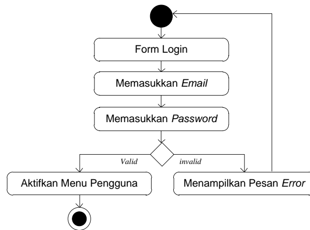
Gambar III.11. Activity Diagram Login
