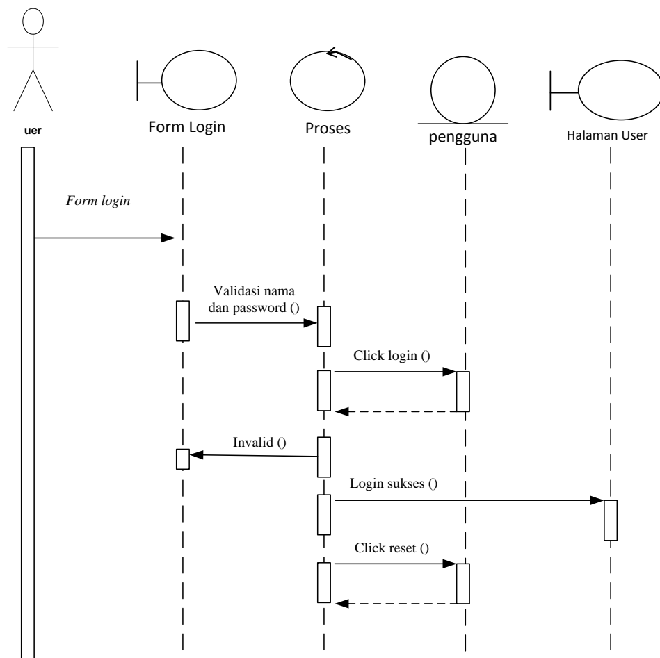
Gambar III.21. Sequence Diagram Login
