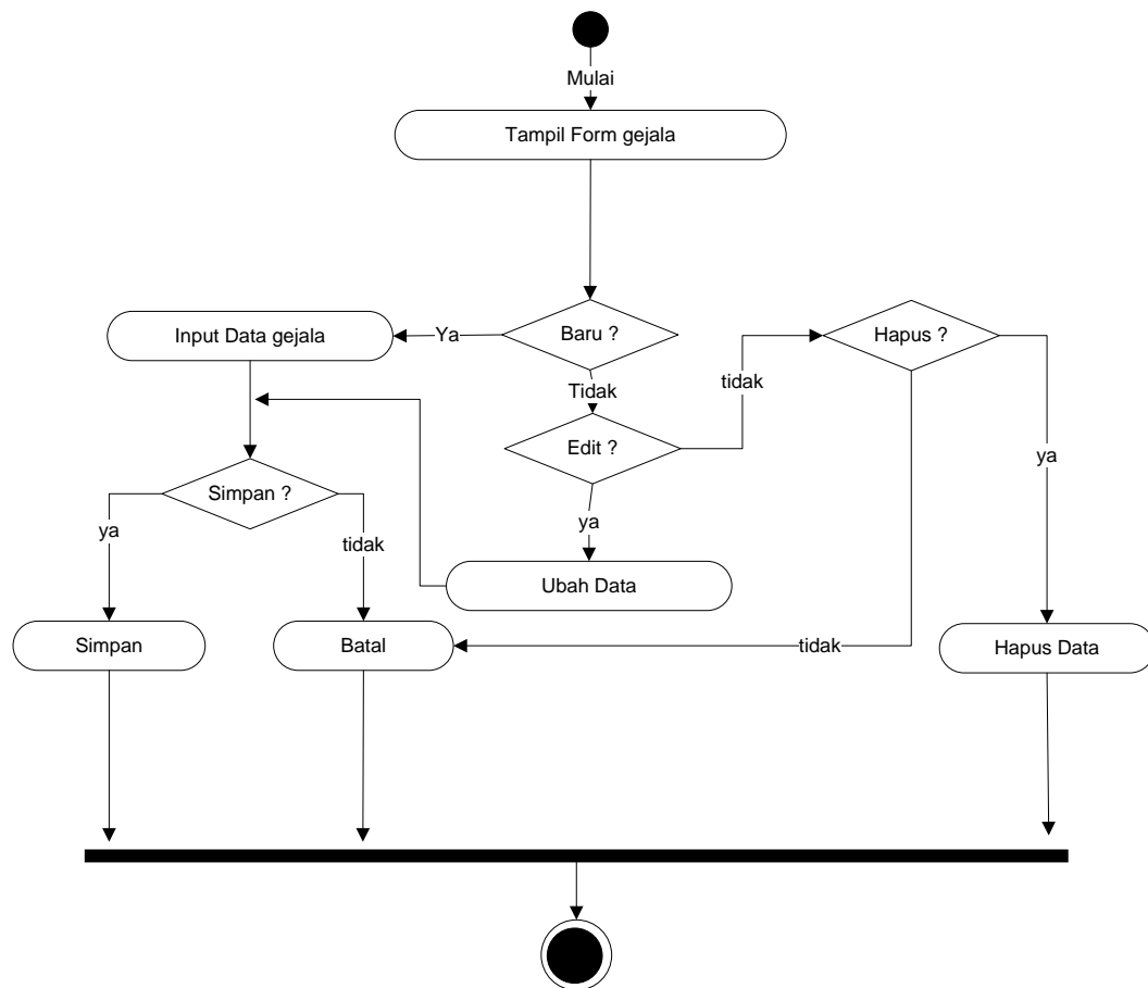
Gambar III.10. Activity Diagram Data Pakar
