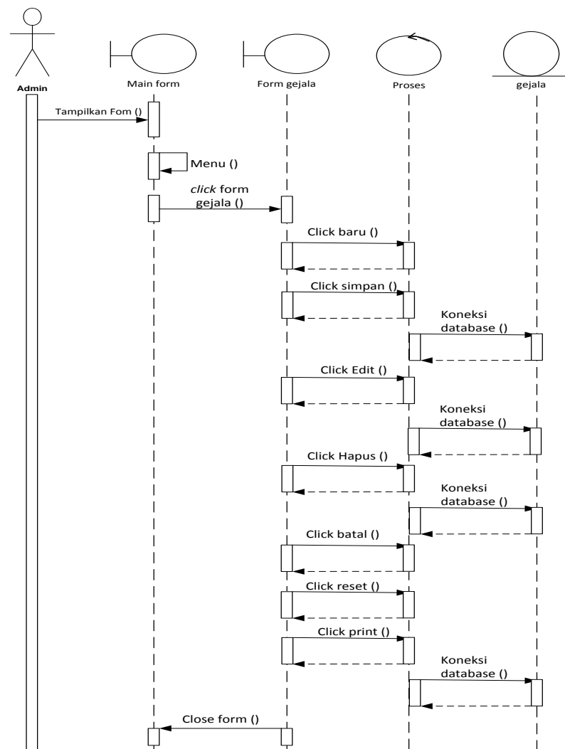
Gambar III.17. Sequence Diagram Data Gejala
