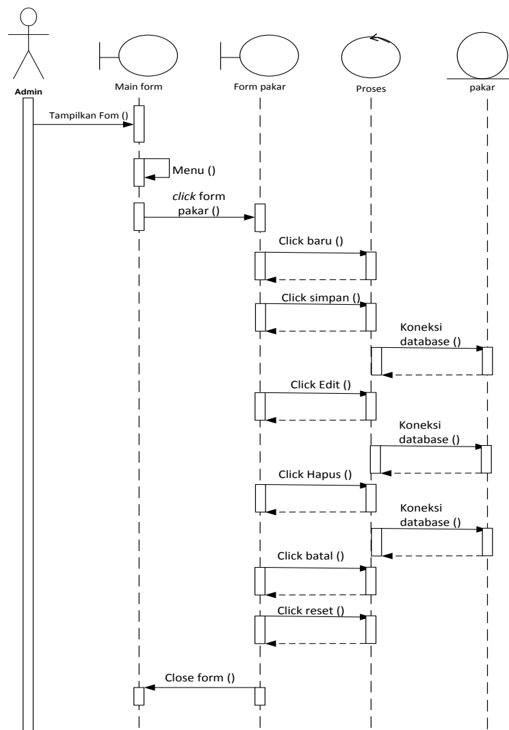
Gambar III.20. Sequence Diagram Data Pengaturan Akun Pakar
