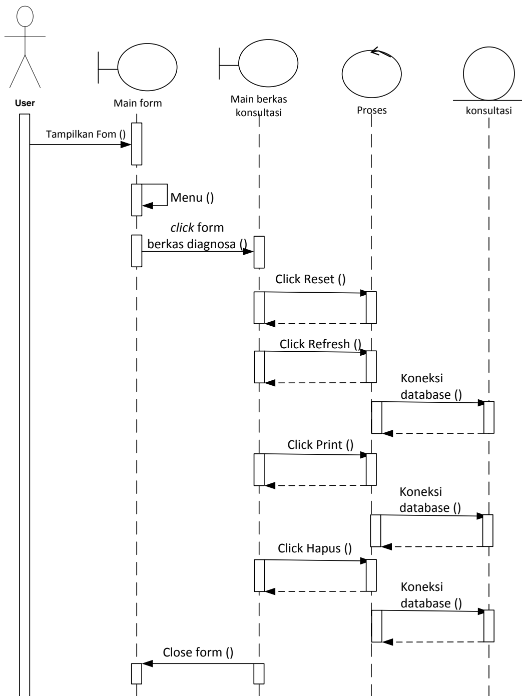
Gambar III.23. Sequence Diagram Berkas Diagnosa
