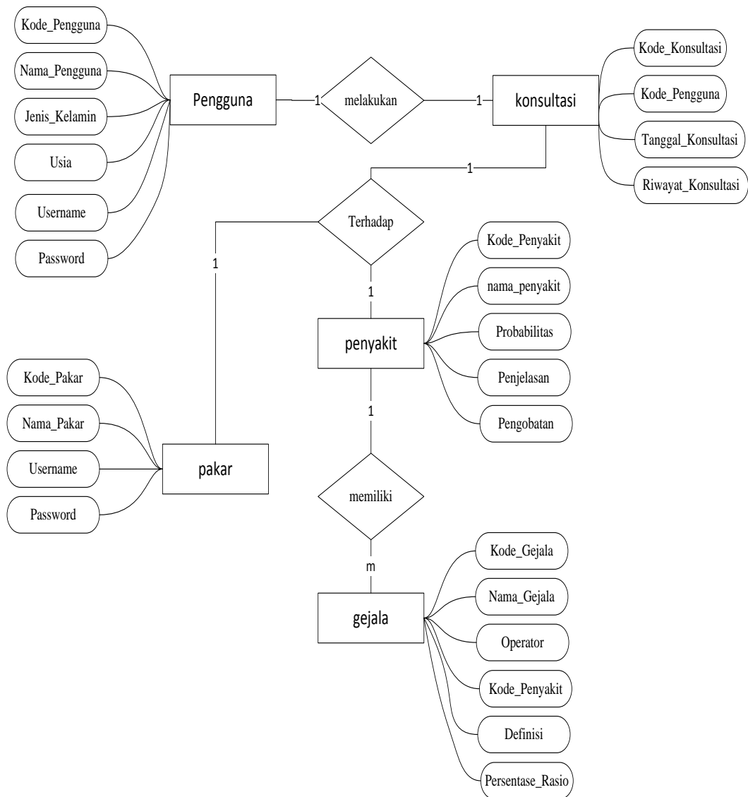
Gambar III.38. Diagram ERD
