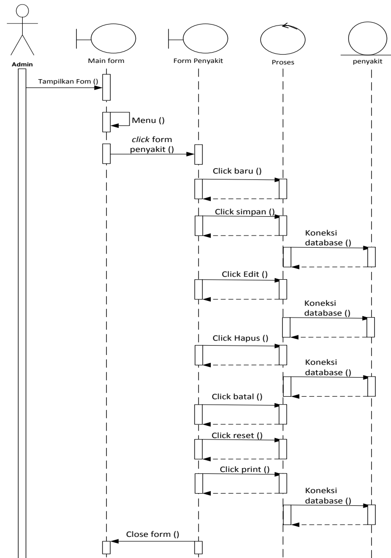
Gambar III.16. Sequence Diagram Data Penyakit
