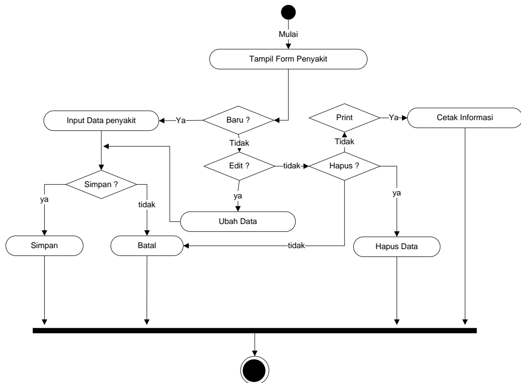
Gambar III.6. Activity Diagram Data Penyakit
