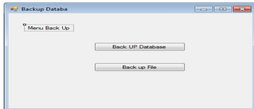
Gambar IV.14. Menu Backup
