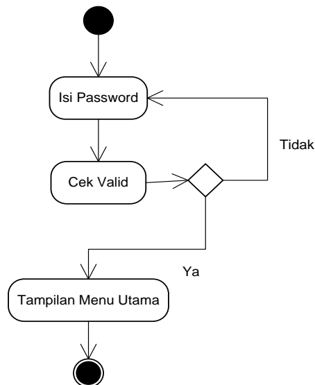
Gambar III.23 Activity Diagram Login Admin
