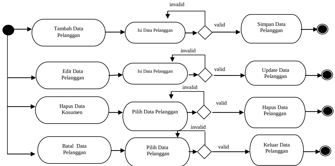
Gambar III.24. Activity Diagram Form Input Data Pelanggan
