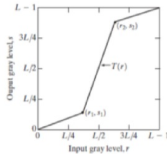
Gambar 2. Fungsi Contrast Stretching
