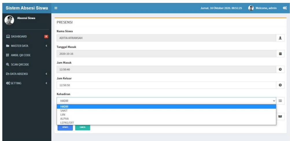
Gambar IV.11. Tampilan Publish Absensi
