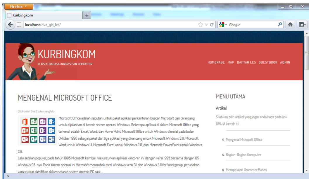
Gambar IV.1. Tampilan HomePage
