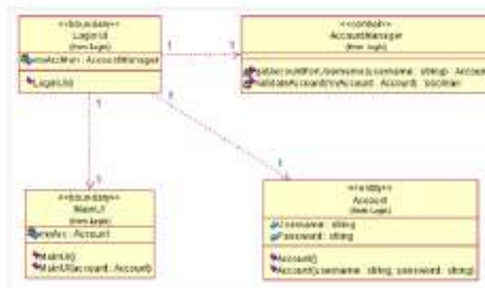
Gambar II.2. Contoh Class Diagram (Sumber : Haviluddin ; 2011 : 3)
