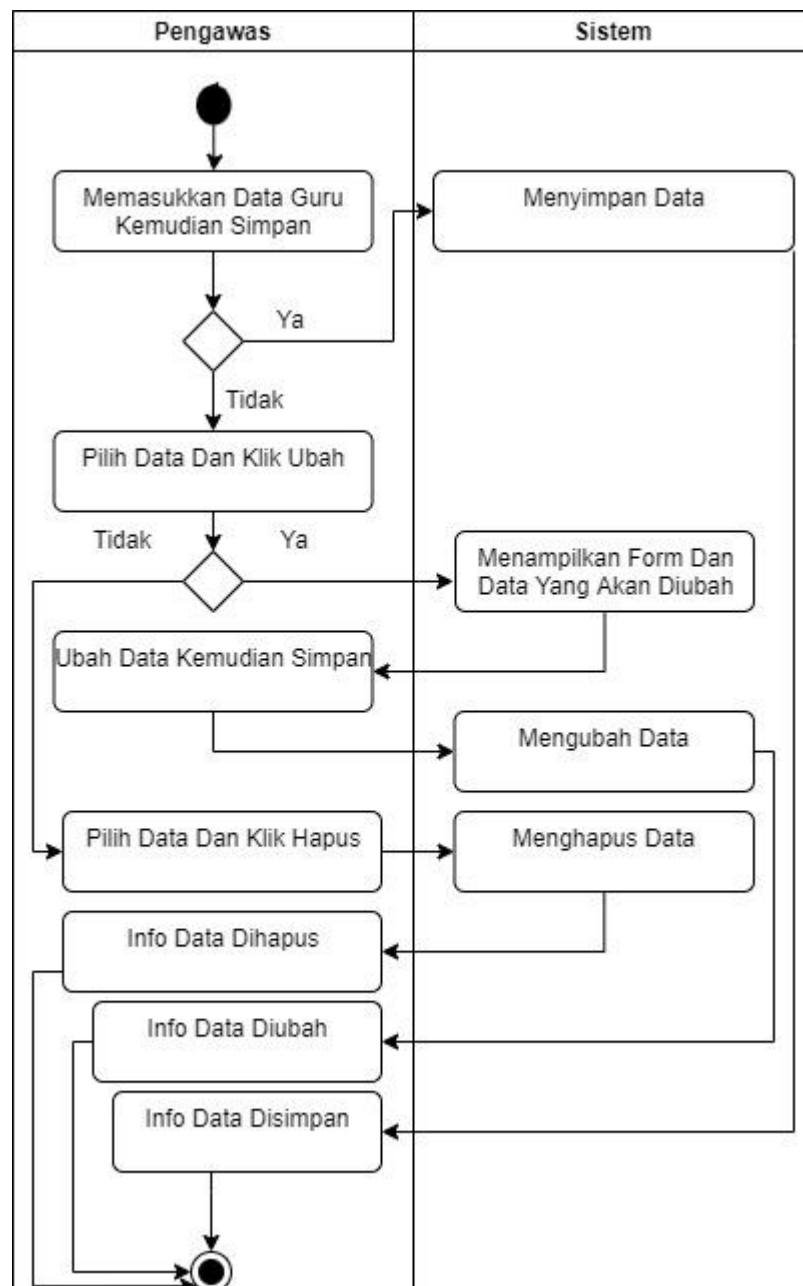
Gambar III.7. Activity Diagram Guru Bagian Pengawas
