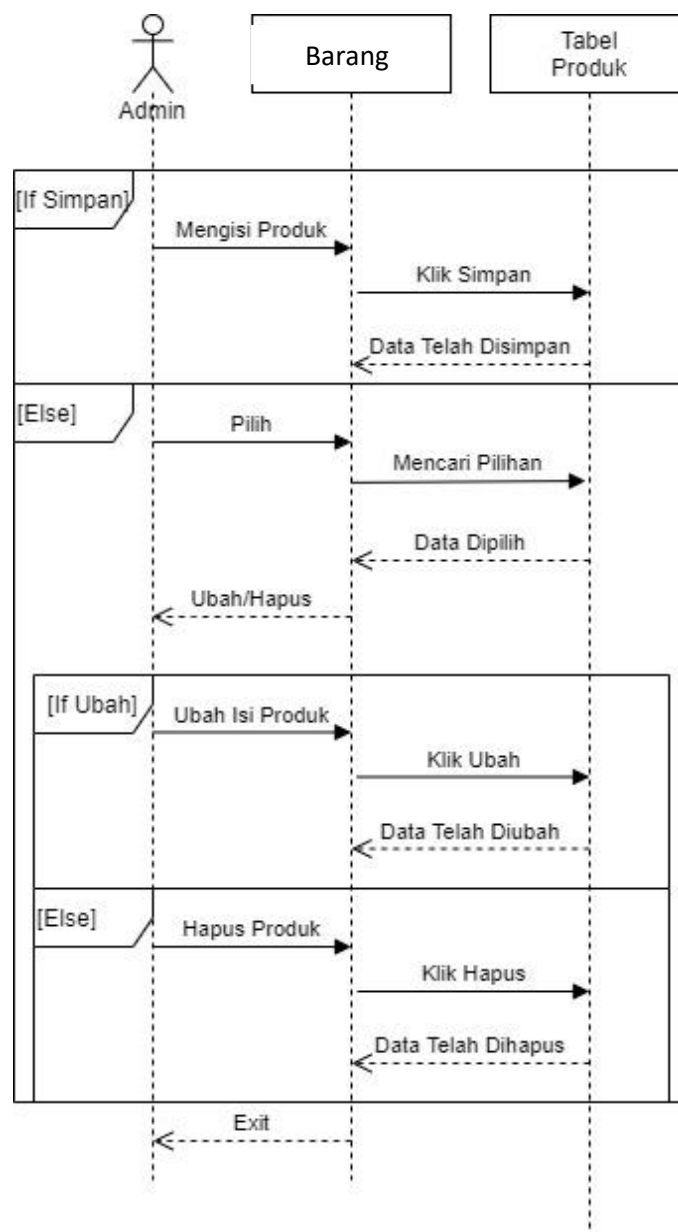
Gambar III.12. Sequence Diagram Barang Bagian Admin
