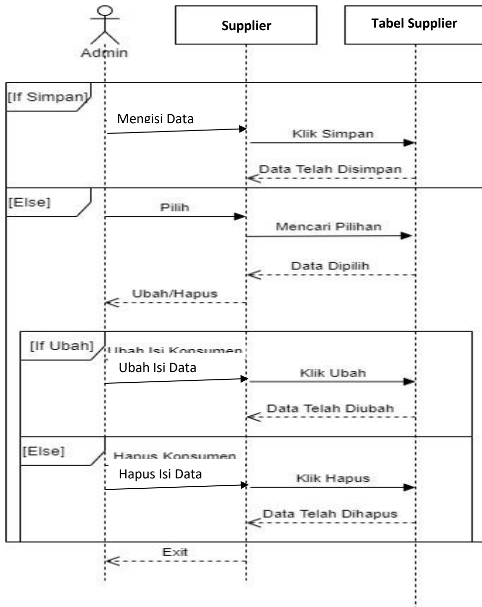
Gambar III.13. Sequence Diagram Supplier Bagian Admin
