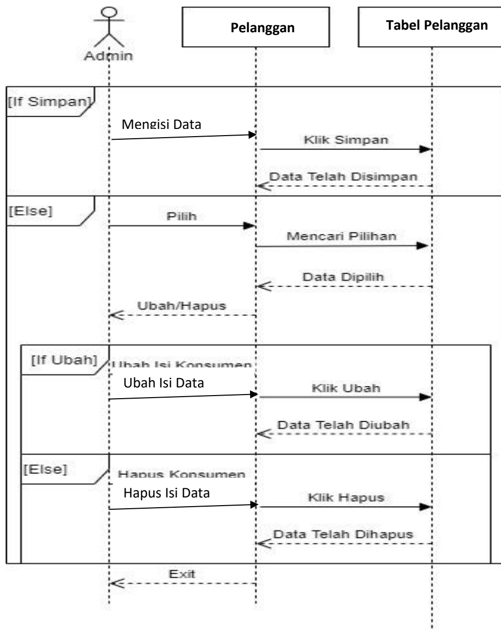
Gambar III.14. Sequence Diagram Pelanggan Bagian Admin
