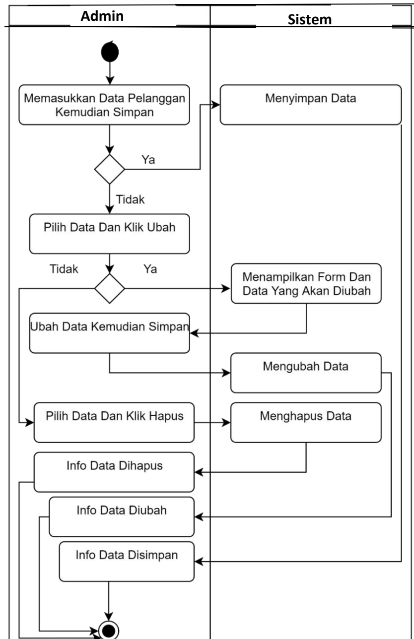
Gambar III.5. Activity Diagram Supplier Bagian Admin/Pemilik Toko
