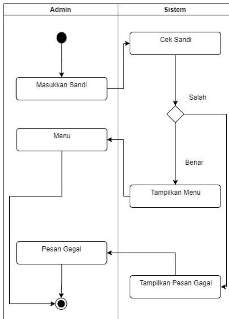
Gambar III.3. Activity Diagram Login Admin/Pemilik Toko
