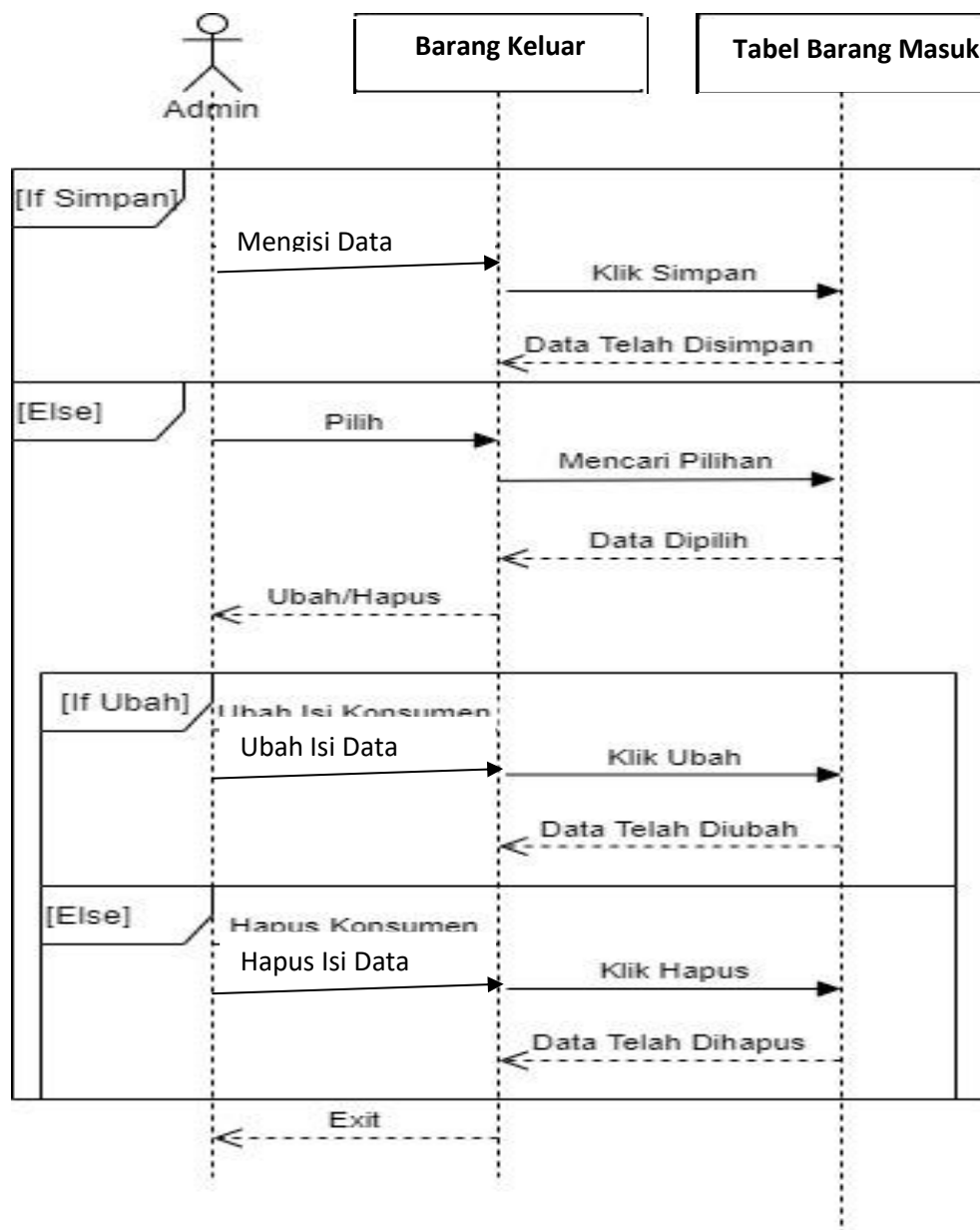
Gambar III.16. Sequence Diagram Barang Masuk Bagian Admin
