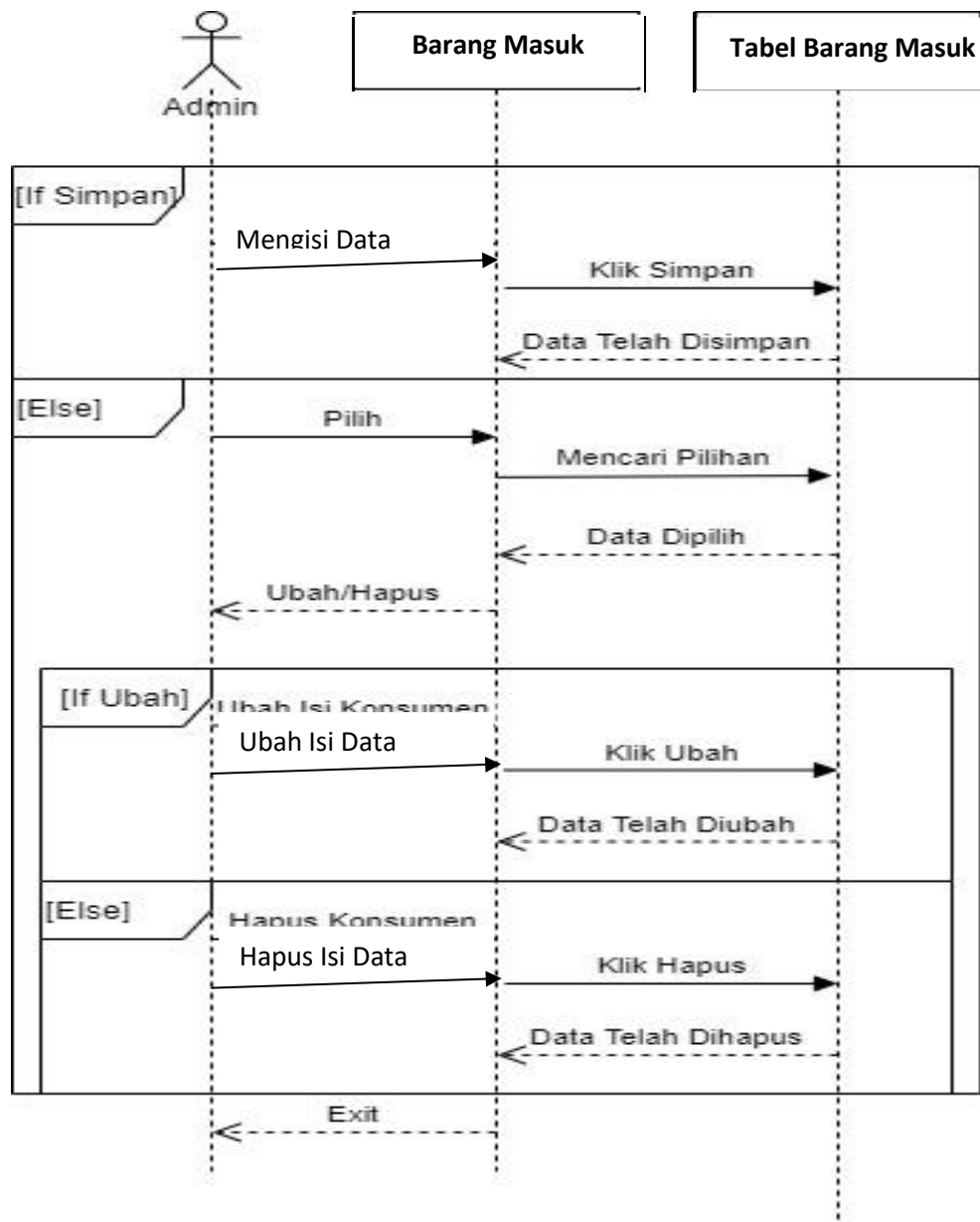
Gambar III.15. Sequence Diagram Barang Masuk Bagian Admin
