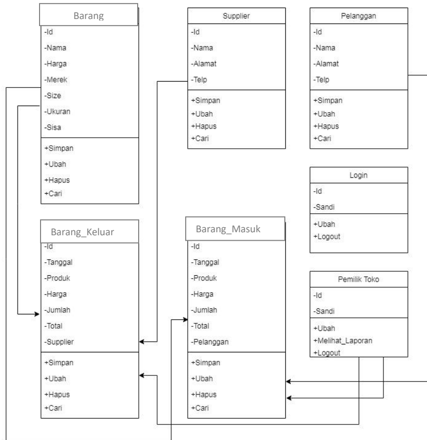
Gambar III.2. Class Diagram Perancangan Sistem Persediaan Barang
