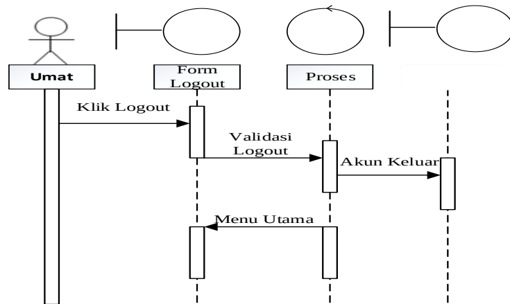
Gambar III.27. Sequence Diagram pada form logout umat
