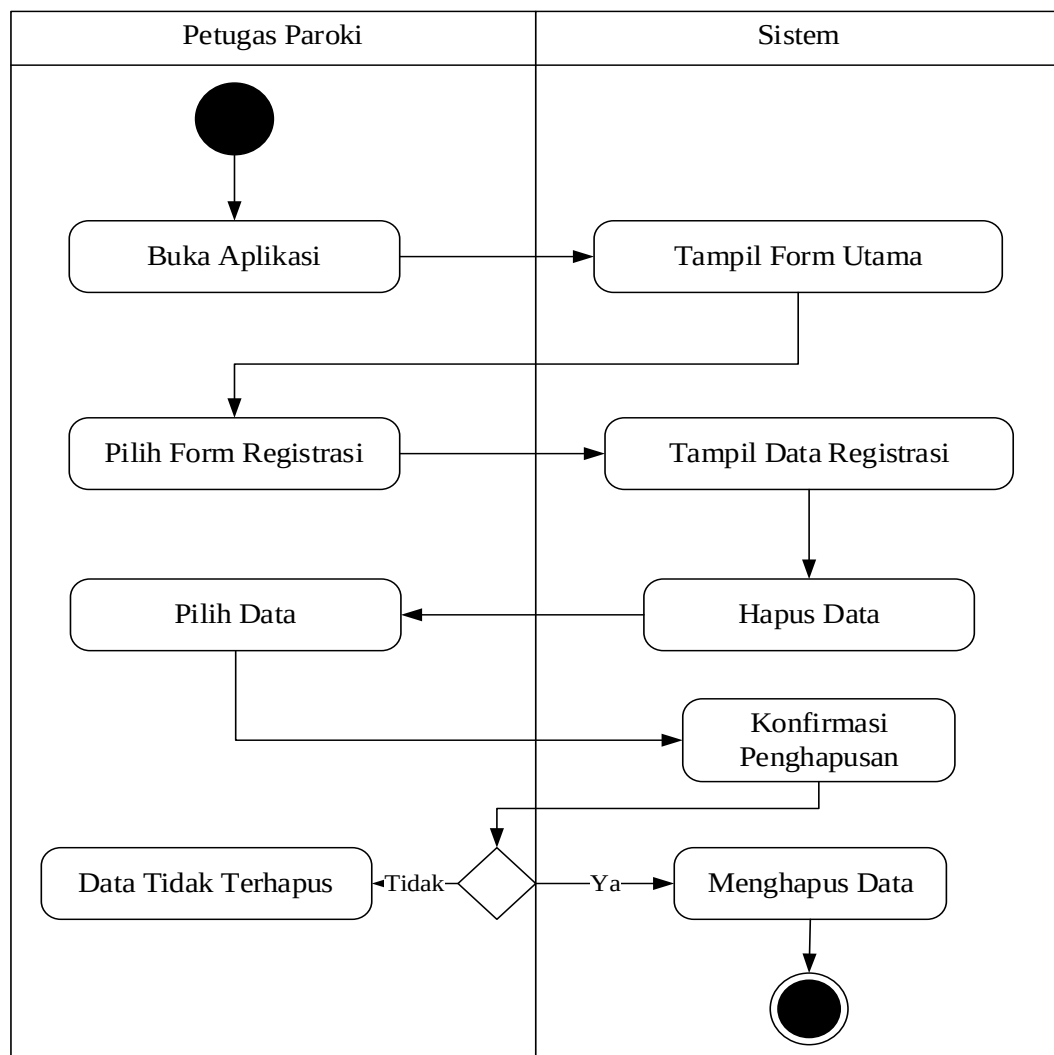
Gambar III.13. Activity Diagram Data Registrasi
