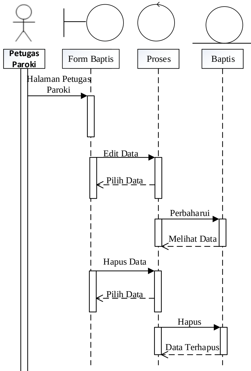
Gambar III.32. Sequence Diagram form Data Baptis
