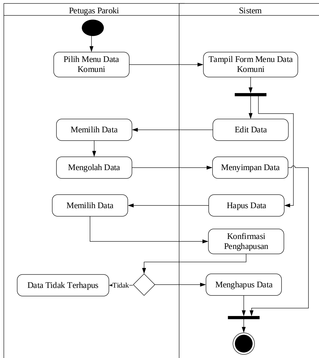
Gambar III.17. Activity Diagram Data Komuni
