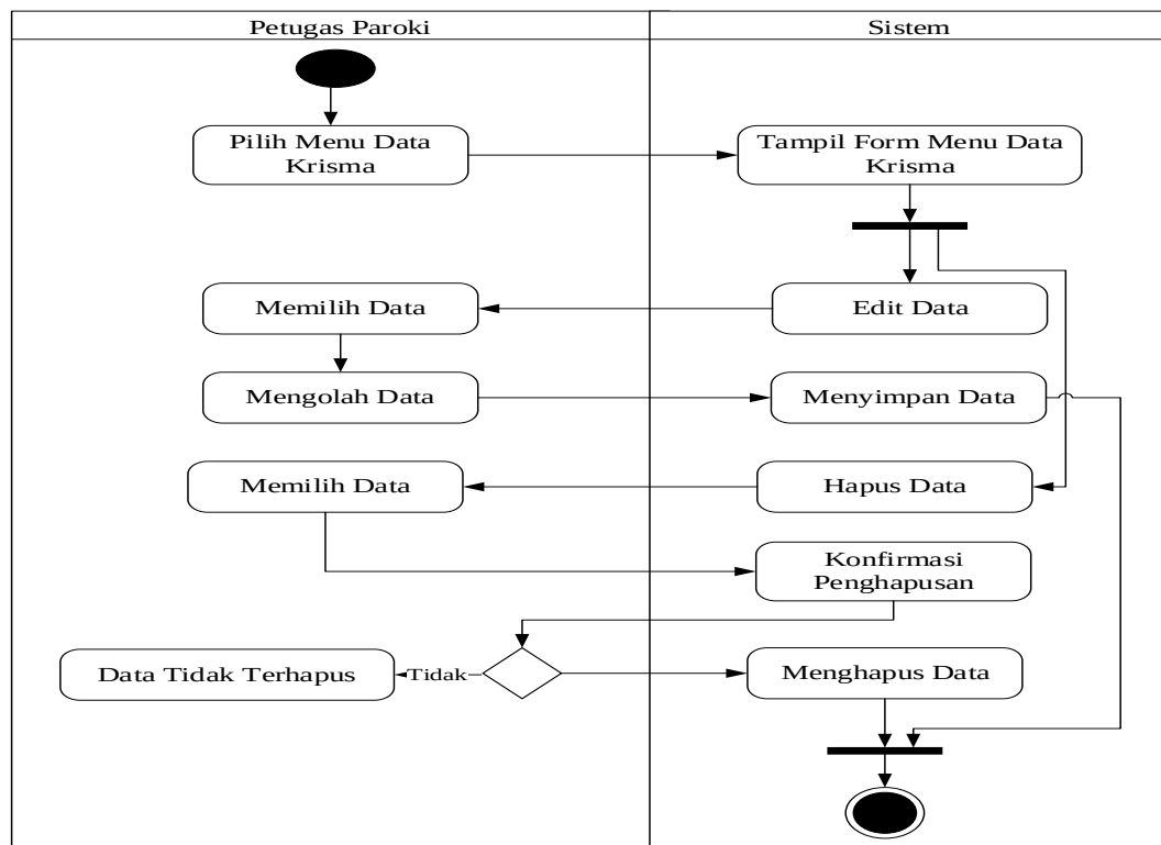
Gambar III.18. Activity Diagram Data Krisma
