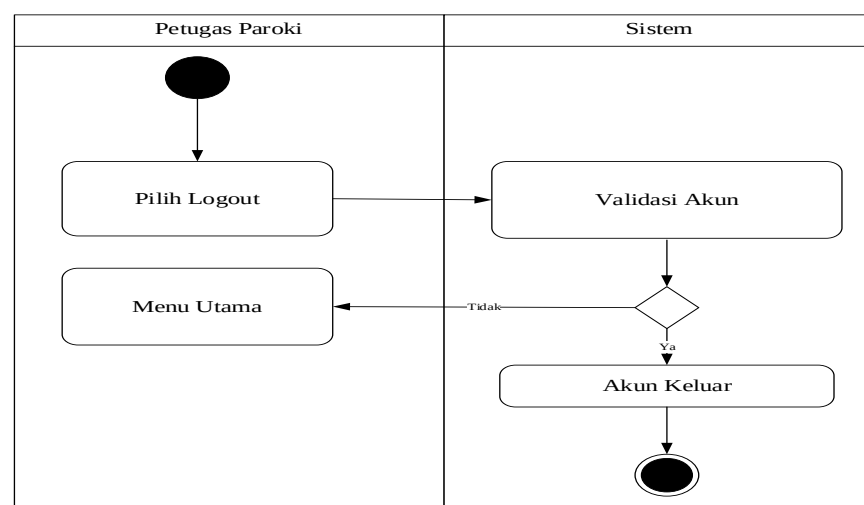
Gambar III.19. Activity Diagram Logout
