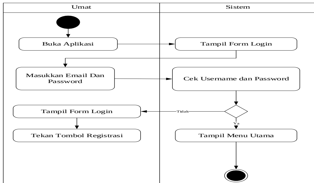
Gambar III.5. Activity Diagram Login Umat
