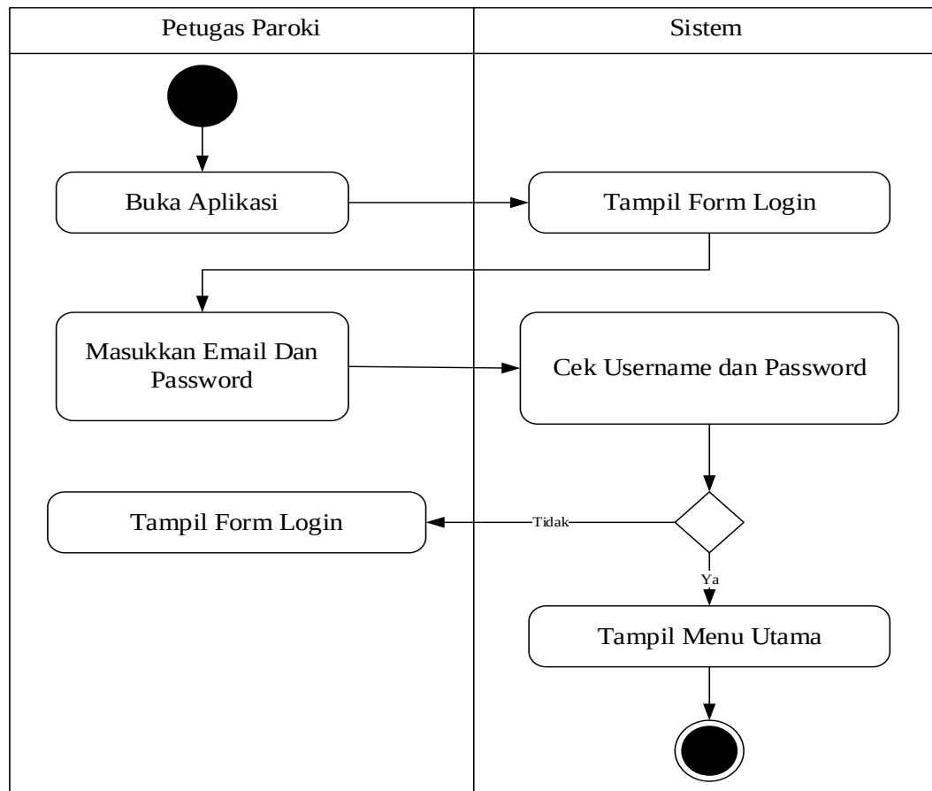
Gambar III.12. Activity Diagram Login Petugas Paroki
