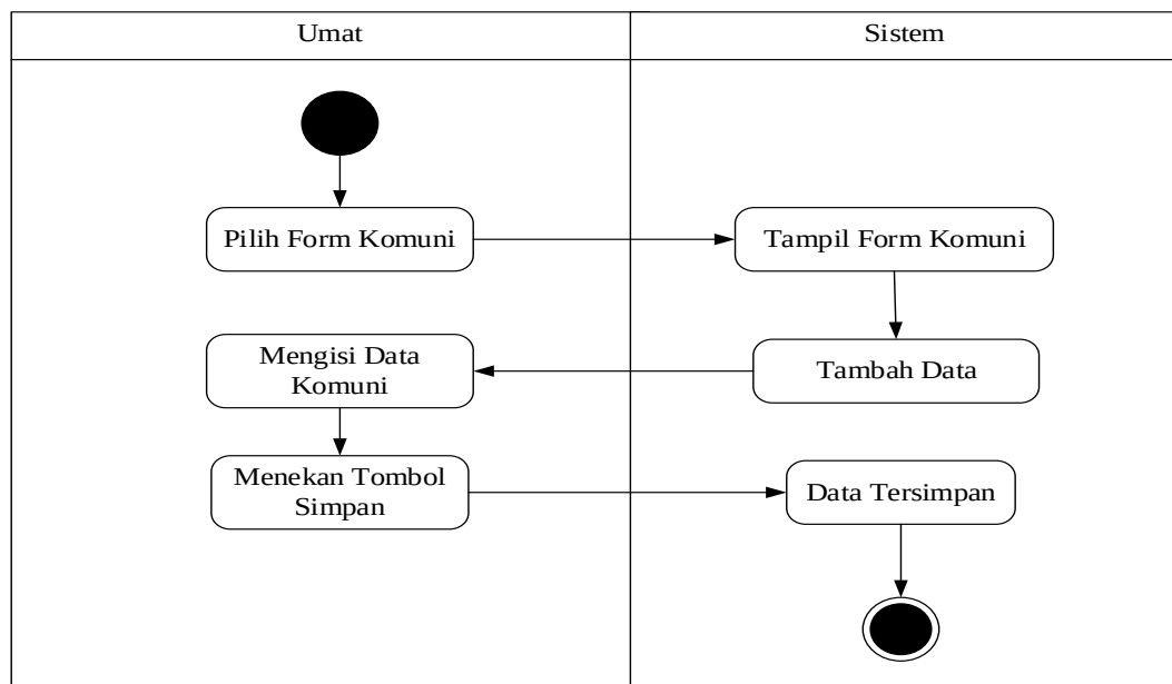
Gambar III.9. Activity Diagram Data Komuni
