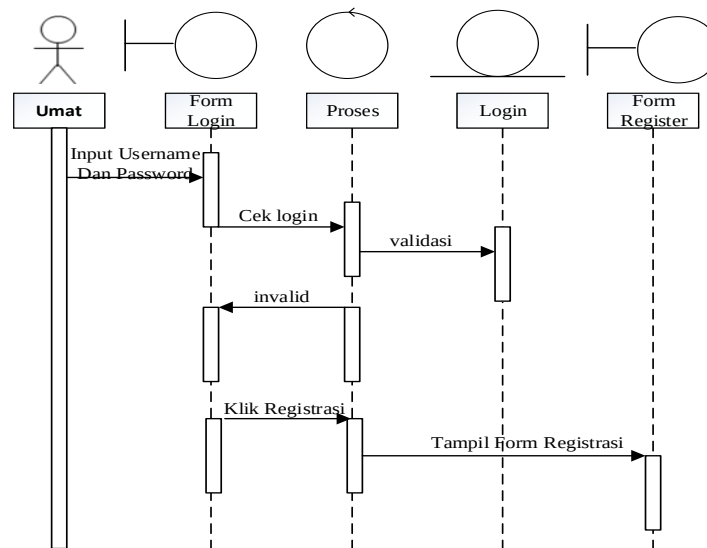
Gambar III.21. Sequence Diagram pada form login umat
