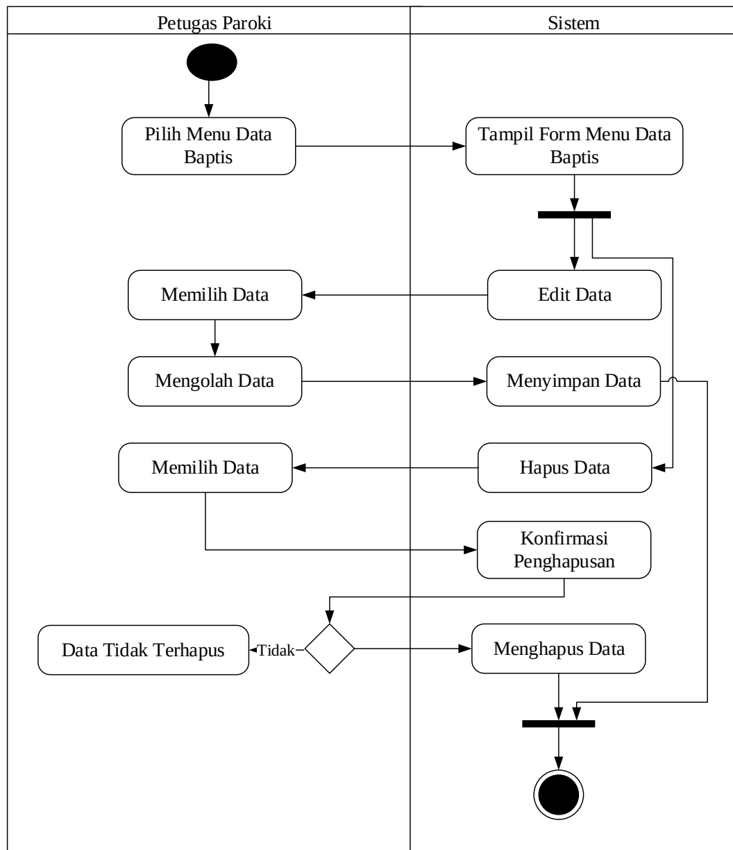
Gambar III.16. Activity Diagram Data Baptis
