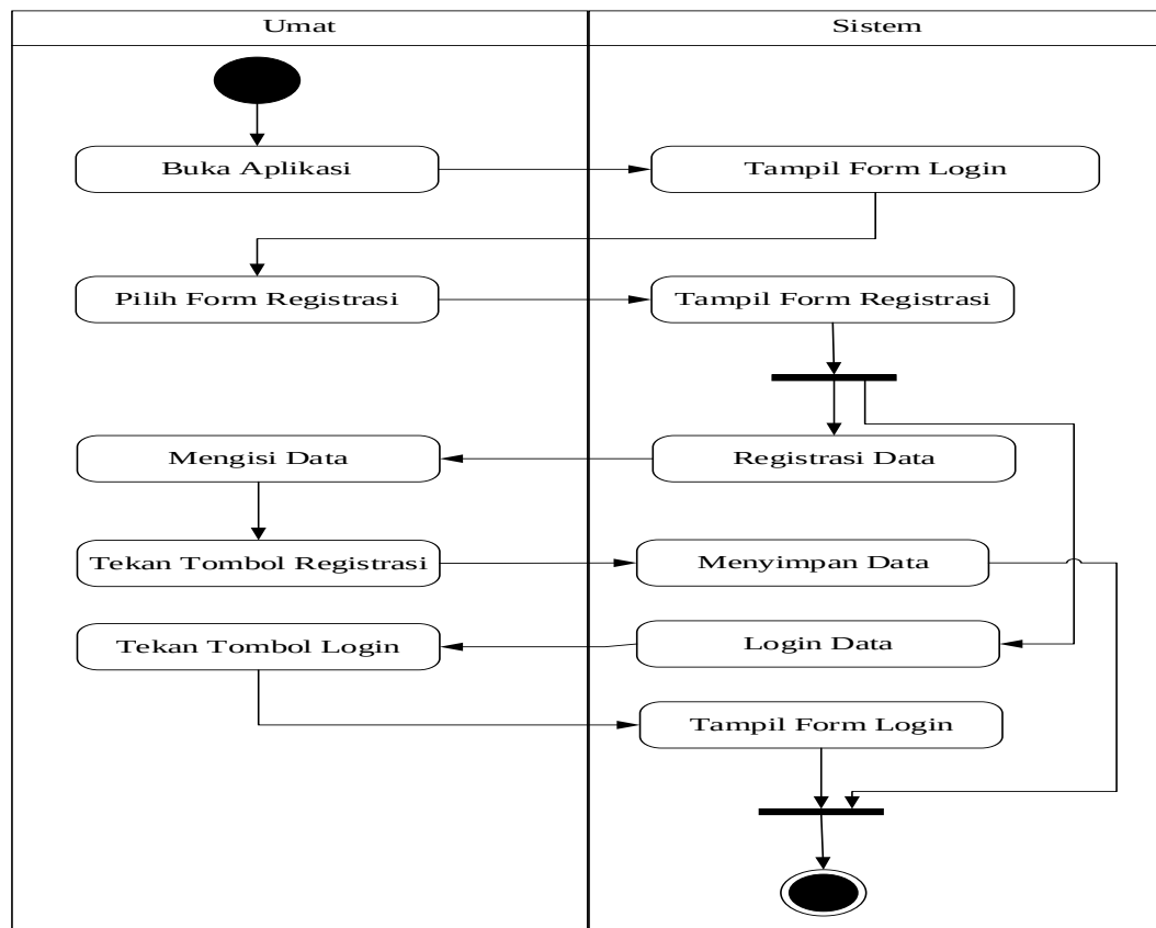
Gambar III.4. Activity Diagram Registrasi
