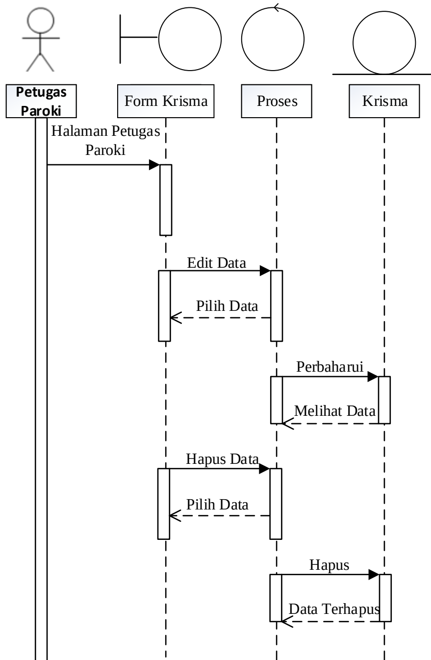
Gambar III.34. Sequence Diagram form Data Krisma
