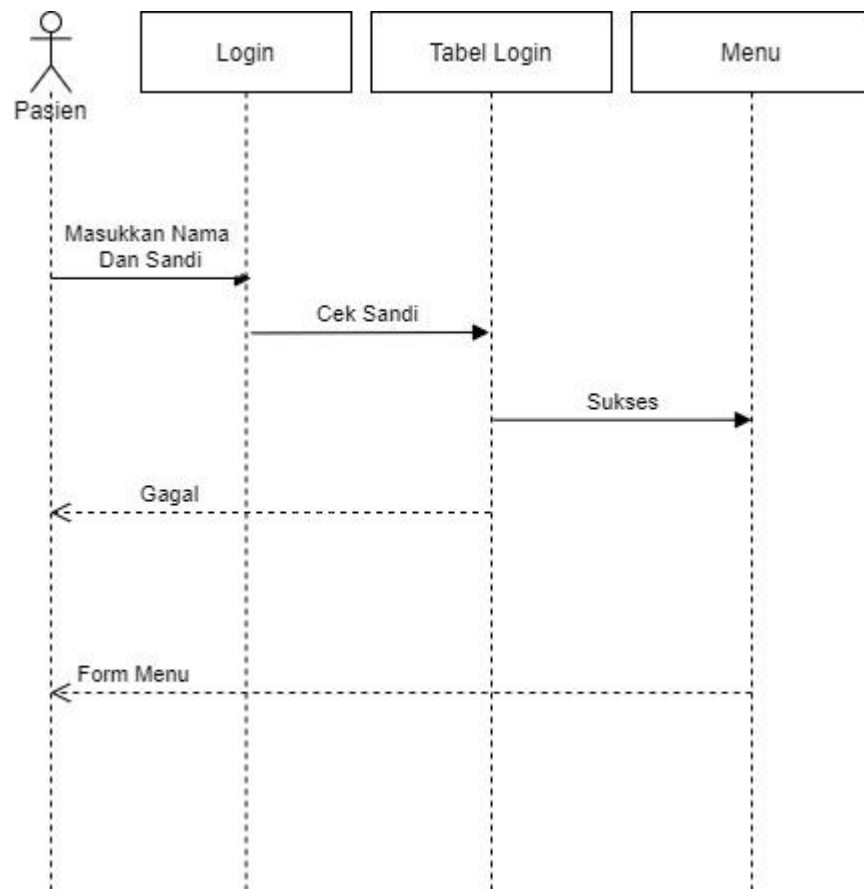
Gambar III.22. Sequence Diagram Login
