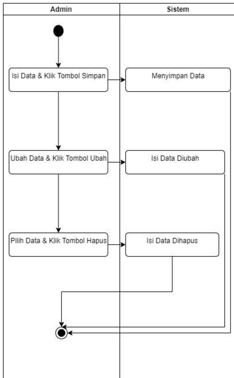
Gambar III.5. Activity Diagram Jadwal Dokter
