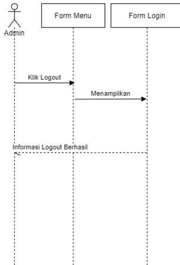
Gambar III.21. Sequence Diagram Logout
