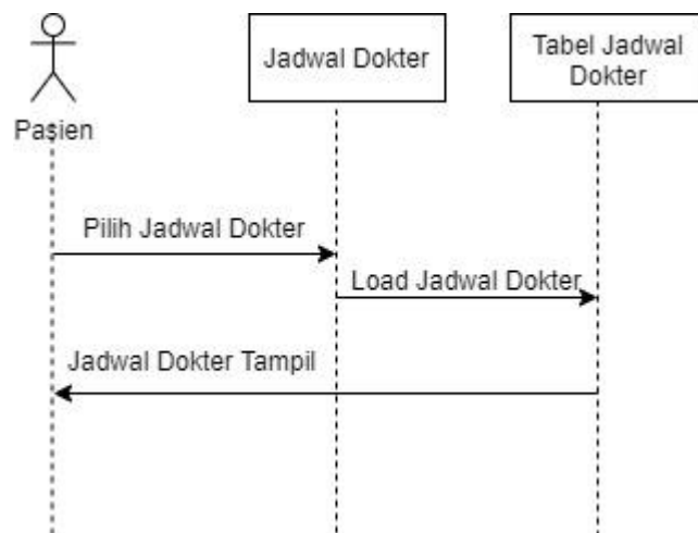
Gambar III.24. Sequence Diagram Jadwal Dokter
