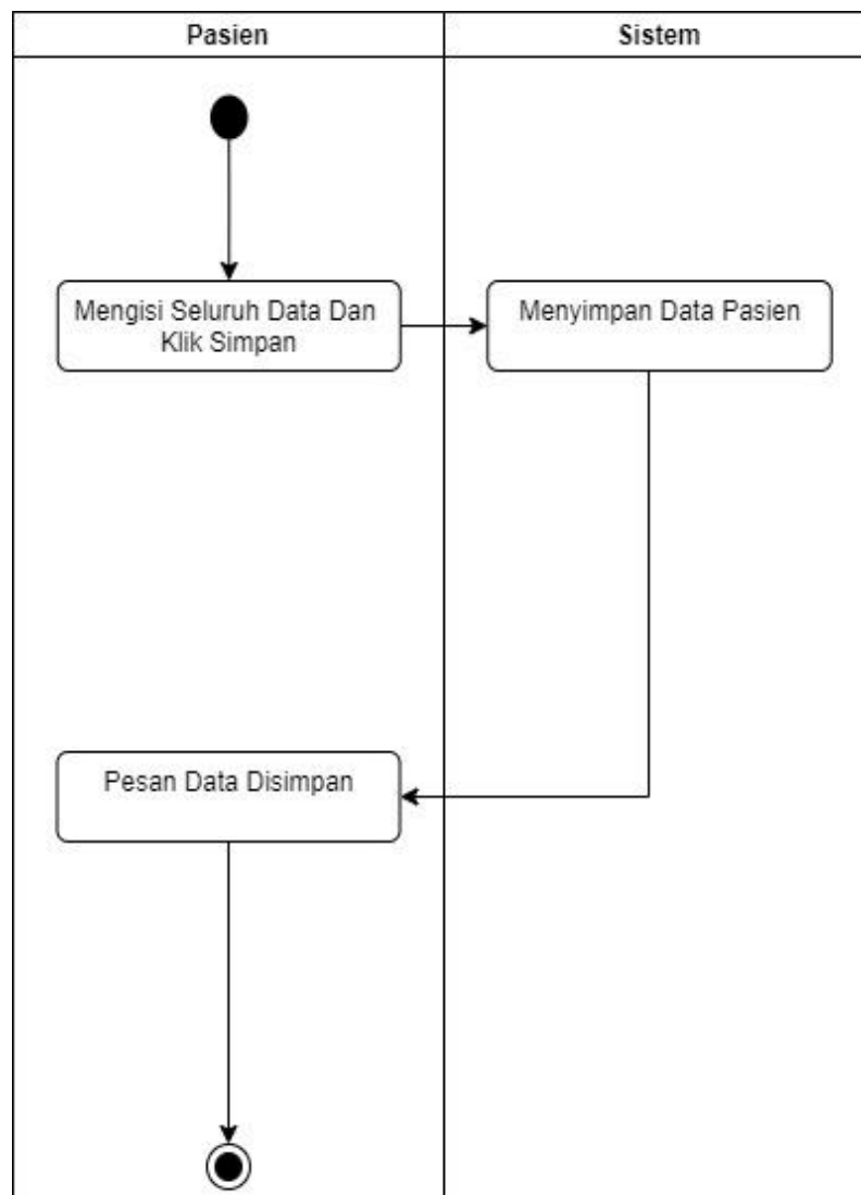
Gambar III.11. Activity Diagram Daftar
