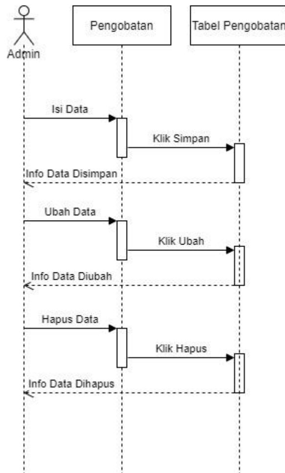
Gambar III.20. Sequence Diagram Pengobatan Gigi
