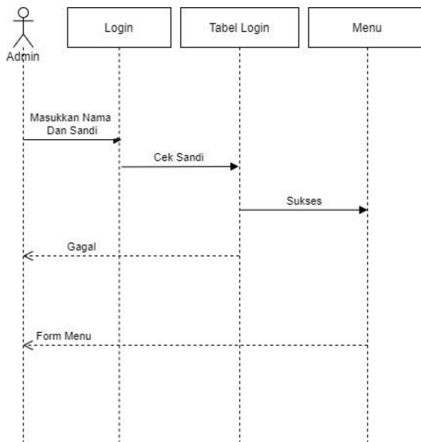
Gambar III.16. Sequence Diagram Login
