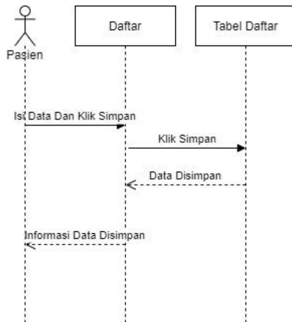
Gambar III.23. Sequence Diagram Daftar
