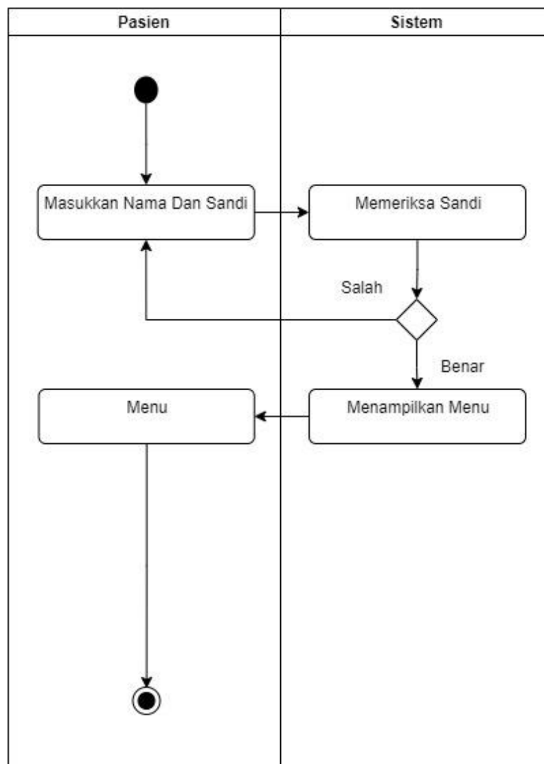
Gambar III.10. Activity Diagram Login
