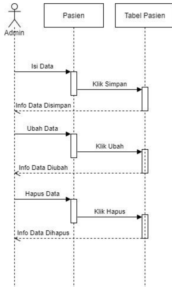
Gambar III.18. Sequence Diagram Pasien
