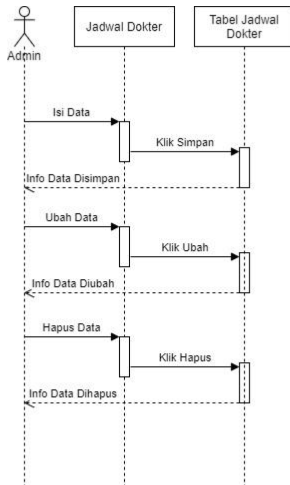
Gambar III.17. Sequence Diagram Jadwal Dokter
