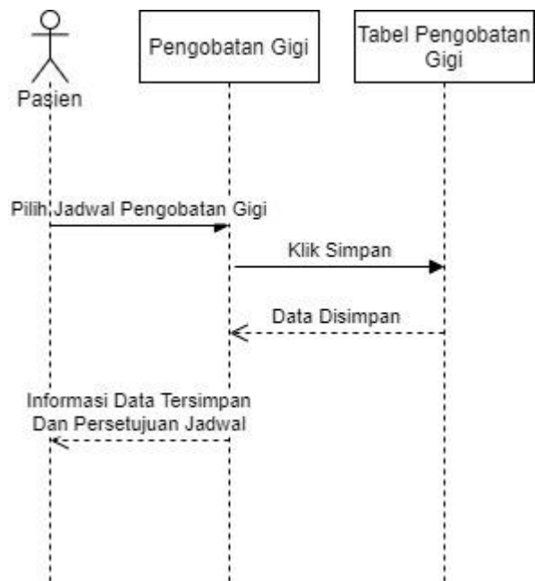
Gambar III.26. Sequence Diagram Pengobatan Gigi
