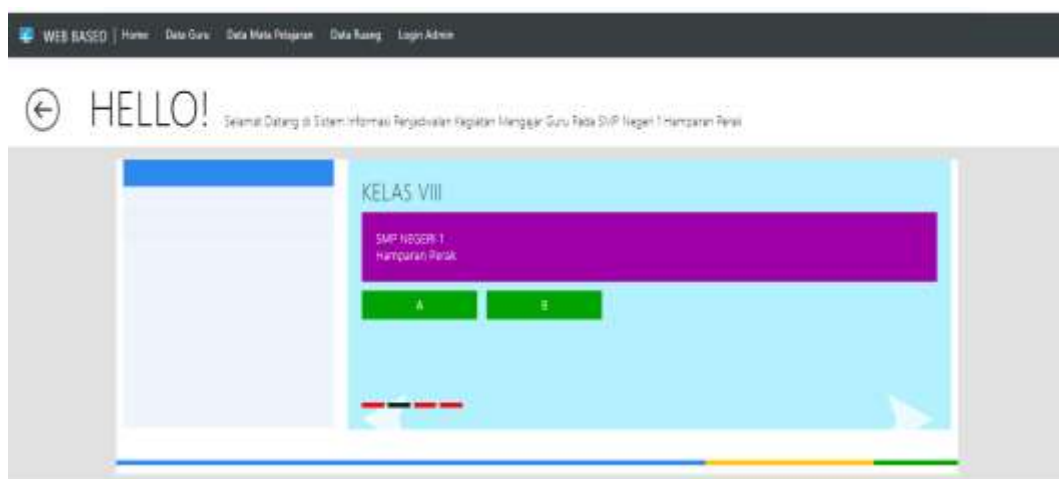
Gambar IV.7. Halaman Home
