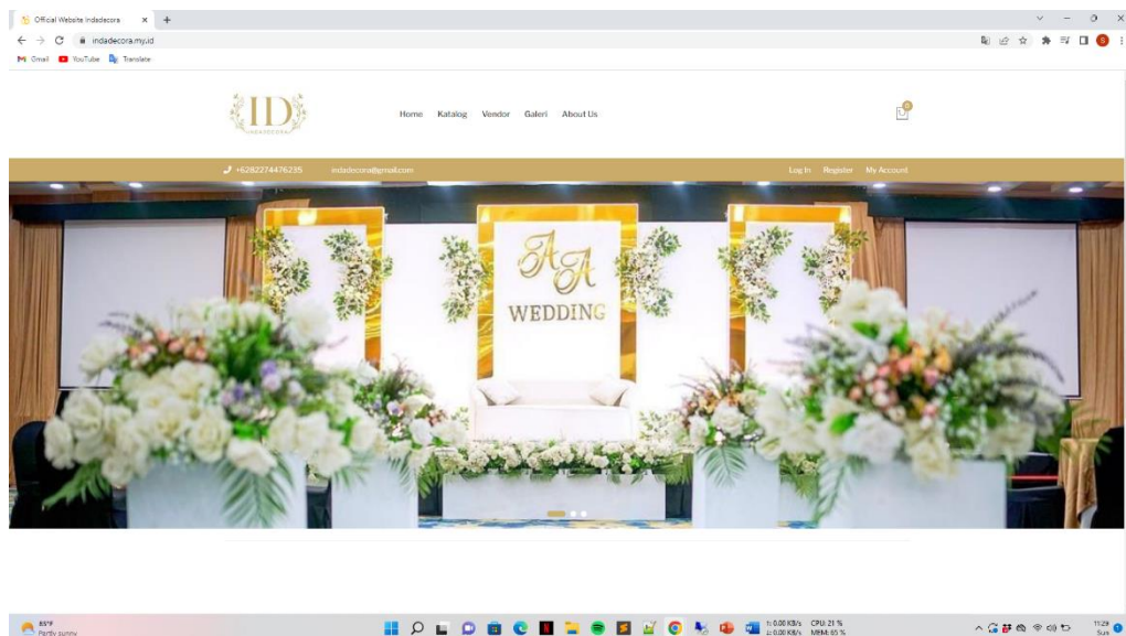
Gambar IV.1 Tampilan Home
