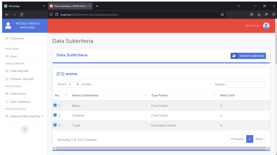
Gambar IV.8 Tampilan Halaman sub kriteria
