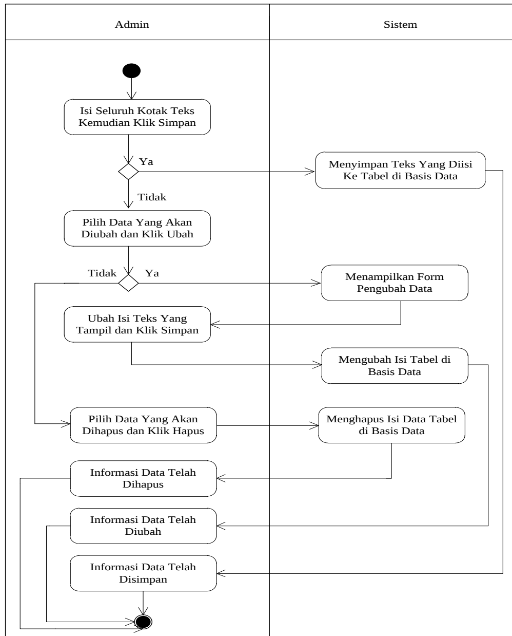
Gambar III.6. Activity Diagram Form Lokasi
