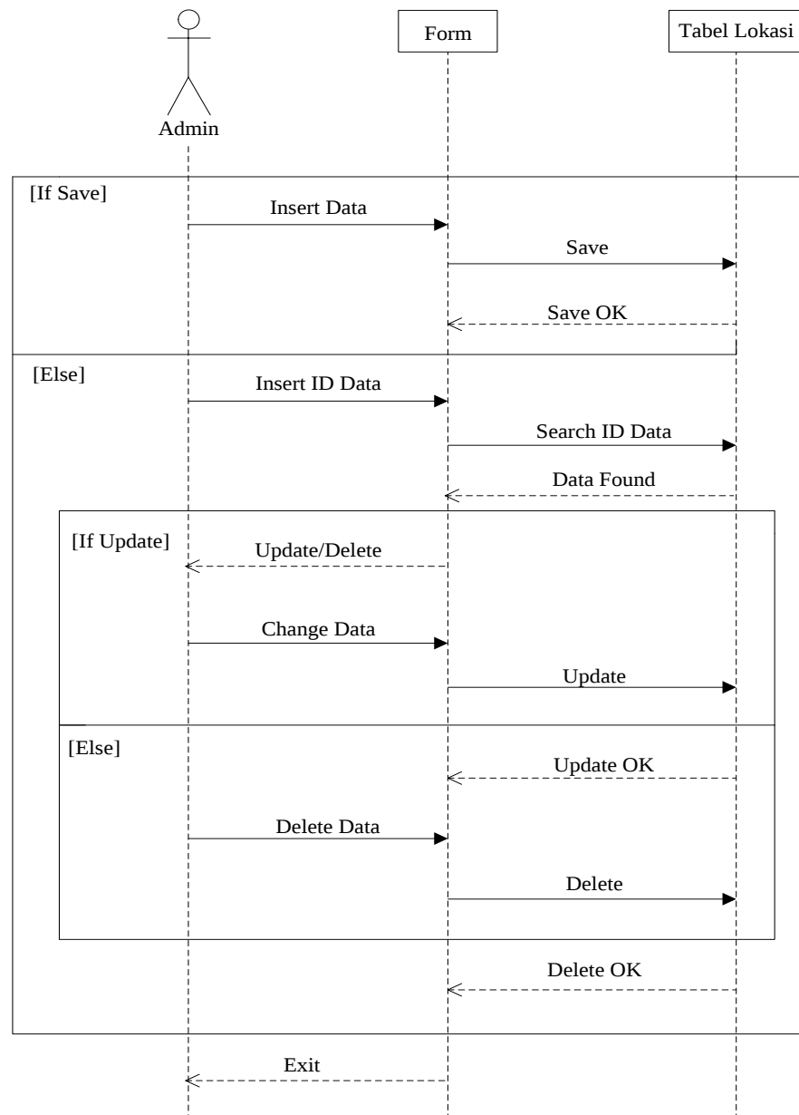
Gambar III.13. Sequence Diagram Form Lokasi
