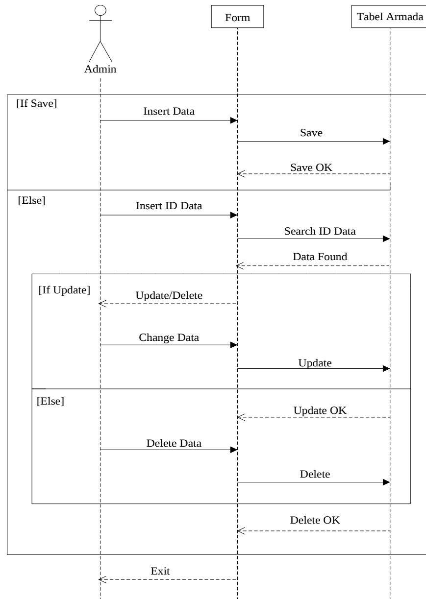
Gambar III.14. Sequence Diagram Form Armada
