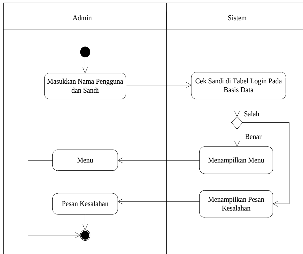
Gambar III.4. Activity Diagram Form Login
