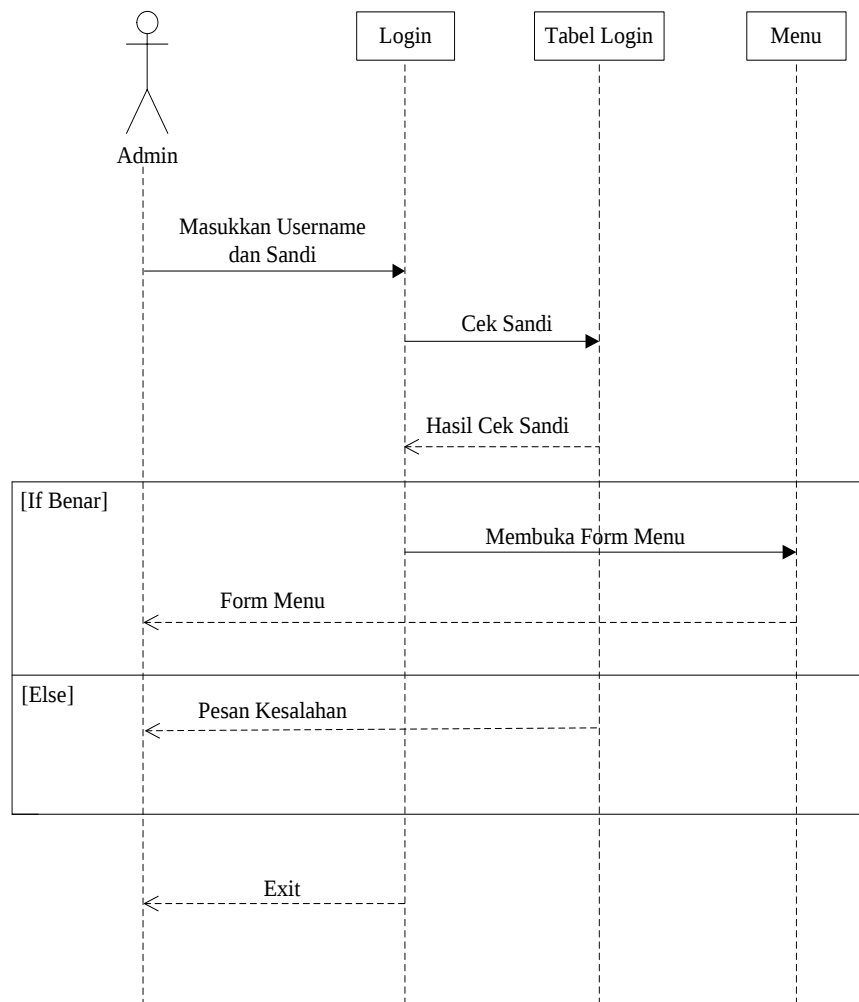
Gambar III.11. Sequence Diagram Form Login
