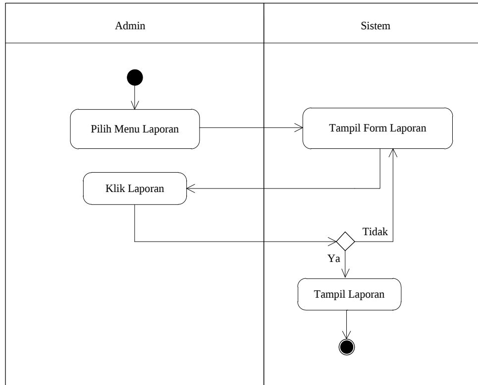
Gambar III.9. Activity Diagram Laporan Eksekutif
