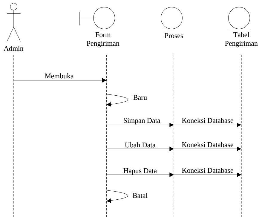
Gambar III.15. Sequence Diagram Form Pengiriman
