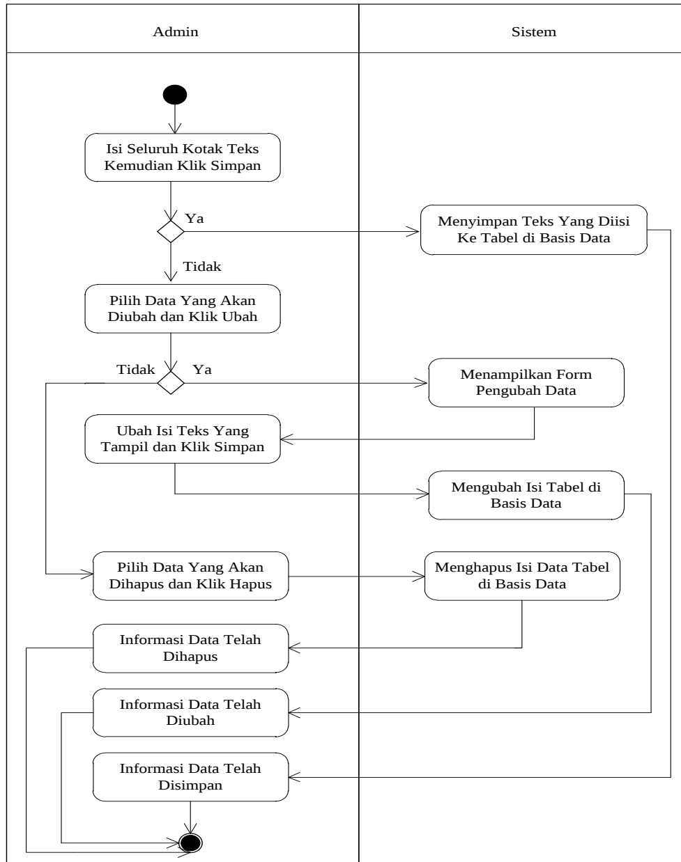
Gambar III.5. Activity Diagram Form Barang
