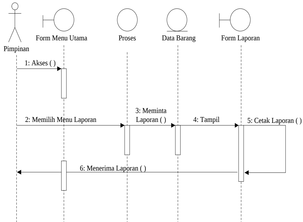
Gambar III.16. Sequence Diagram Form Laporan Eksekutif
