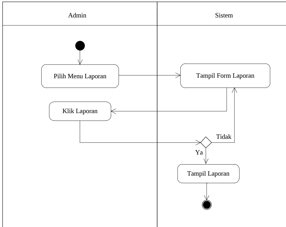
Gambar III.10. Activity Diagram Laporan Grafik
