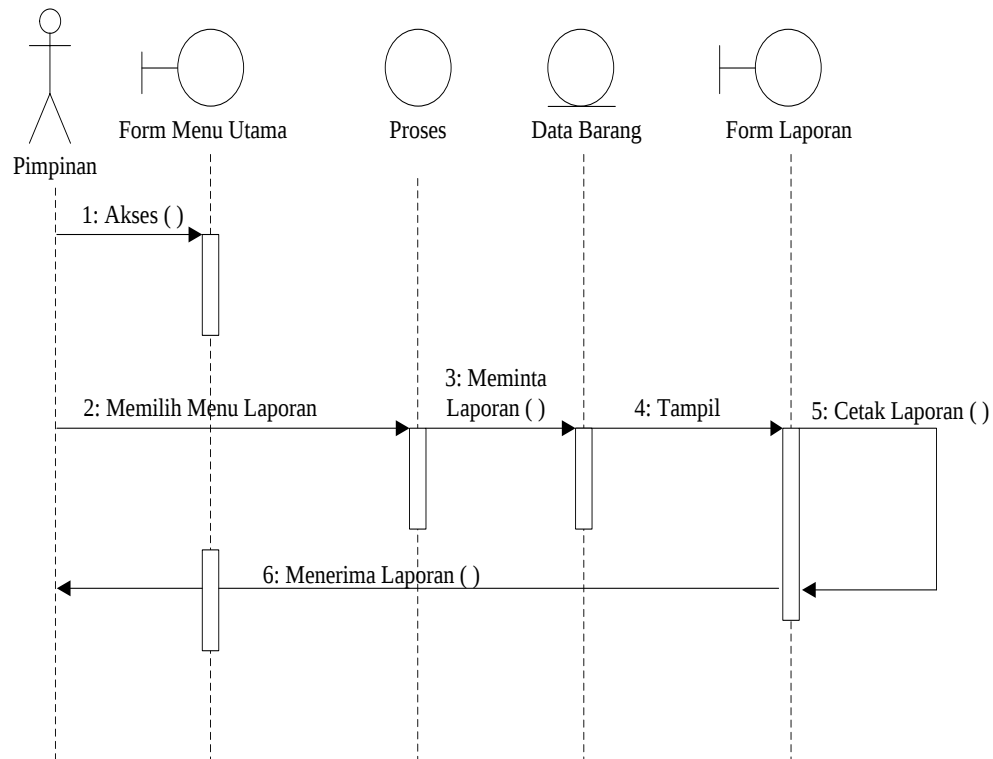
Gambar III.17. Sequence Diagram Form Laporan Grafik
