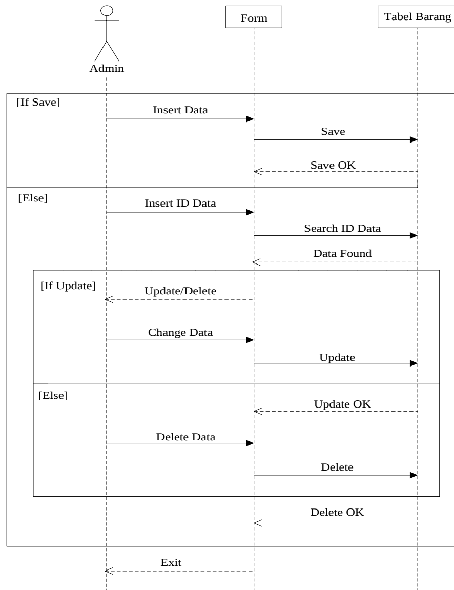
Gambar III.12. Sequence Diagram Form Barang
