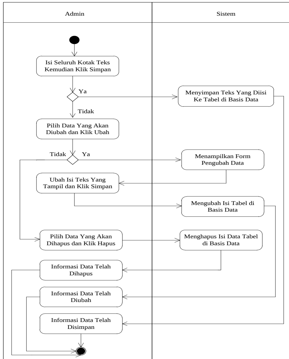
Gambar III.7. Activity Diagram Form Armada
