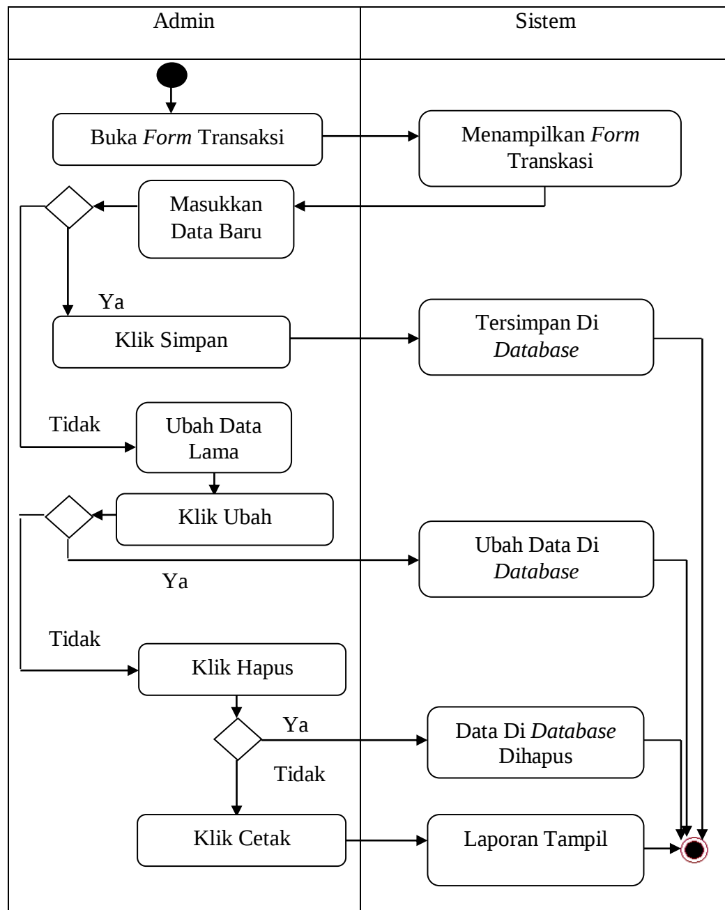
Gambar III.13. Activity Diagram Transaksi Bagian Admin
