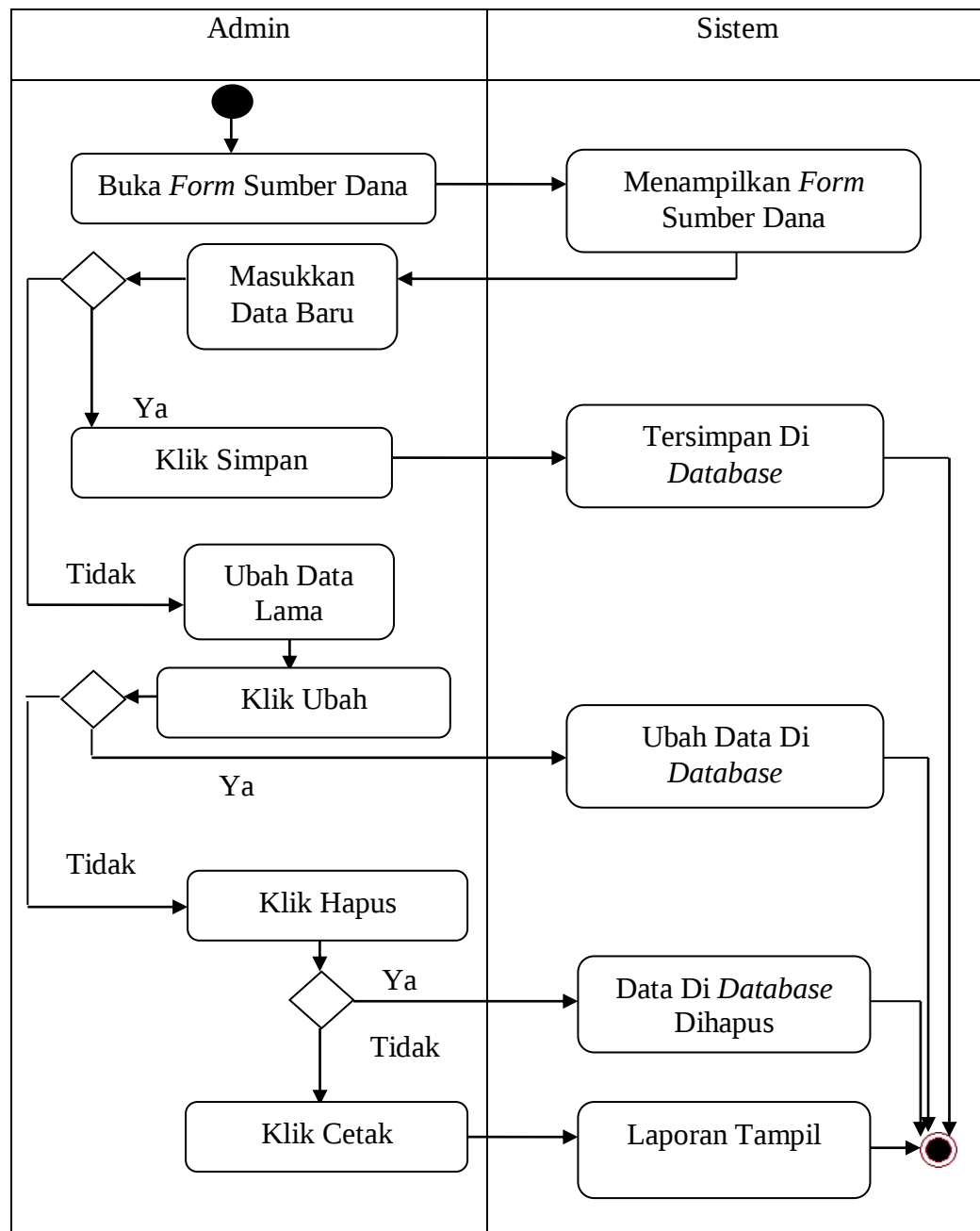
Gambar III.12. Activity Diagram Sumber Dana Bagian Admin
