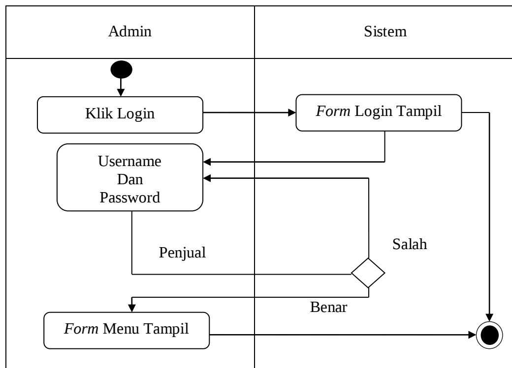
Gambar III.9. Activity Diagram Login Bagian Admin
