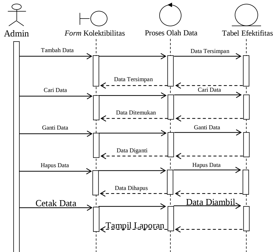
Gambar III.25. Sequence Diagram Efektifitas Bagian Admin
