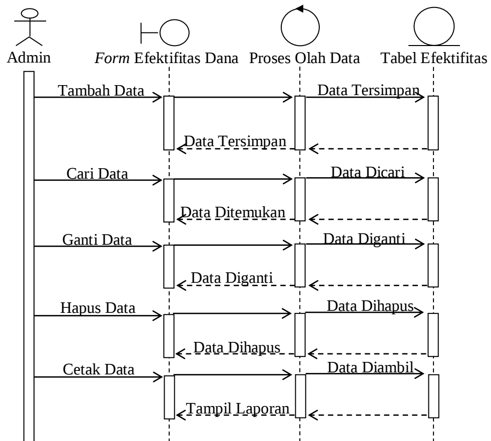
Gambar III.20. Sequence Diagram Efektifitas Bagian Admin
