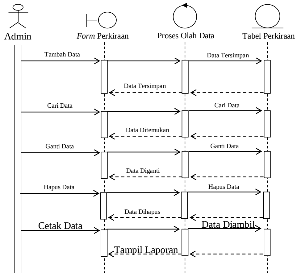
Gambar III.23. Sequence Diagram Perkiraan Bagian Admin
