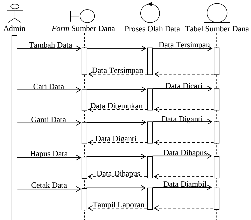
Gambar III.21. Sequence Diagram Sumber Dana Bagian Admin
