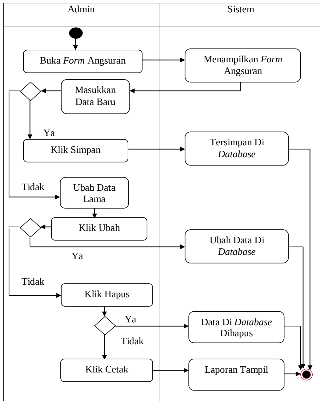
Gambar III.10. Activity Diagram Angsuran Bagian Admin
