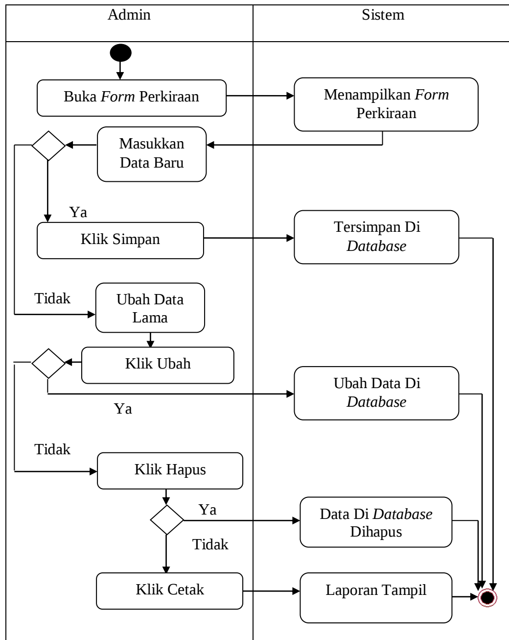
Gambar III.14. Activity Diagram Perkiraan Bagian Admin
