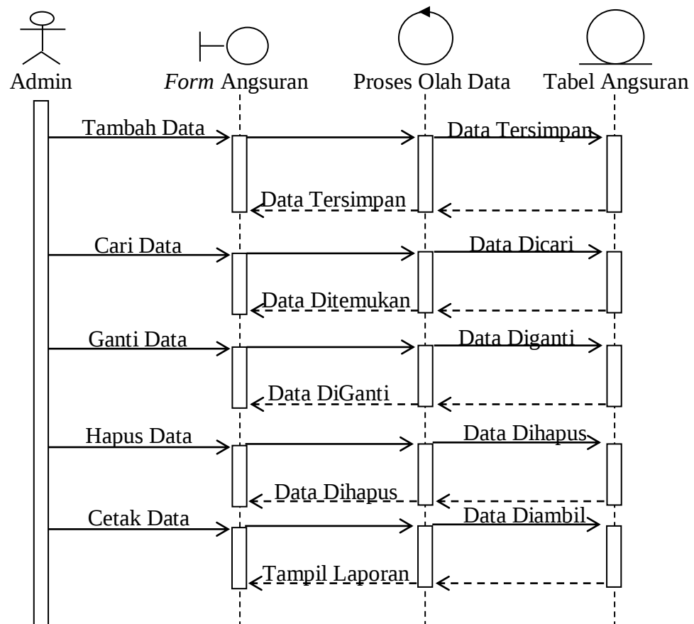
Gambar III.19. Sequence Diagram Angsuran Bagian Admin
