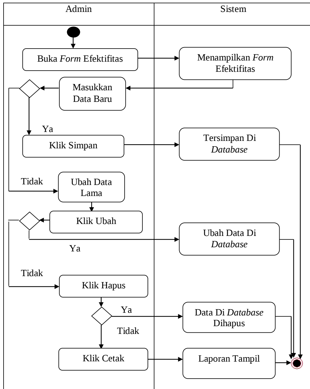
Gambar III.11. Activity Diagram Efektifitas Bagian Admin
