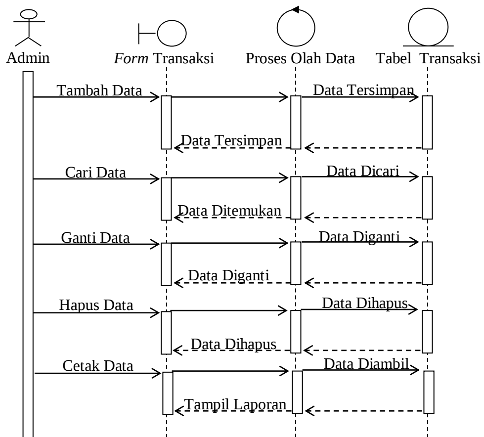
Gambar III.22. Sequence Diagram Transaksi Bagian Admin
