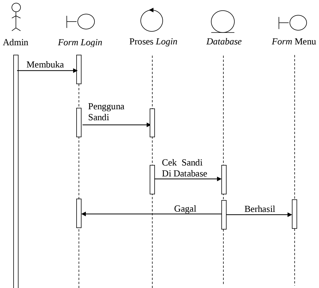
Gambar III.18. Sequence Diagram Login Bagian Admin
