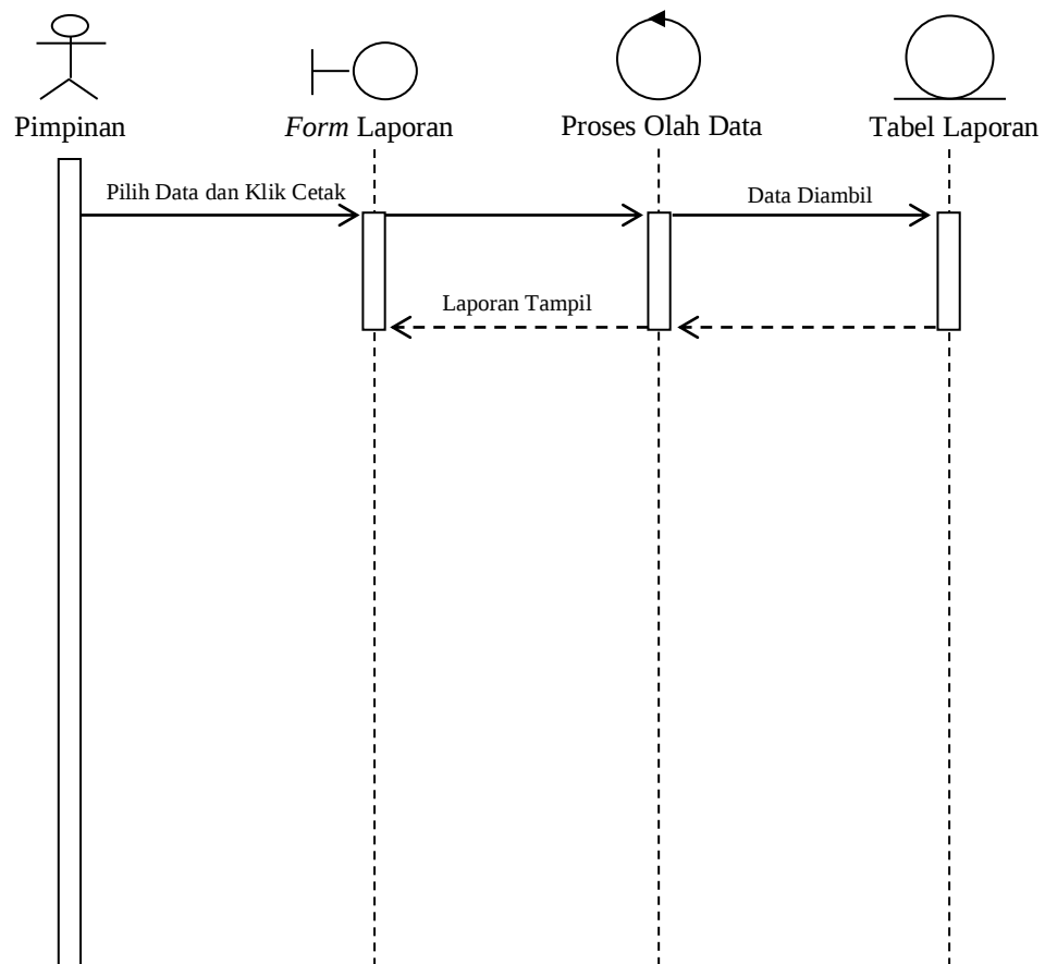
Gambar III.26. Sequence Diagram Laporan Bagian Pimpinan
