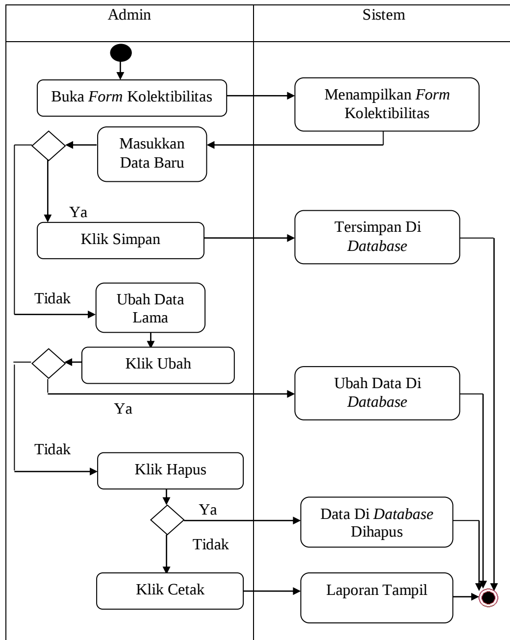
Gambar III.16. Activity Diagram Kolektibilitas Bagian Admin
