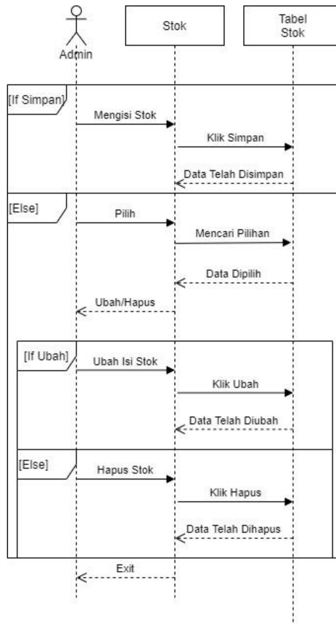
Gambar III.16. Sequence Diagram Data Stok Bagian Admin
