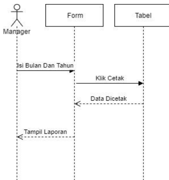
Gambar III.20. Sequence Diagram Laporan Bagian Manager
