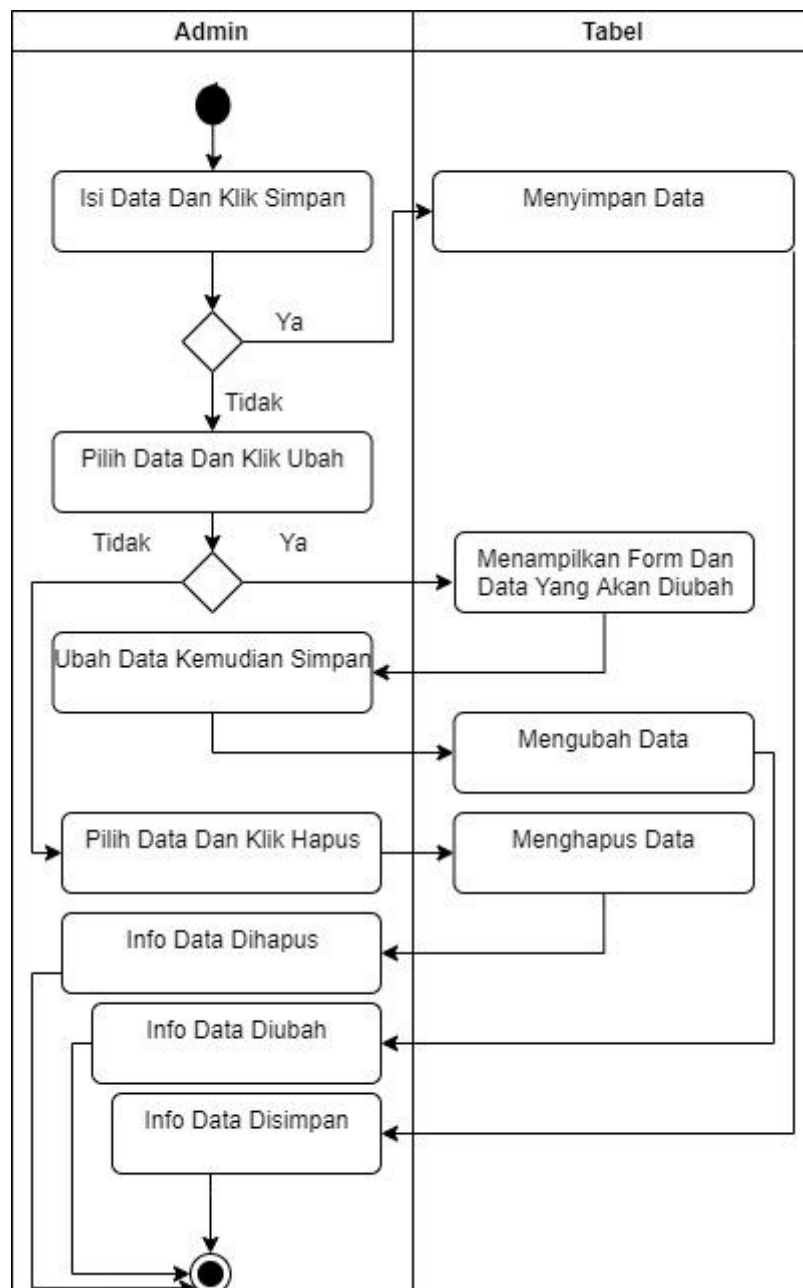
Gambar III.9. Activity Diagram Stok Bagian Admin
