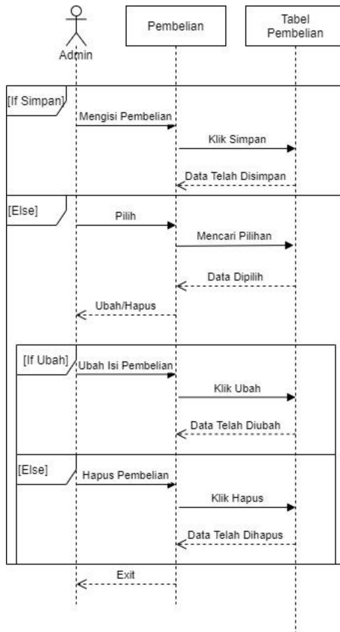
Gambar III.17. Sequence Diagram Pembelian Bagian Admin
