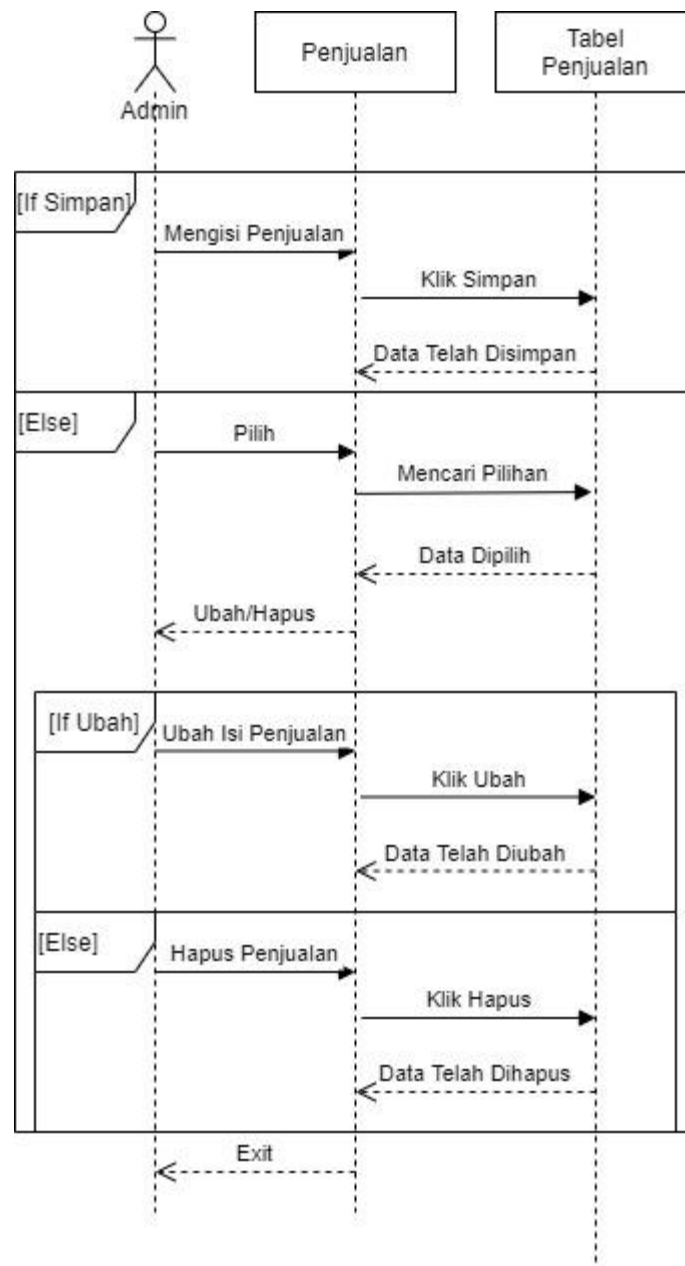
Gambar III.18. Sequence Diagram Penjualan Bagian Admin
