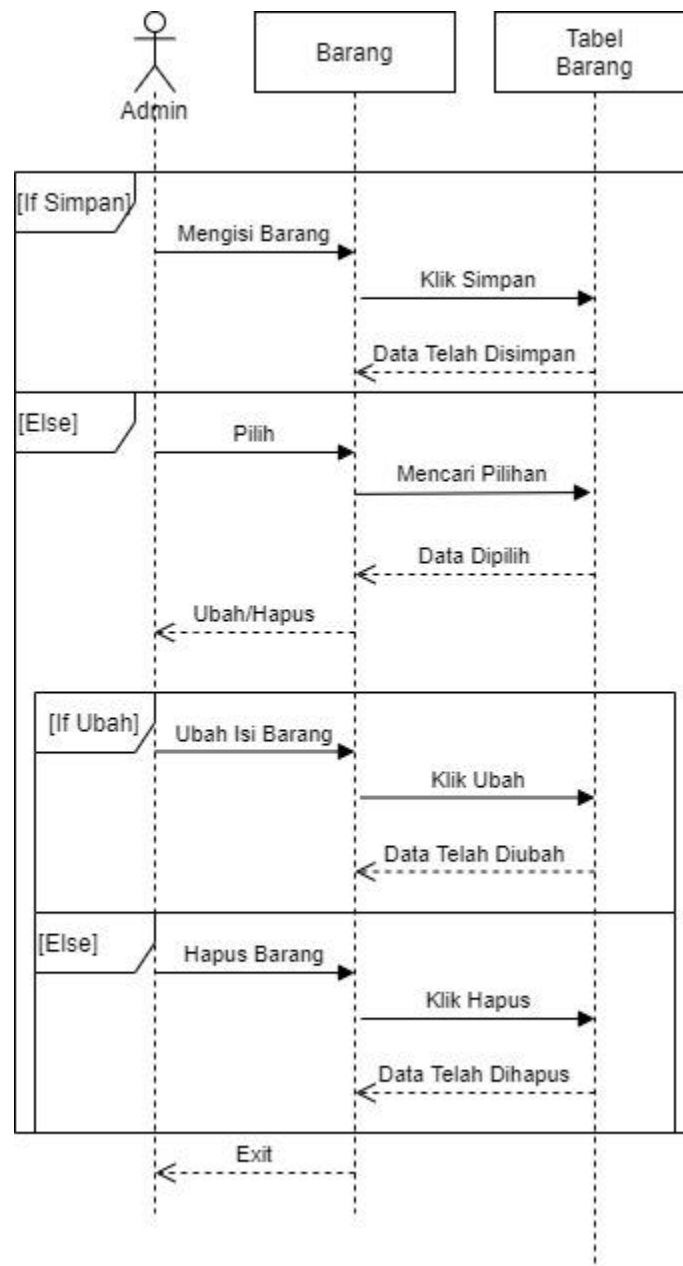
Gambar III.16. Sequence Diagram Data Barang Bagian Admin
