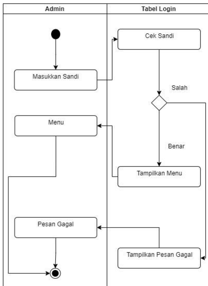
Gambar III.8. Activity Diagram LoginBagian Admin
