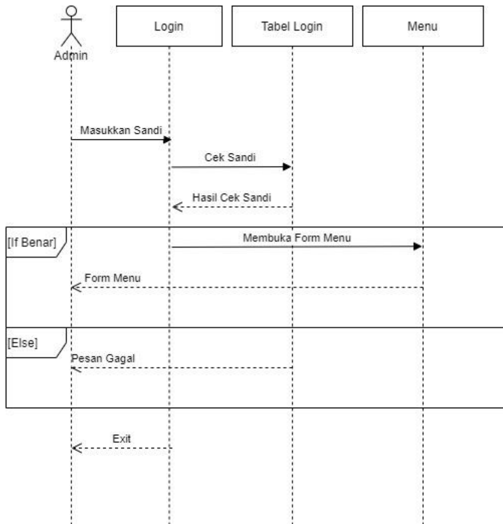
Gambar III.15. Sequence Diagram Login Bagian Admin
