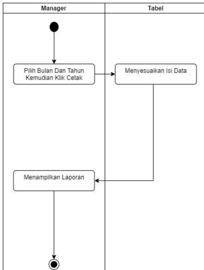
Gambar III.13. Activity Diagram Laporan Bagian Manager
