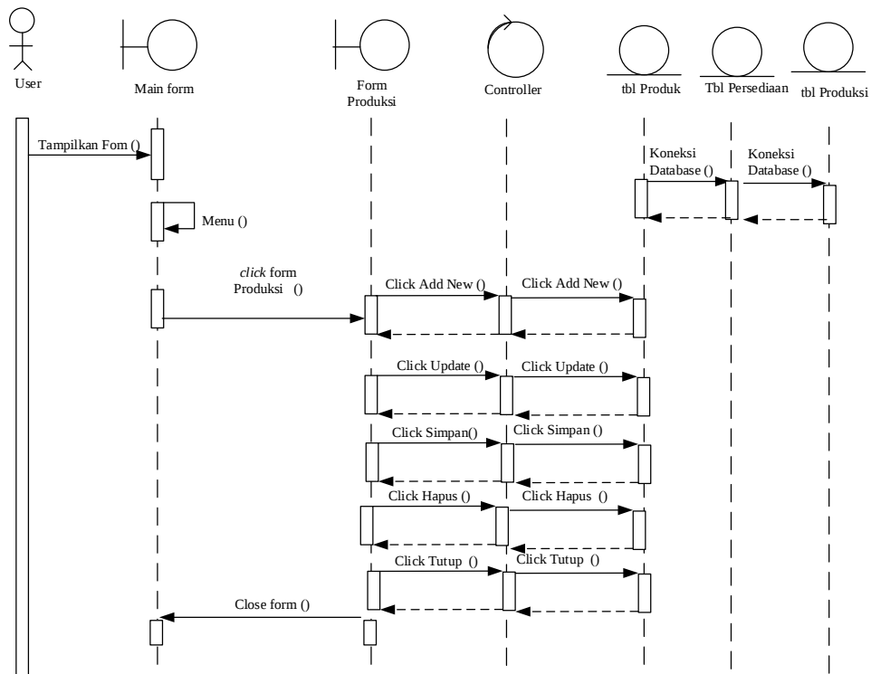
Gambar III.16. Sequence Diagram Form Produksi
