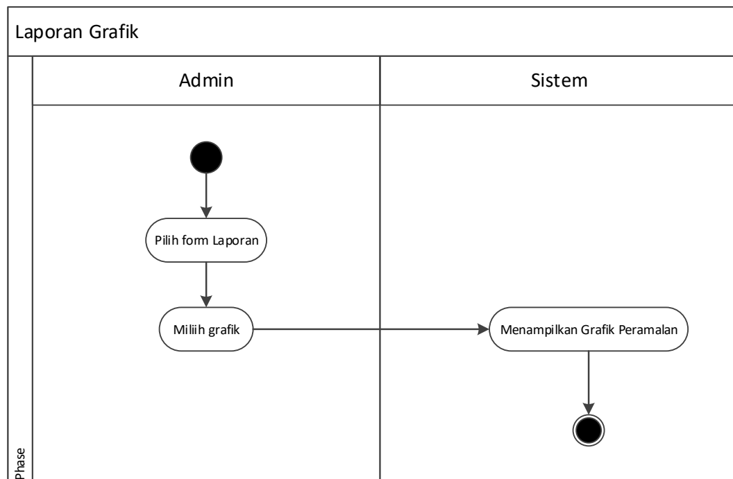
Gambar III.9. Activity Diagram Form Laporan Grafik
