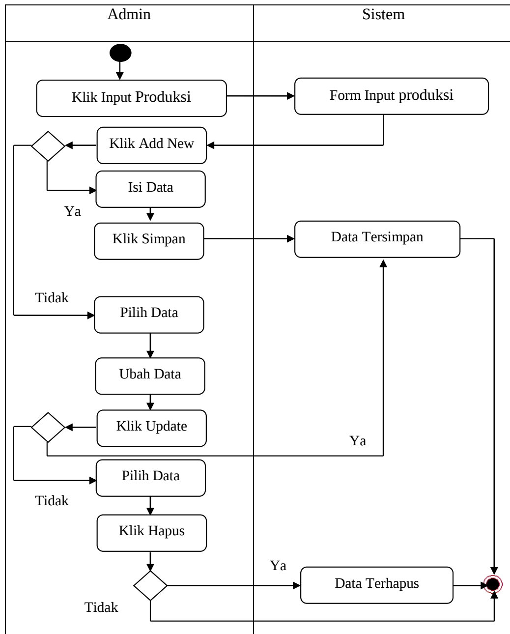
Gambar III.5. Activity Diagram Form Produksi
