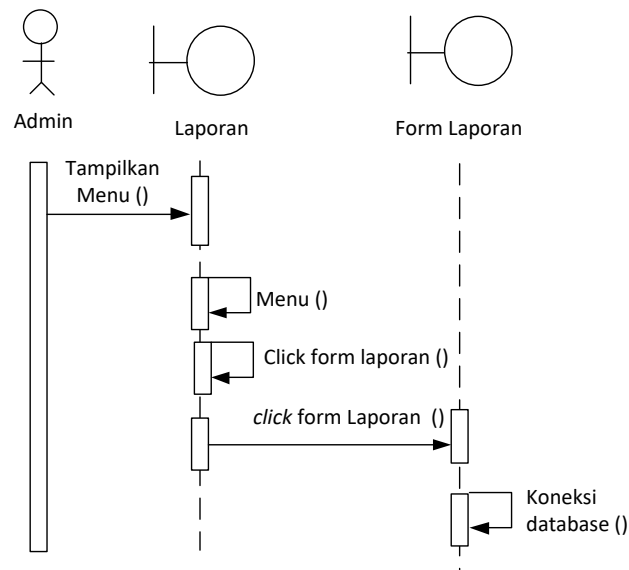
Gambar III.19. Sequence Diagram Form Laporan Produksi
