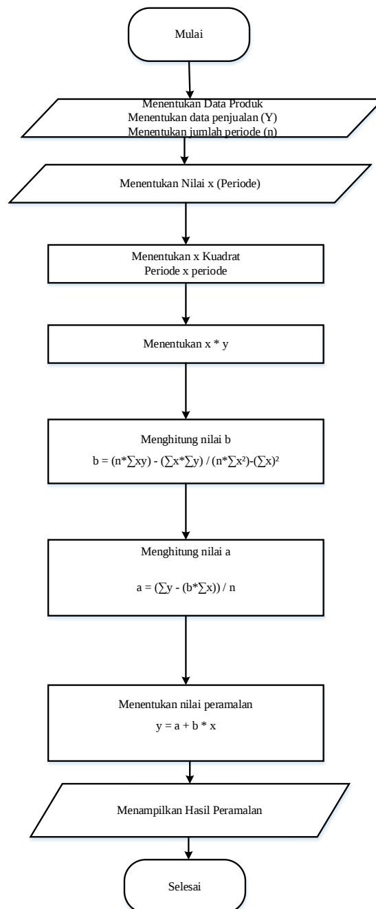
Gambar III.1. Flowchart Metode Trend projection
