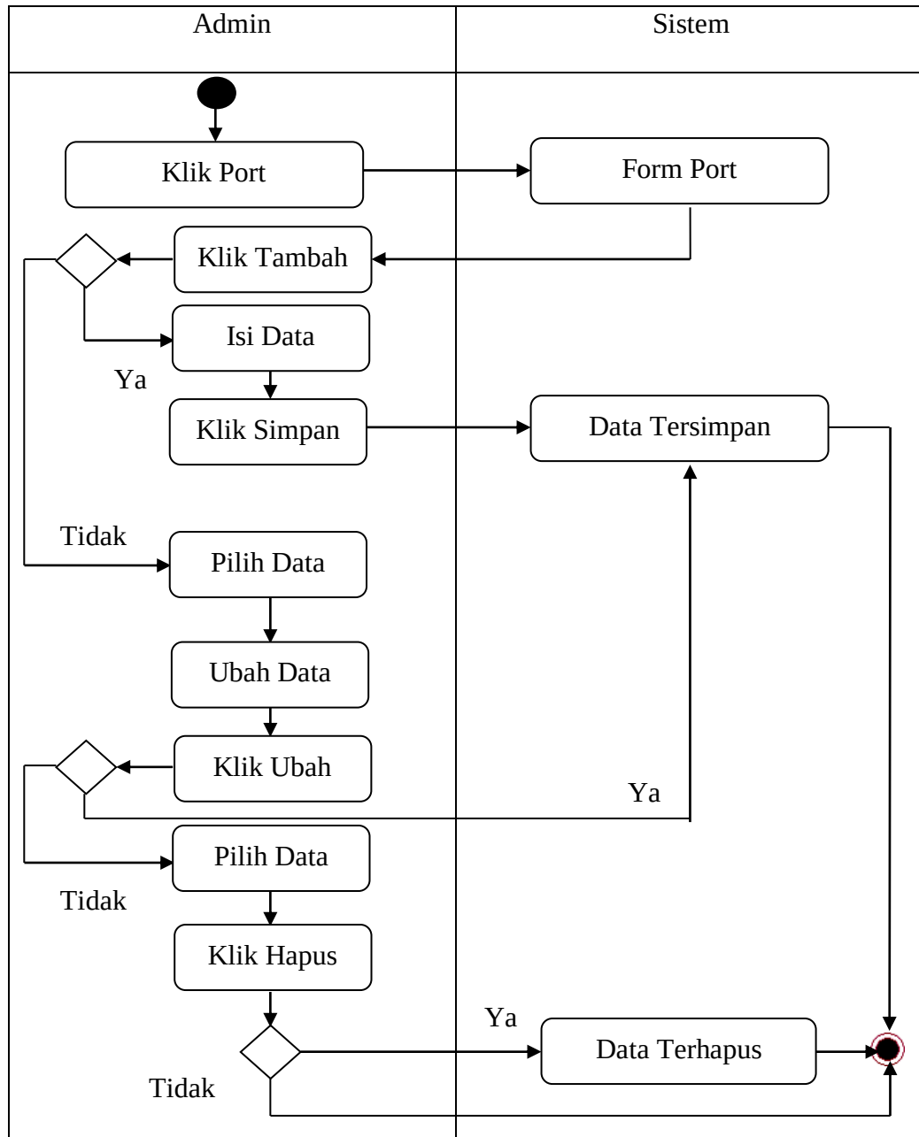
Gambar III.10. Activity Diagram Form Port
