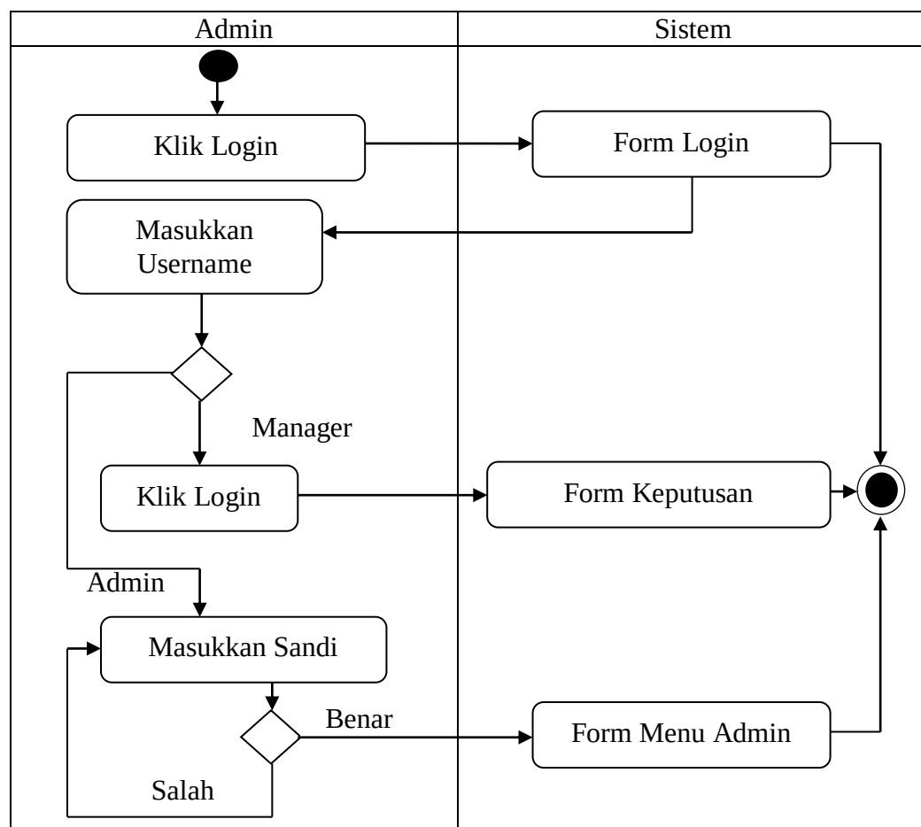
Gambar III.7. Activity Diagram Login
