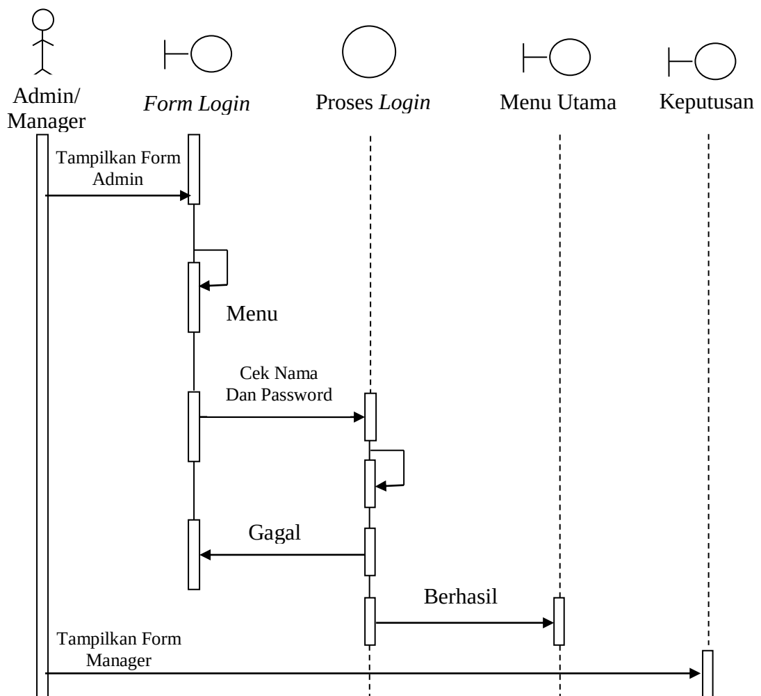
Gambar III.15. Sequence Diagram Login
