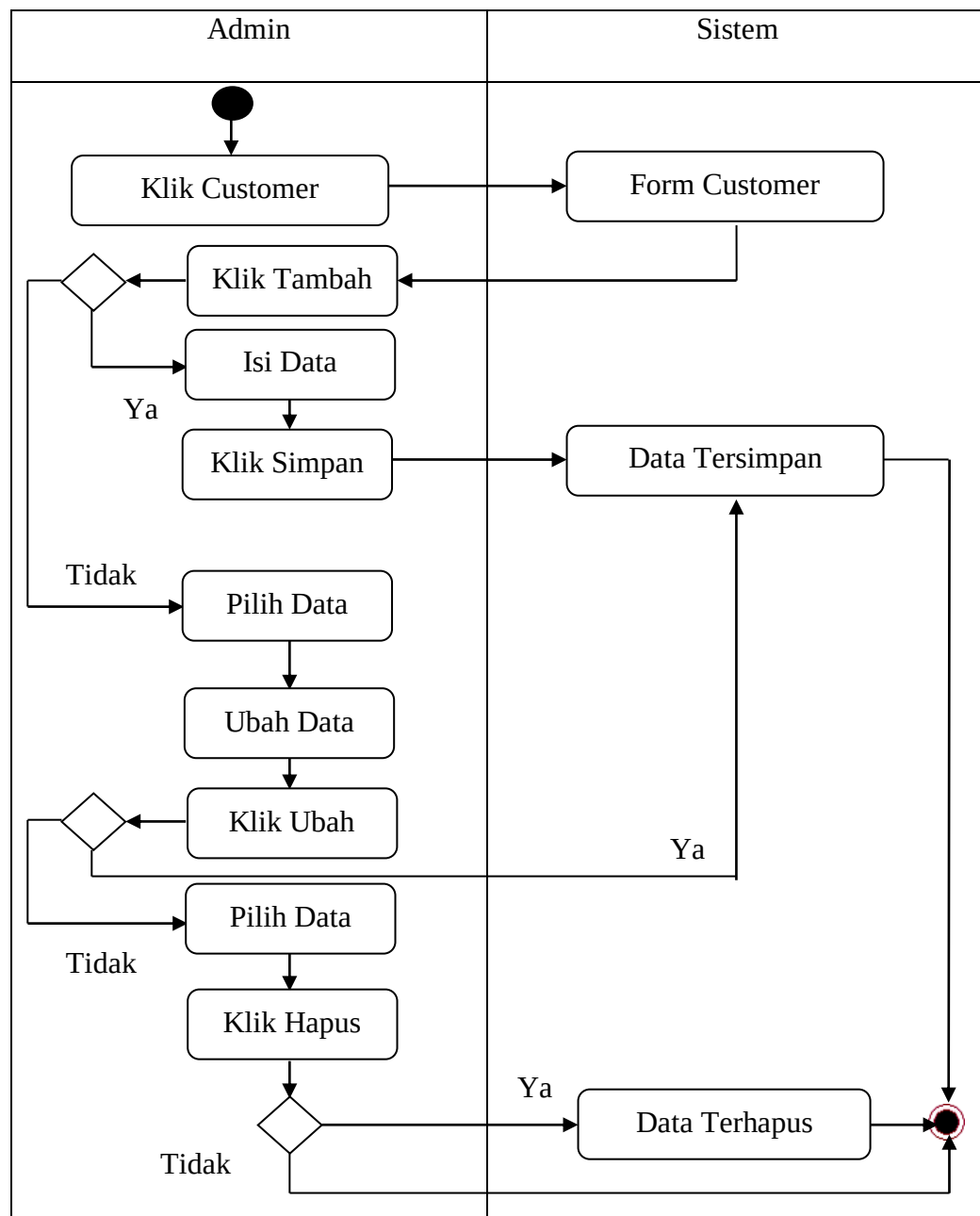
Gambar III.11. Activity Diagram Form Customer
