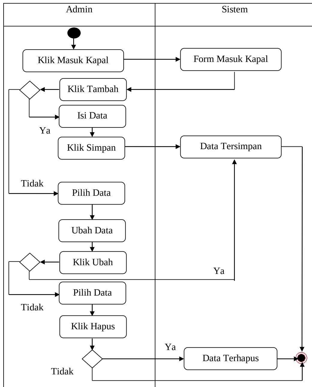
Gambar III.13. Activity Diagram Form Masuk Kapal
