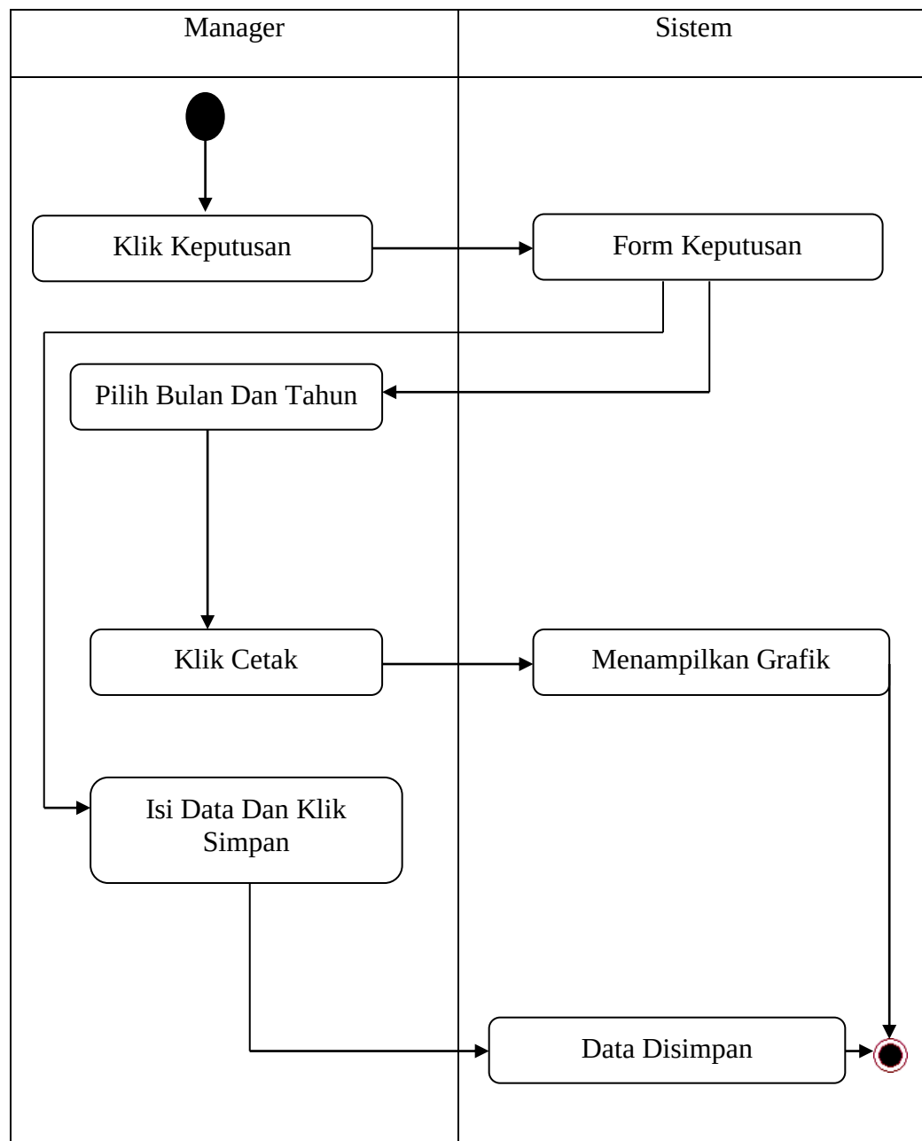
Gambar III.14. Activity Diagram Form Manager
