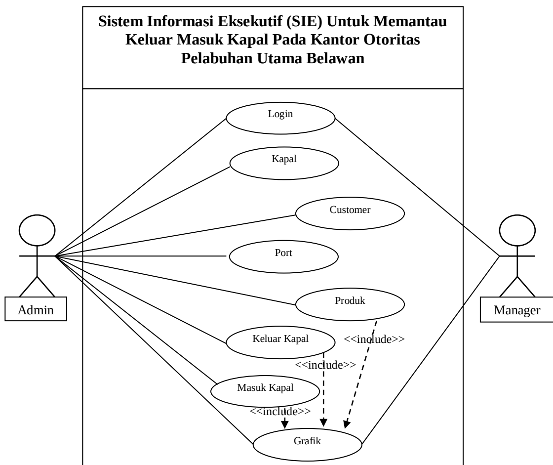
Gambar III.5. Use Case Diagram
