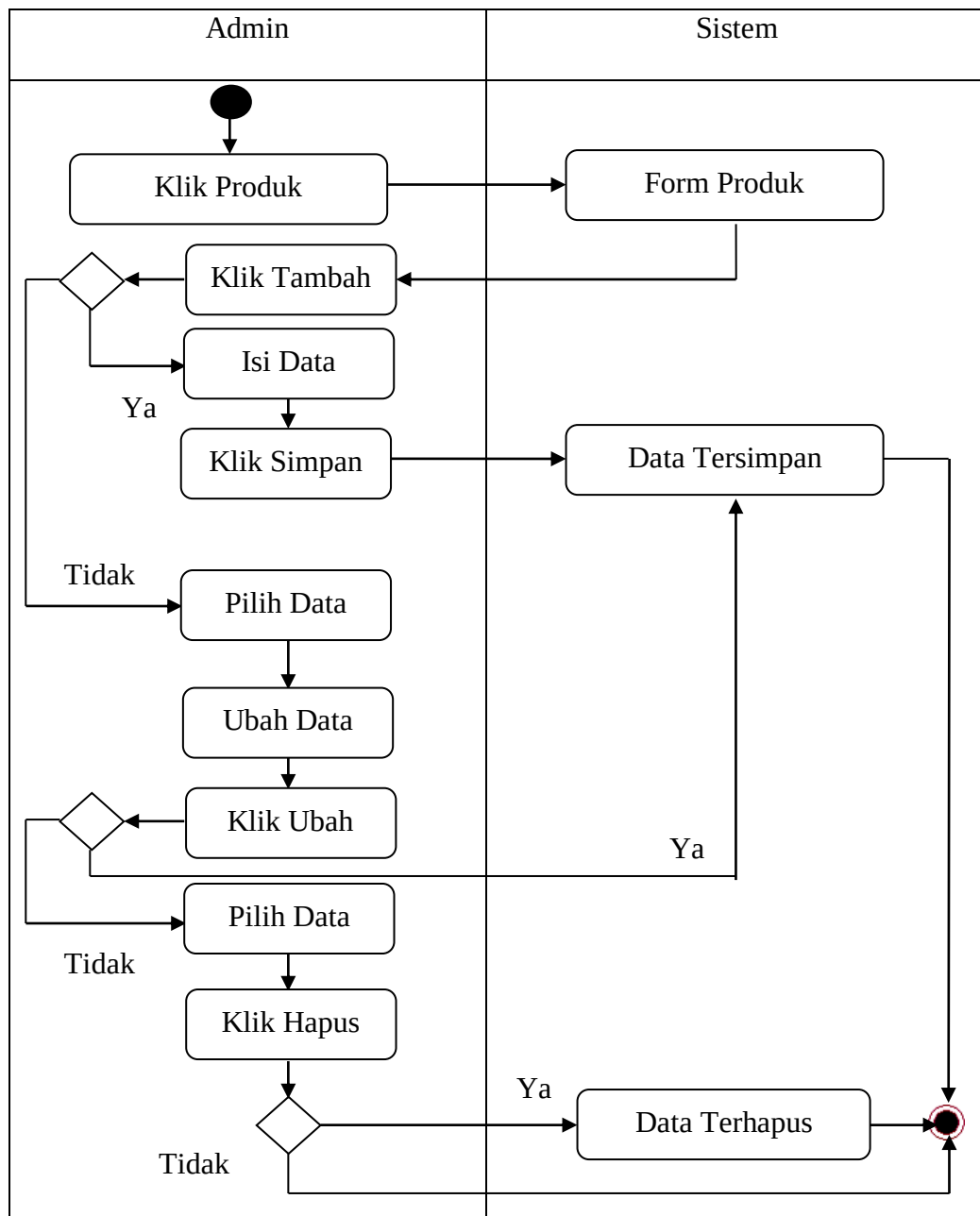
Gambar III.9. Activity Diagram Form Produk
