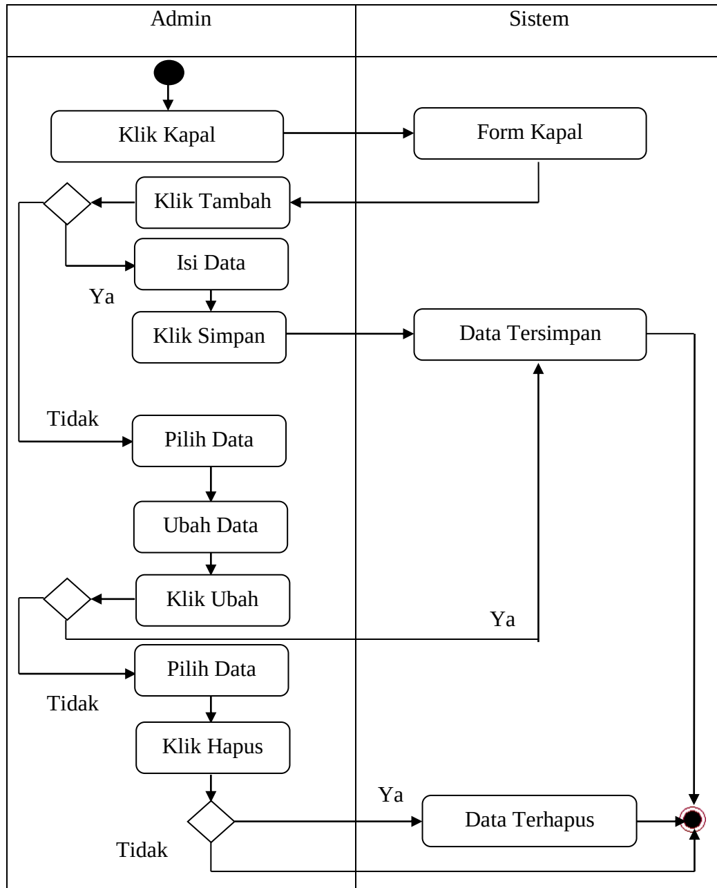
Gambar III.8. Activity Diagram Form Kapal
