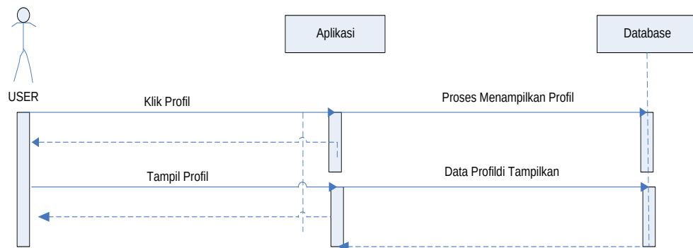
Gambar III.10 Sequence Diagram Halaman Profil
