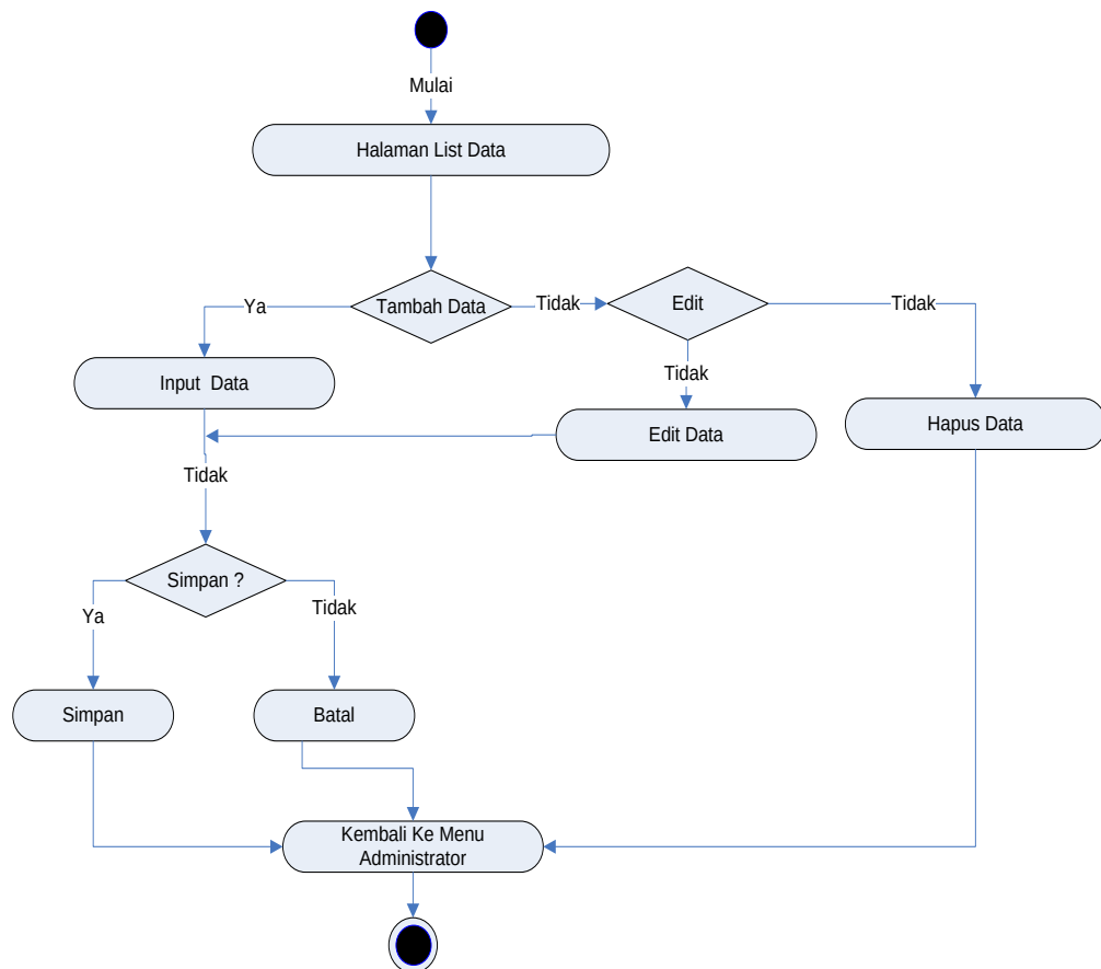
Gambar III.24. Diagram Activity Halaman Input Data
