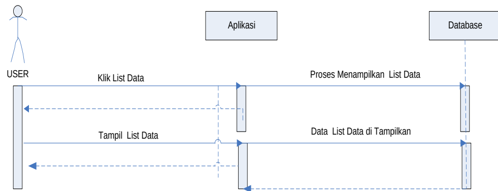
Gambar III.10 Sequence Diagram Halaman List Data
