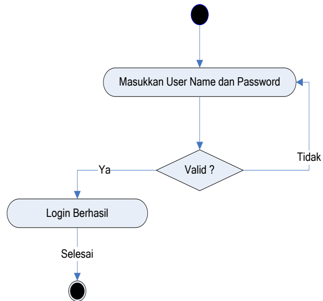
Gambar III.20. Diagram Activity Login Administrator
