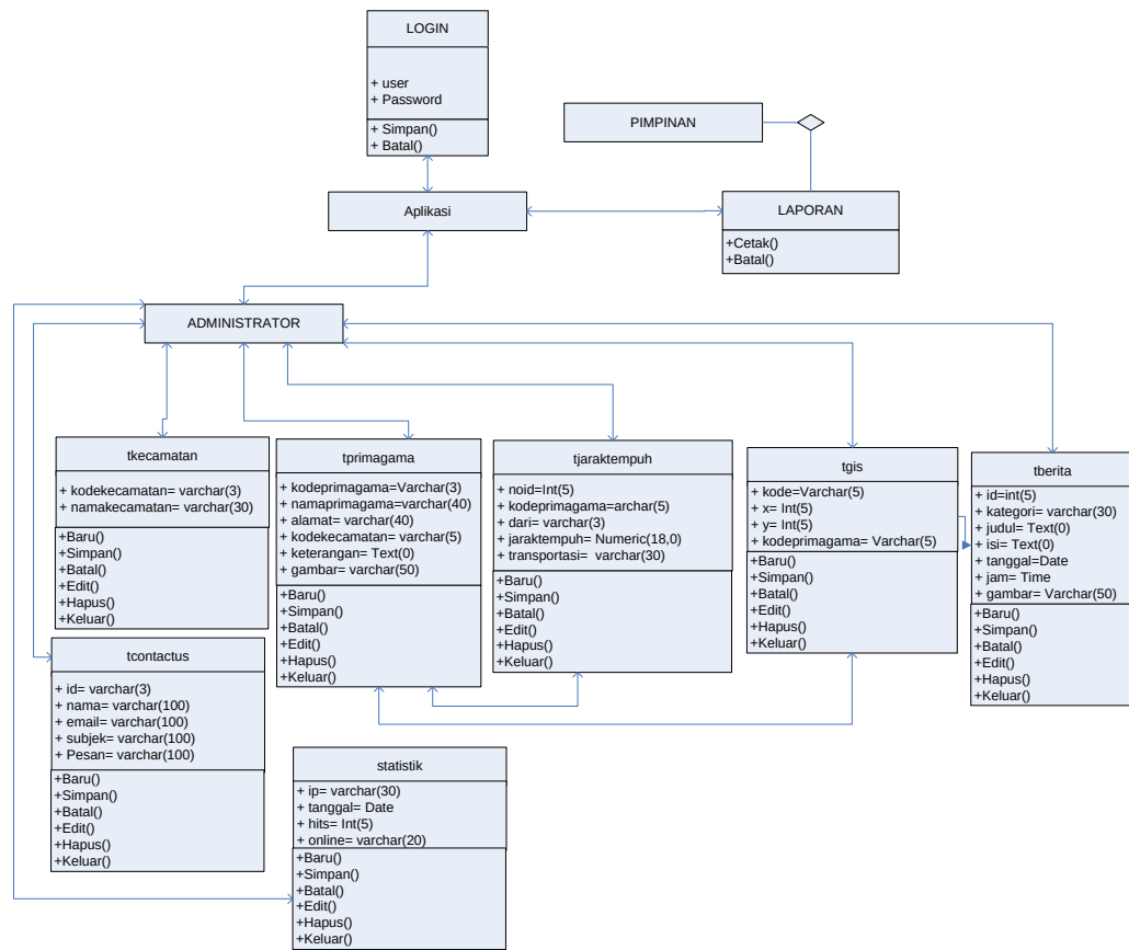
Gambar III.3 Class diagram Admin
