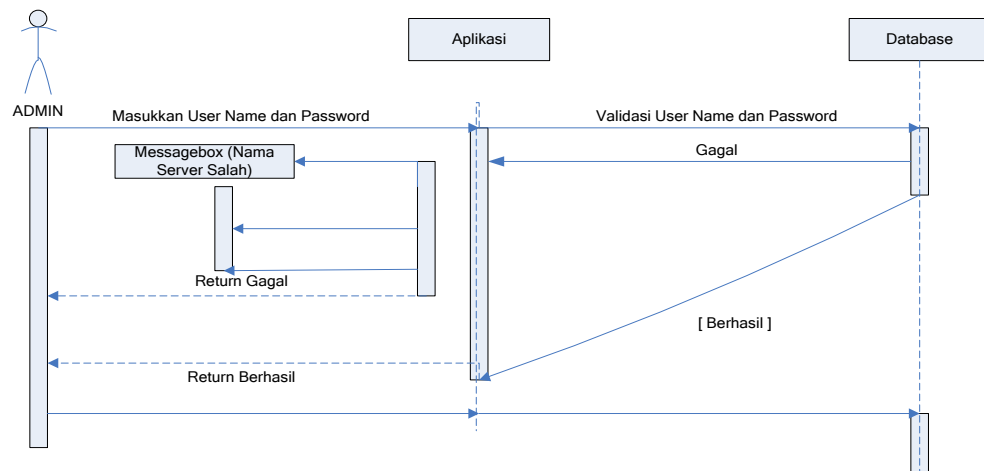
Gambar III.4 Sequence Diagram Login Admin
