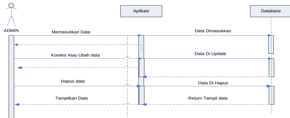
Gambar III.5 Sequence Diagram Input Data
