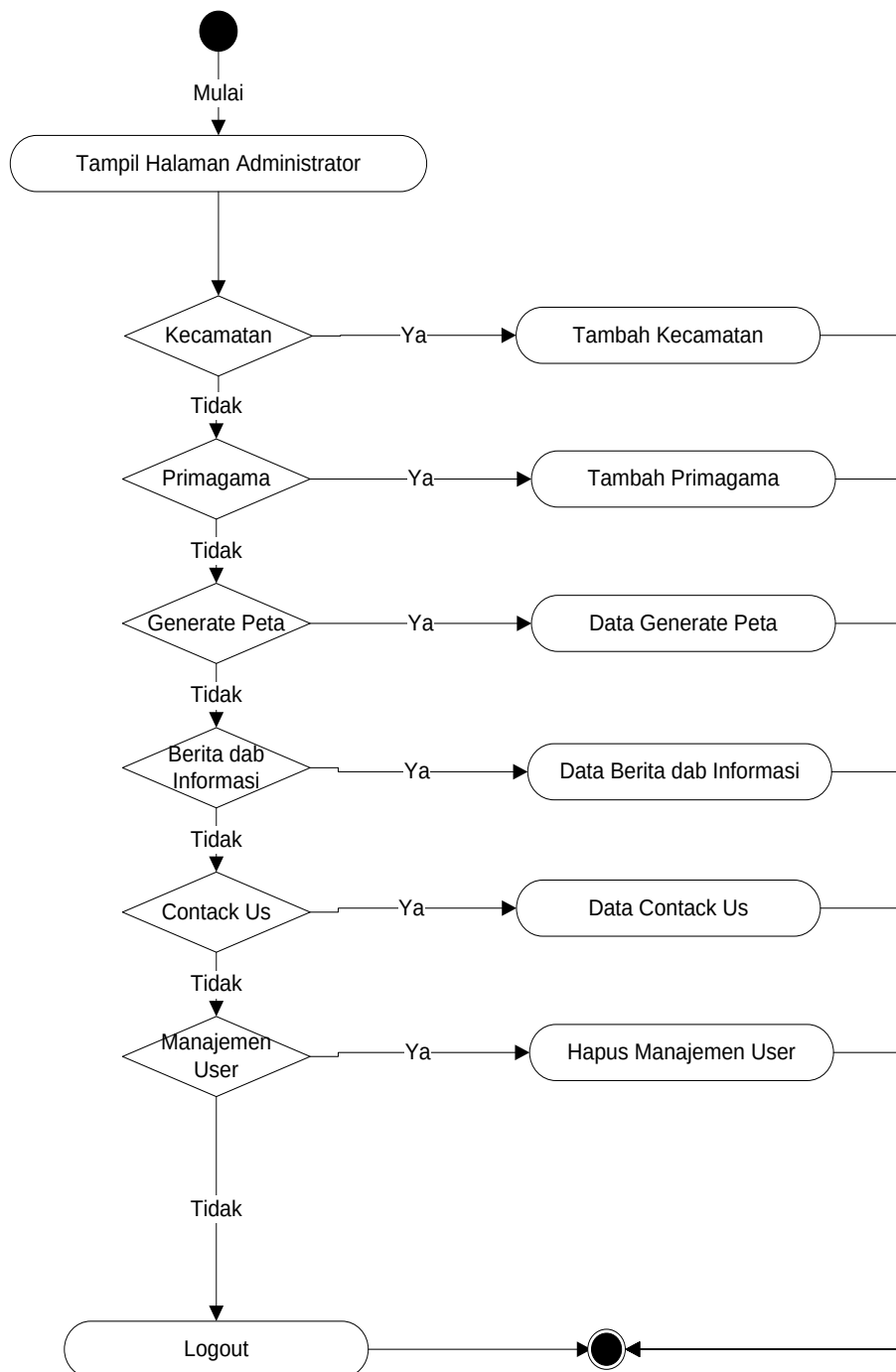
Gambar III.21. Diagram Activity Menu Administrator
