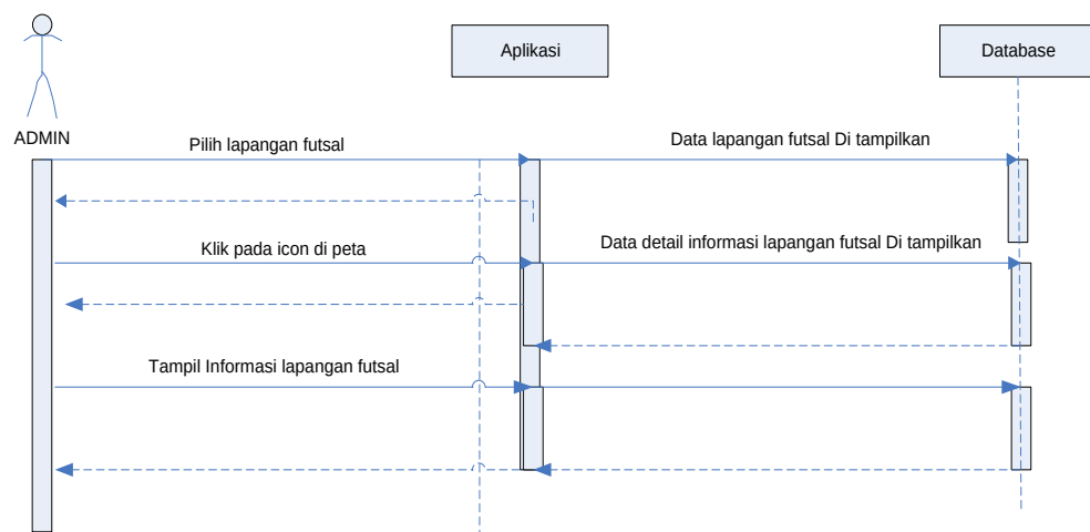
Gambar III.10 Sequence Diagram Halaman List Data
