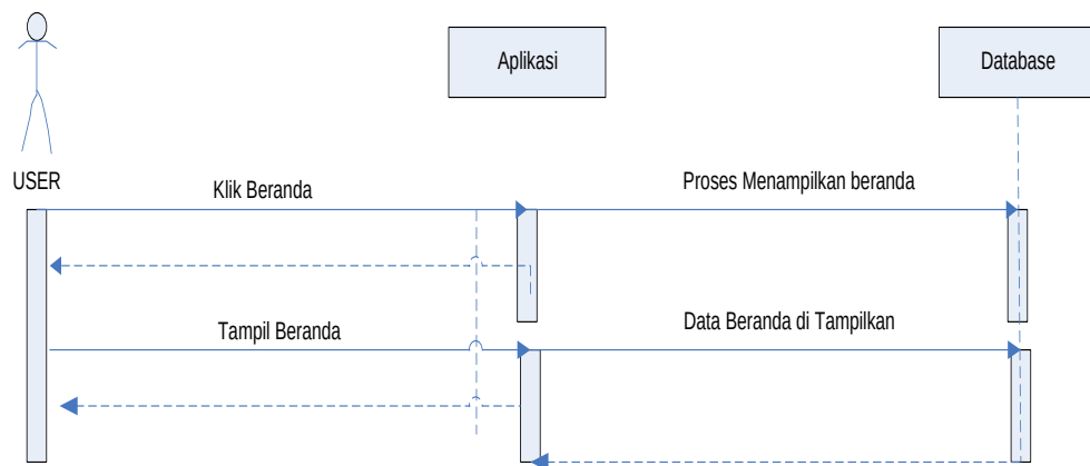
Gambar III.10 Sequence Diagram Halaman Beranda
