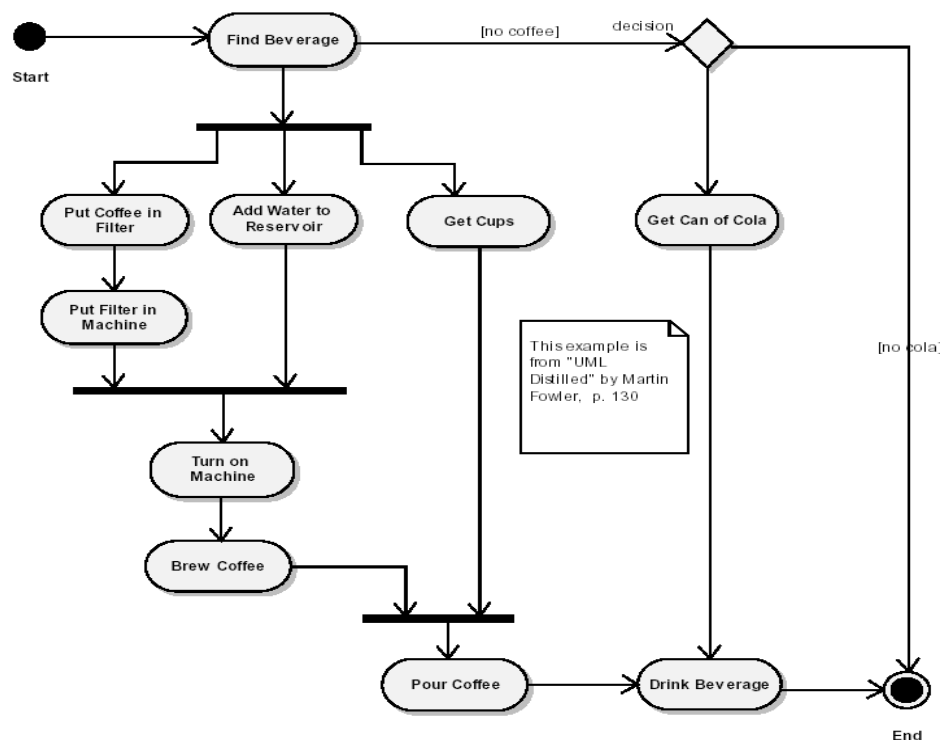
Gambar. II.1 : Activity Diagram Tanpa Swimlalan
