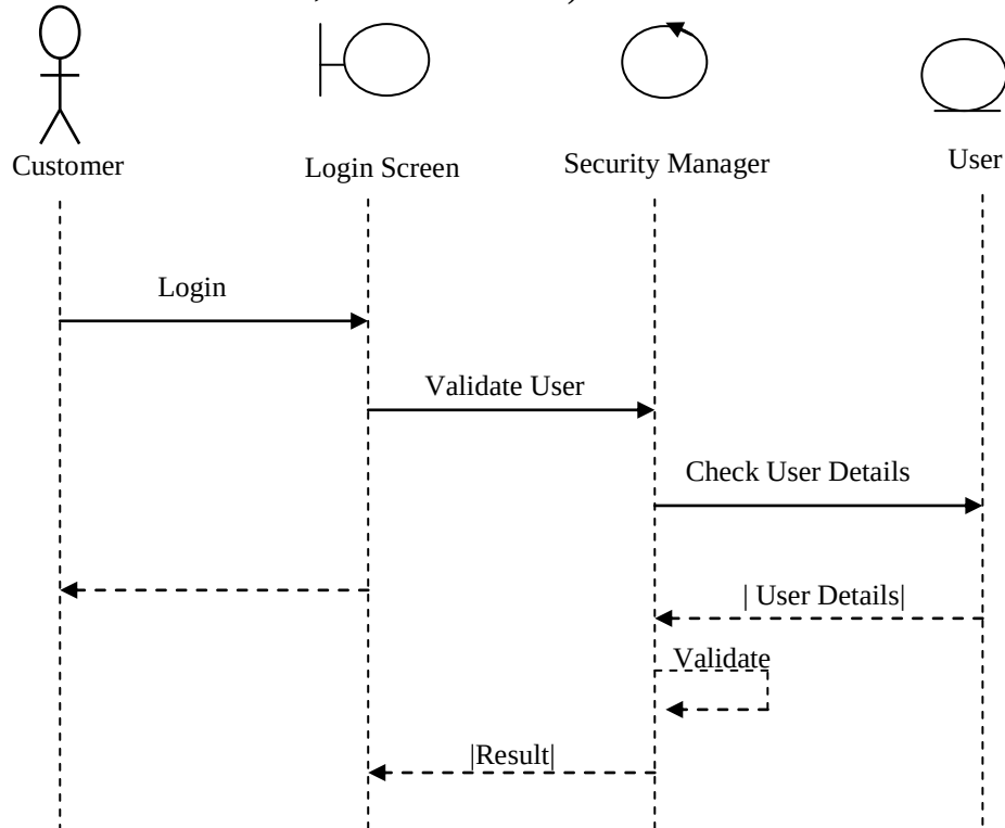
Gambar II.11. Diagram Urutan
