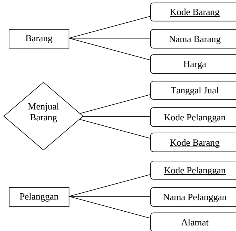
Gambar II.18 Relationship
