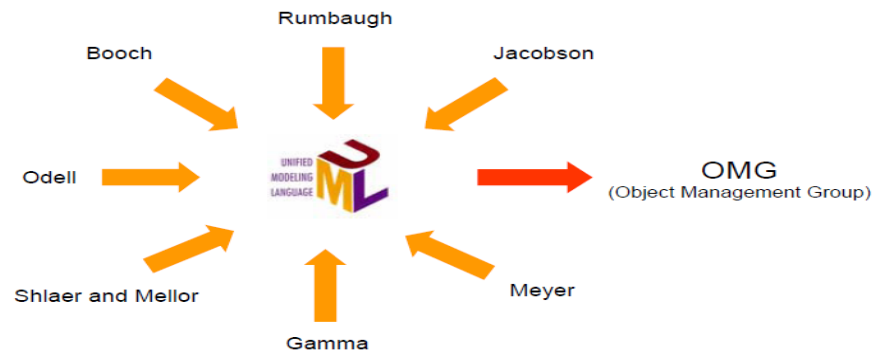
Gambar II.8 : Metodologi UML
