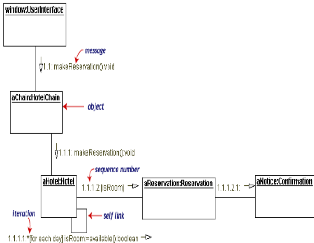
Gambar II.14. Contoh Collaboration Diagram
