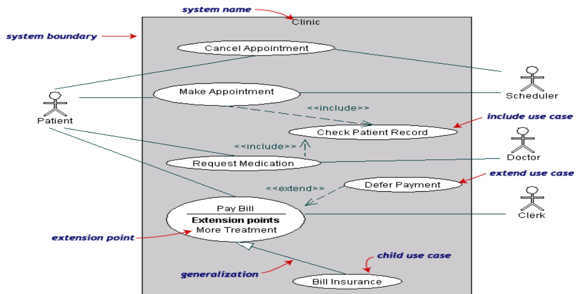
Gambar II.9. : Contoh Diagram Use case
