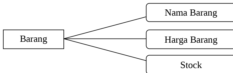
Gambar II.17 Atribut
