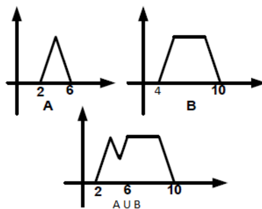
Gambar II.6 Operasi Union
