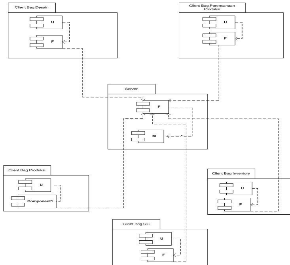
Gambar II.15. Contoh Component Diagram
