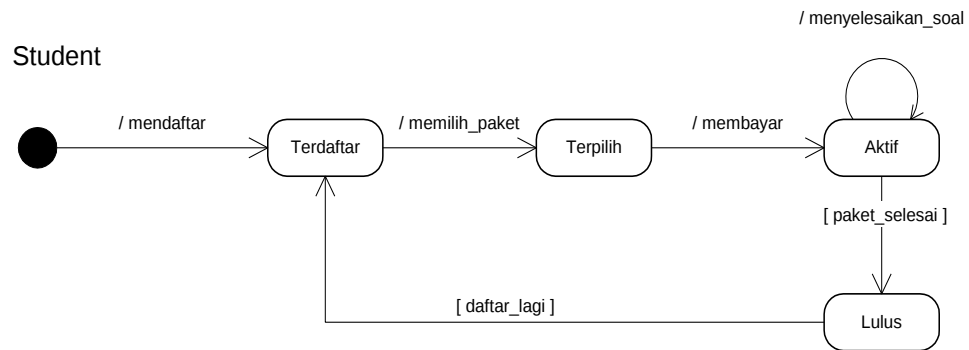
Gambar II.11. Contoh Statechart Diagram
