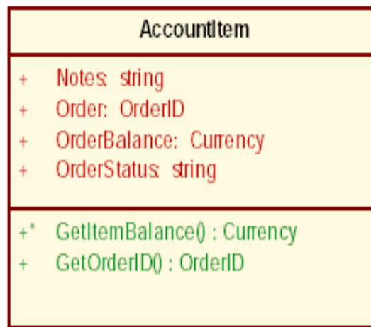
Gambar II.10. Class Diagram
