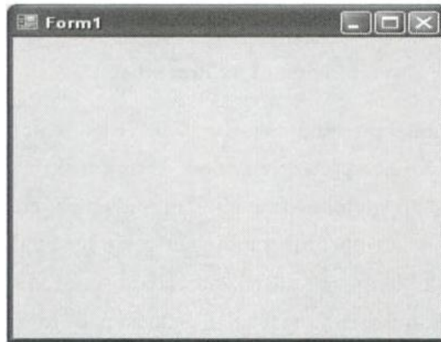
Gambar II.20 Form
