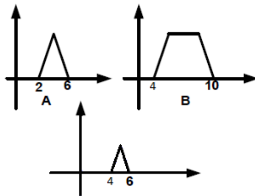
Gambar II.7 operasi Intersection
