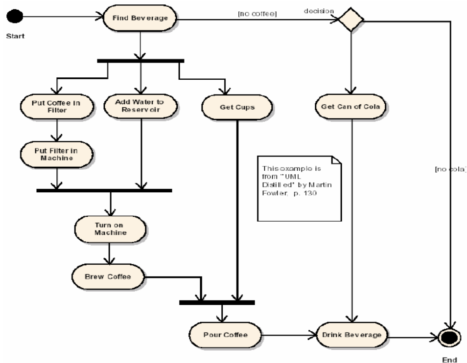
Gambar II.12. Contoh Activity Diagram - Tanpa Swimlane
