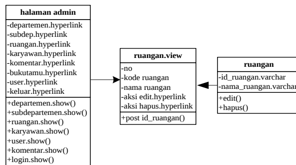
Gambar III.16. Class Diagram Data Ruangan
