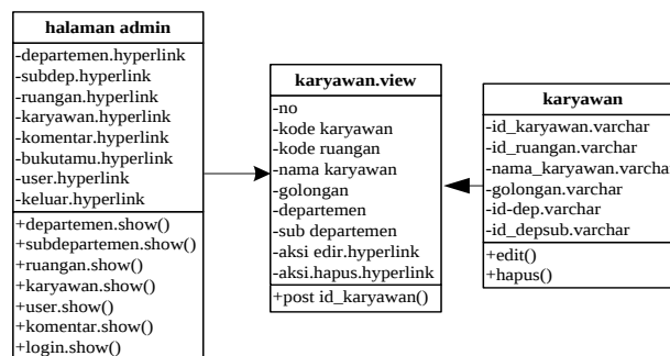
Gambar III.17. Class Diagram Data Karyawan
