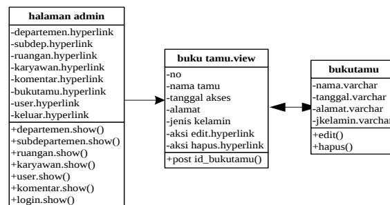
Gambar III.19. Class Diagram Data Buku Tamu
