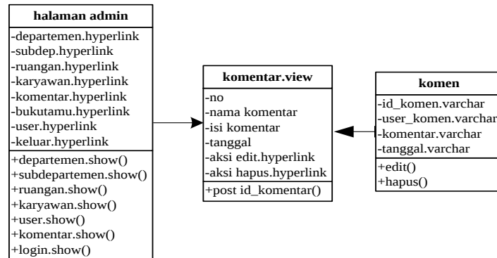
Gambar III.18. Class Diagram Data Komentar
