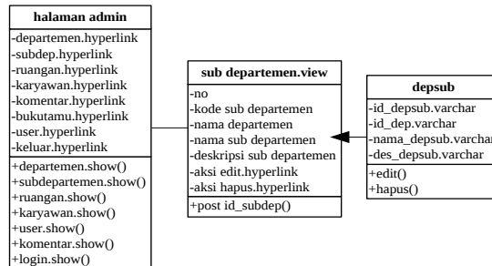
Gambar III.15. Class Diagram Data Sub Departemen
