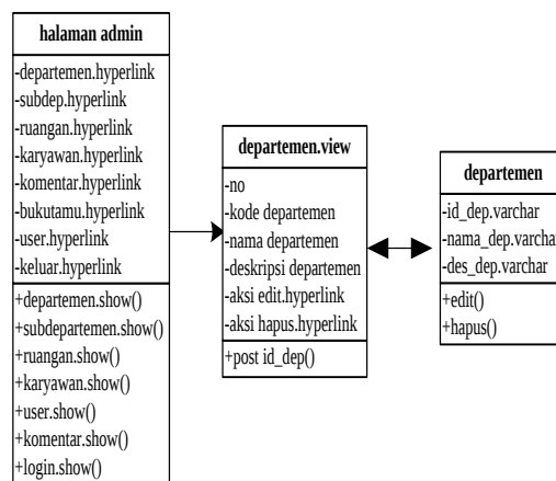
Gambar III.14. Class Diagram Data Departemen
