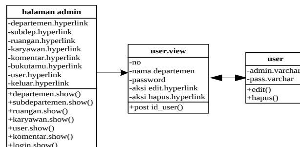
Gambar III.20. Class Diagram Data User
