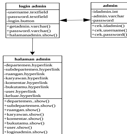
Gambar III.13. Class Diagram Login Admin
