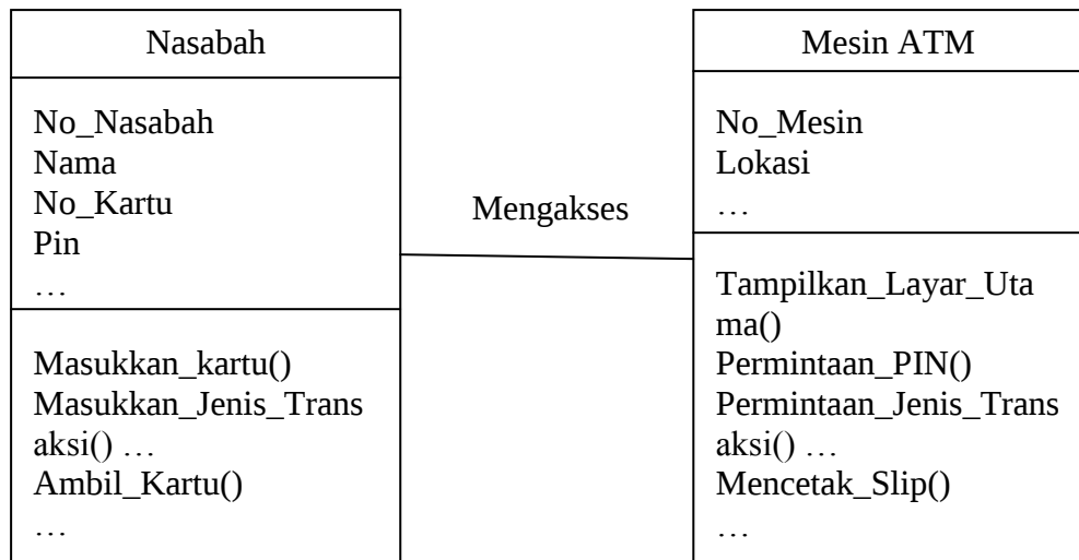
Gambar II.4. Class diagram
