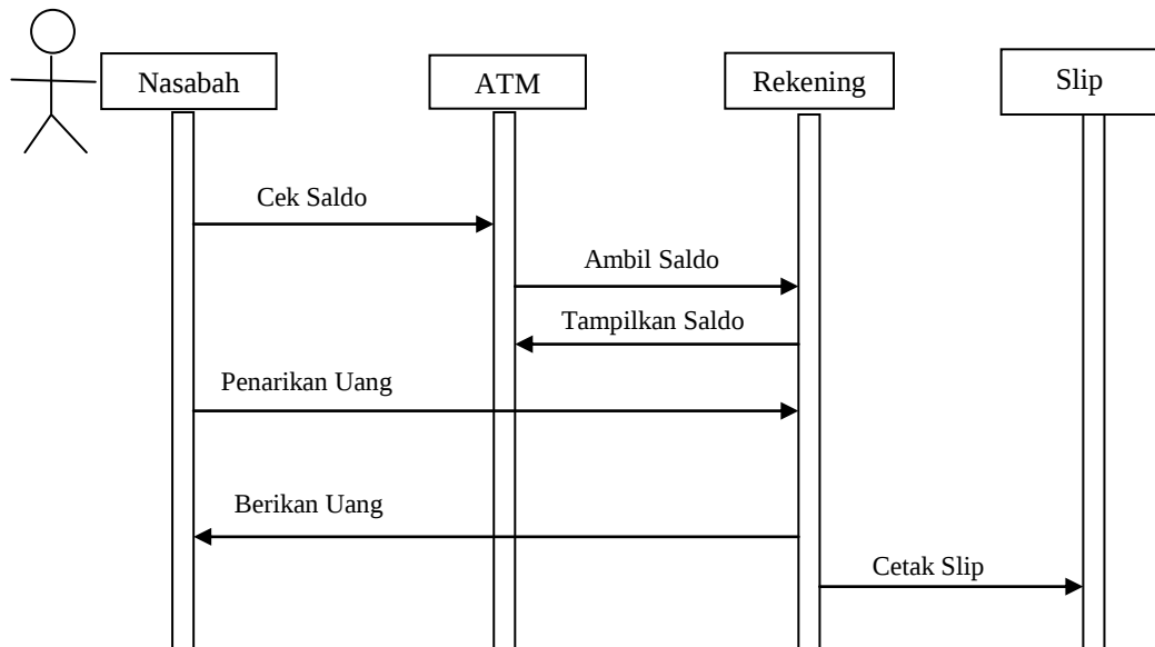
Gambar II.6 Squence Login
