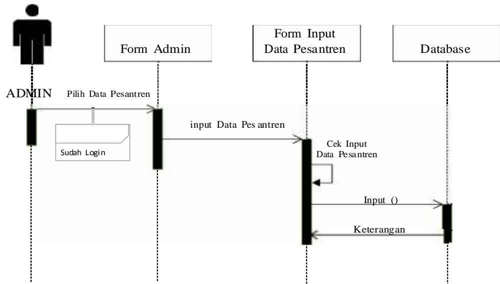
Gambar III.11. Sequence Diagram Input Data Pesantren
