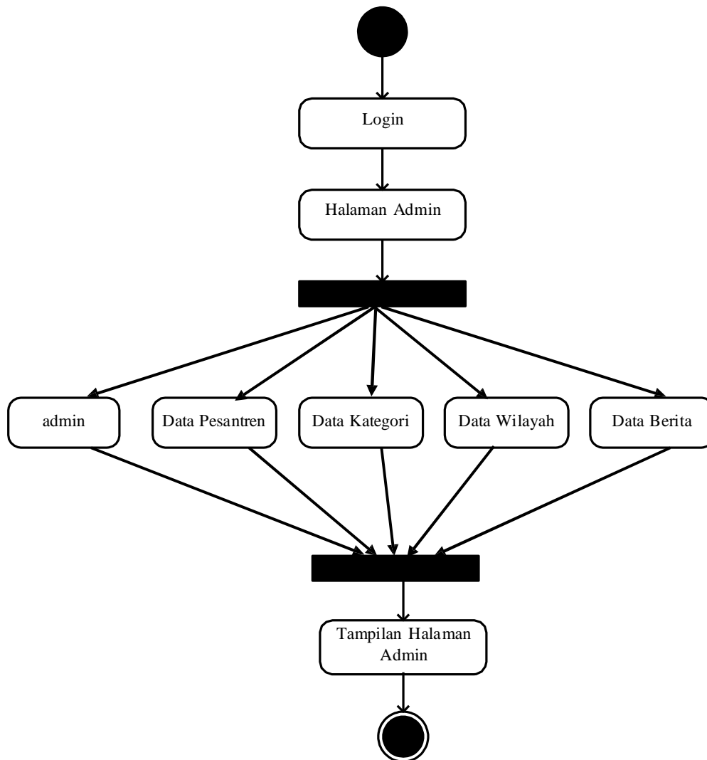
Gambar III.4. Activity Diagram Halaman Admin Sistem Informasi
