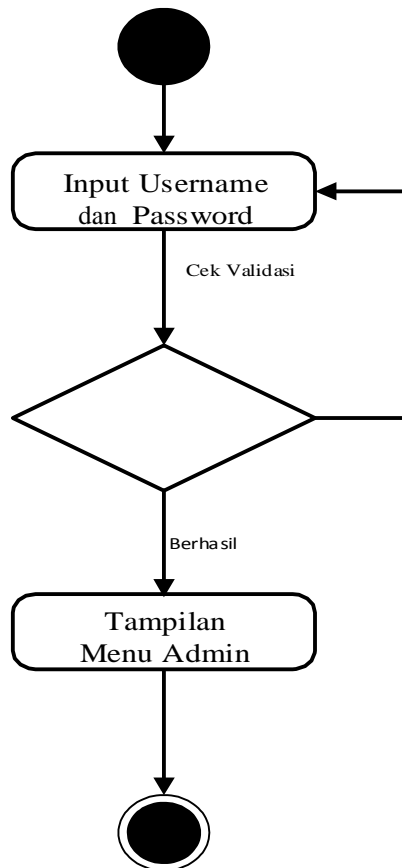
Gambar III.3. Activity Diagram Login Admin Sistem Informasi
