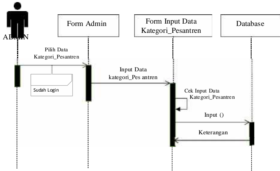
Gambar III.12. Sequence Diagram Input Data Pesantren_Kategori
