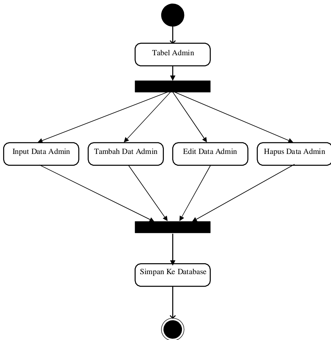
Gambar III.5. Activity Diagram Tabel Admin Sistem Informasi
